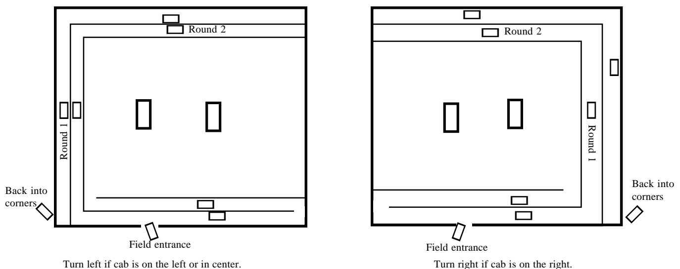
Figure 1. How to start spraying a field — spraying three sides.
