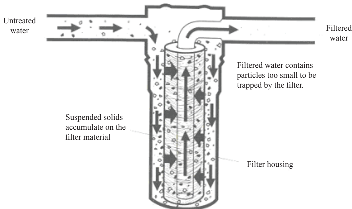
Figure 1. The sediment filtration process. From Wagenet, L. K. Mancl, and M. Sailus, 1995. "Home Water Treatment," Northeast Regional Agricultural Engineering Service, Cooperative Extension, Ithaca, N.Y.
