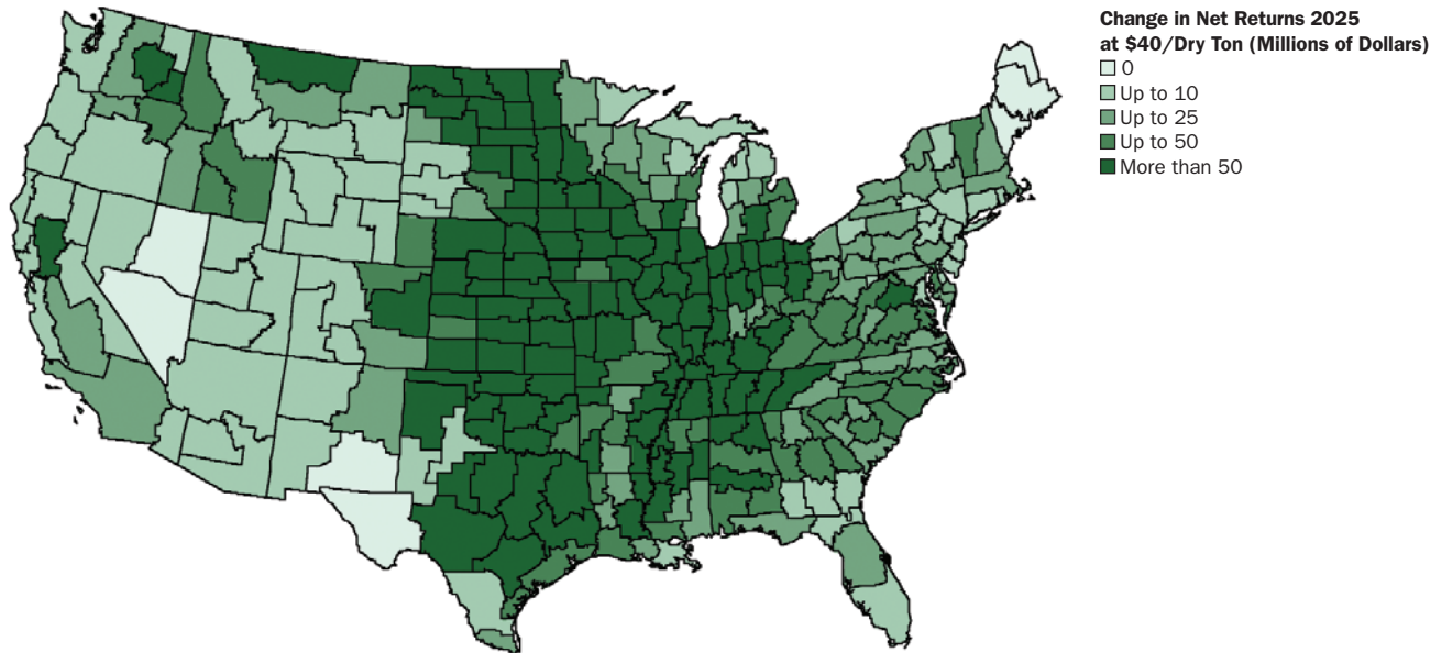
FIGURE 1 2025 Change in Farmers' Total Net Returns Relative to USDA Baseline Due to Switchgrass Market
