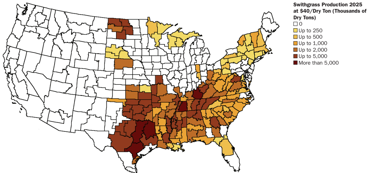
FIGURE 3 Map of Switchgrass Production in 2025 Assuming Constant Price of $40 Per Dry Ton
