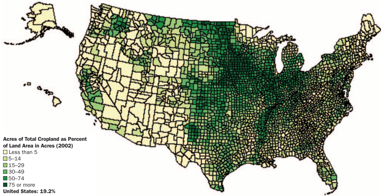
FIGURE 5 Percent of Land Covered by Cropland
