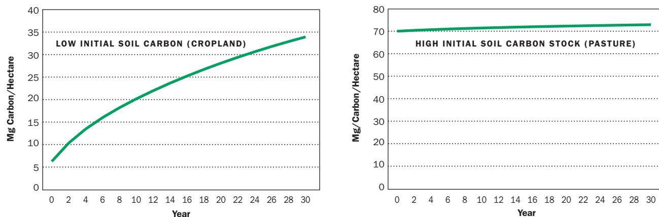
FIGURE 4 Switchgrass Improves Soil Carbon 30
