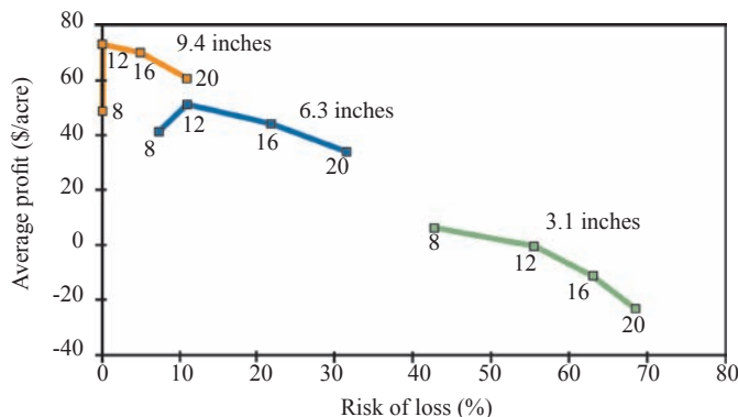
Figure 4. Average profit vs. risk of loss at Sidney, Nebraska with soil water at planting at 3.1, 6.3 and 9.4 inches and 8,000, 12,000, 16,000 and 20,000 established plants. (P = $2.13/bu; FC = $62.19/acre; N = $0.24/lb; S = $100/bag; H = $0.15/bu)
