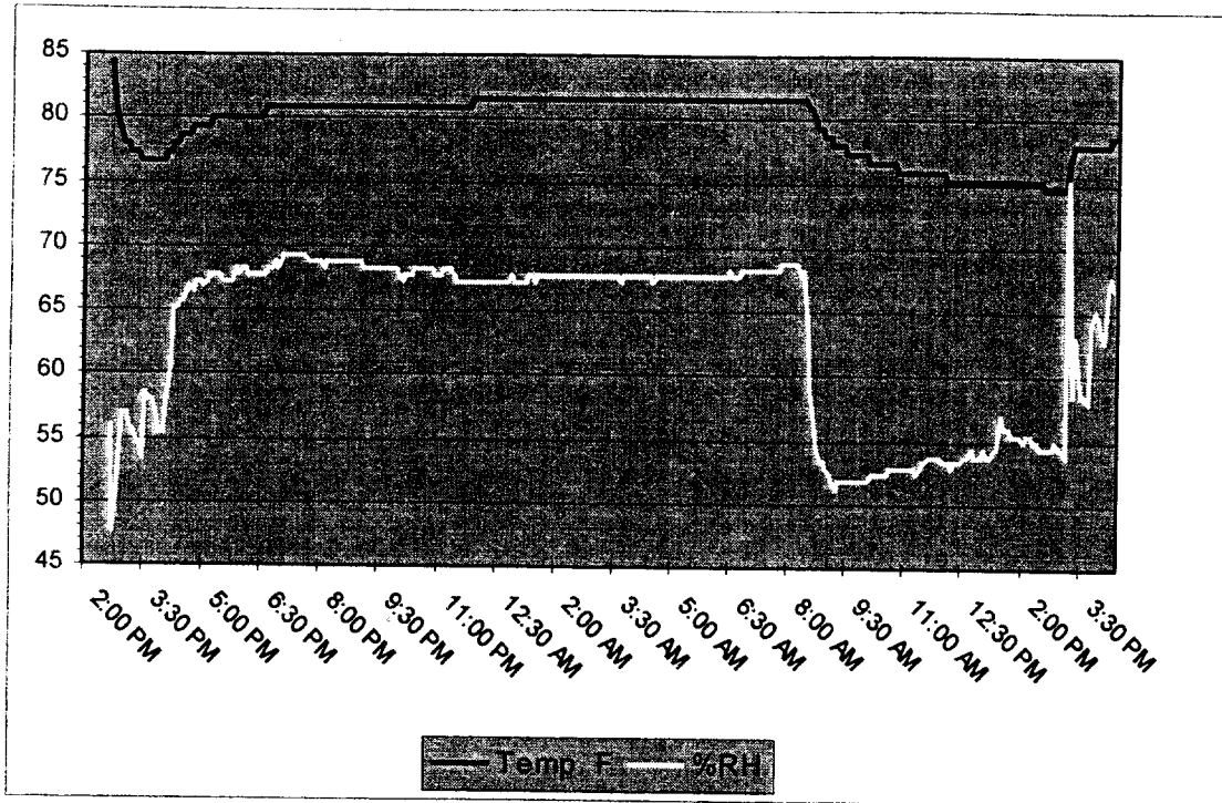
Figure 13. Hobo Instrument's Temp. and %RH Measurements in Room 350
