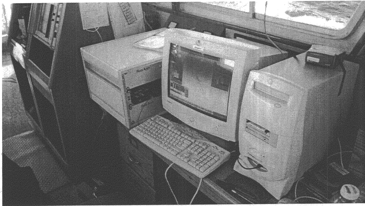
Figure 2-2. RoxAnn Seabed Classification System in operation aboard Hickson .
