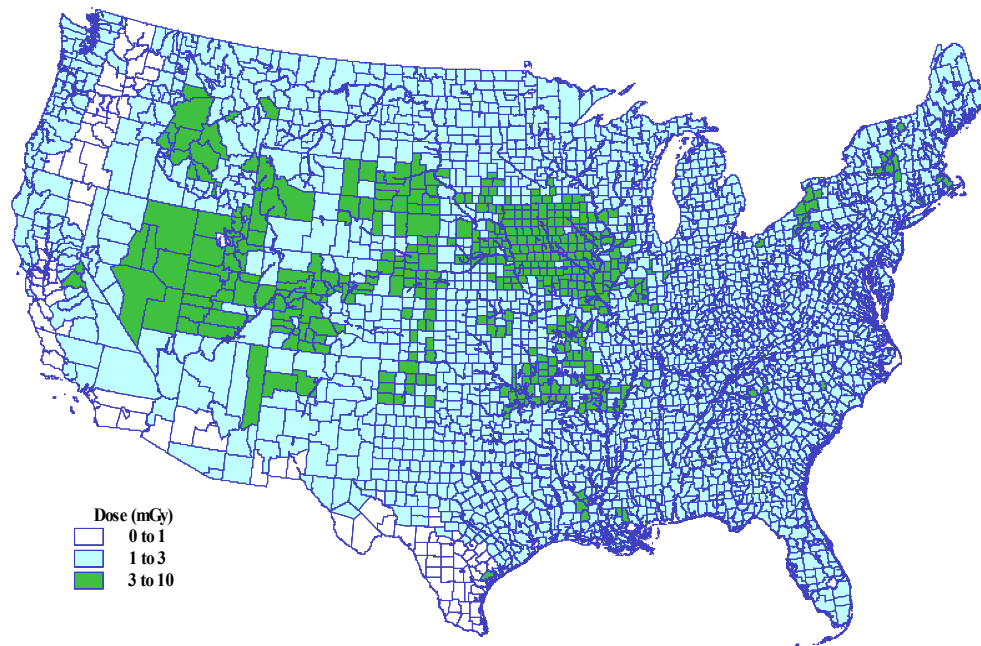
Figure. Preliminary estimates of the total radiation dose (milliGray [mGy]) to the red bone marrow of children born 1 January 1951 from NTS and global fallout for all radionuclides.
