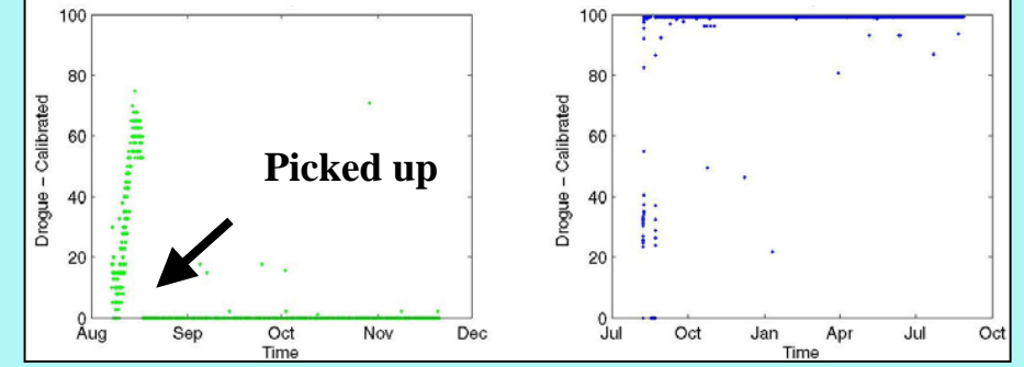
Cluster 8
