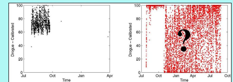
Cluster 7
