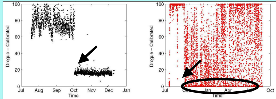
Cluster 6
