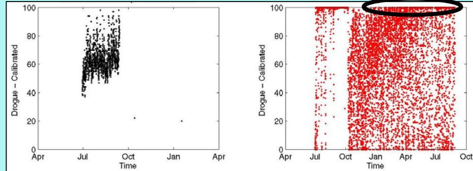
Cluster 5
