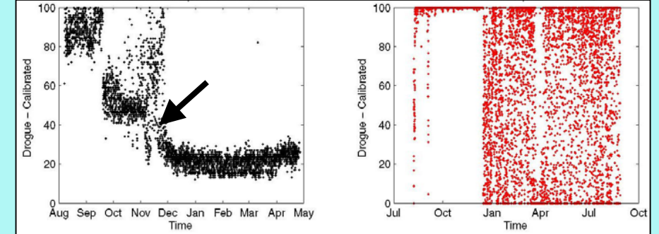
Cluster 8
