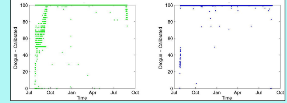
Cluster 7
