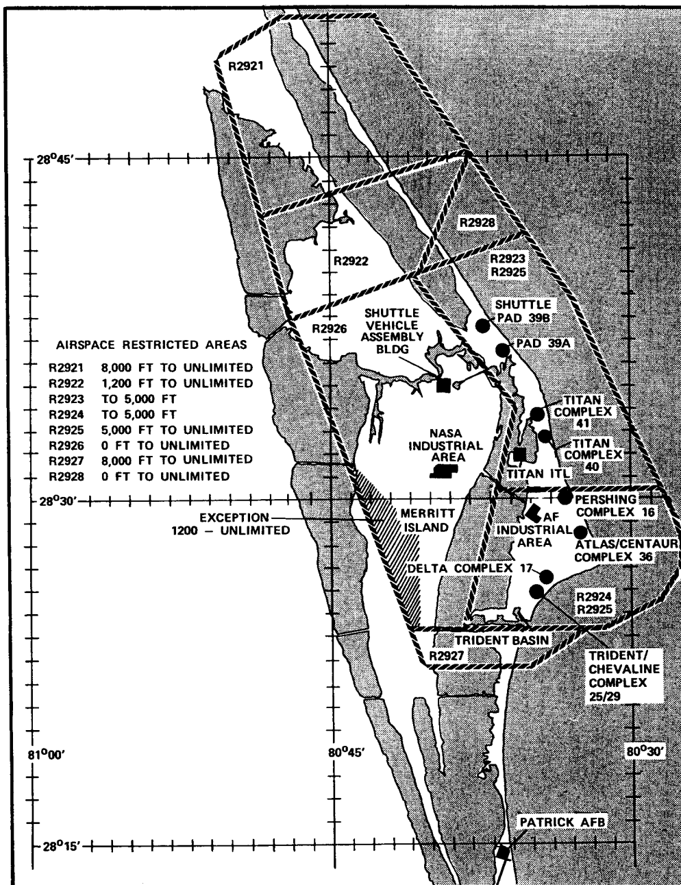
Figure C13.F2. ESMC Launch, Base, Industrial, and Restricted Areas
