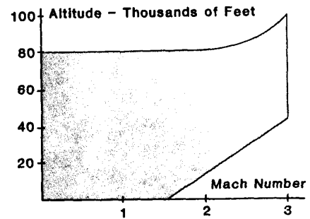
Figure C10.F1. NAPC Facility Capability
