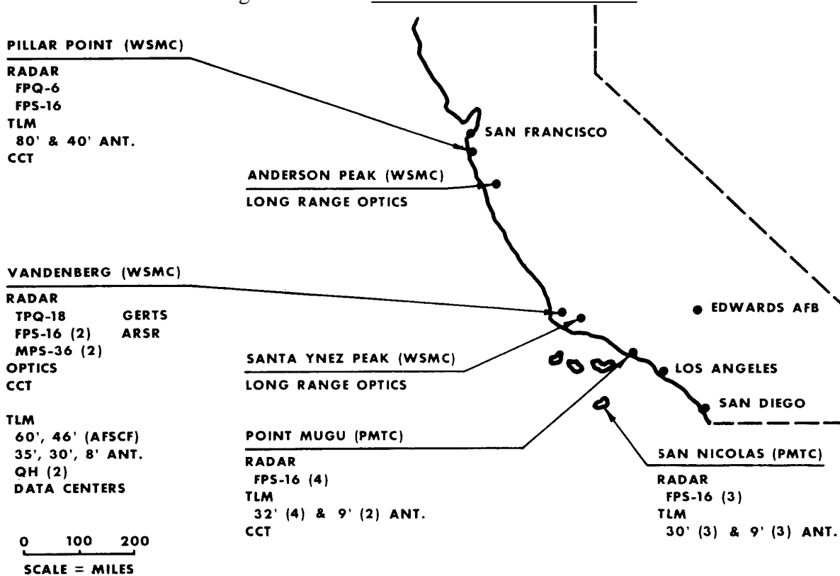
Figure C14.F2. WSMC West Coast Locations
