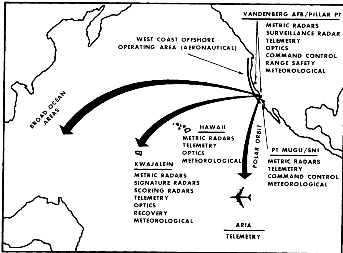
Figure C14.F1. Western Test Range
