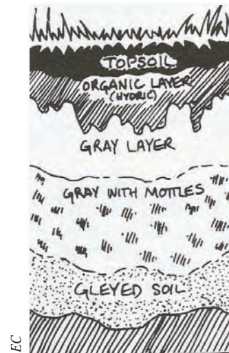
Typical soil profile in a wetland
