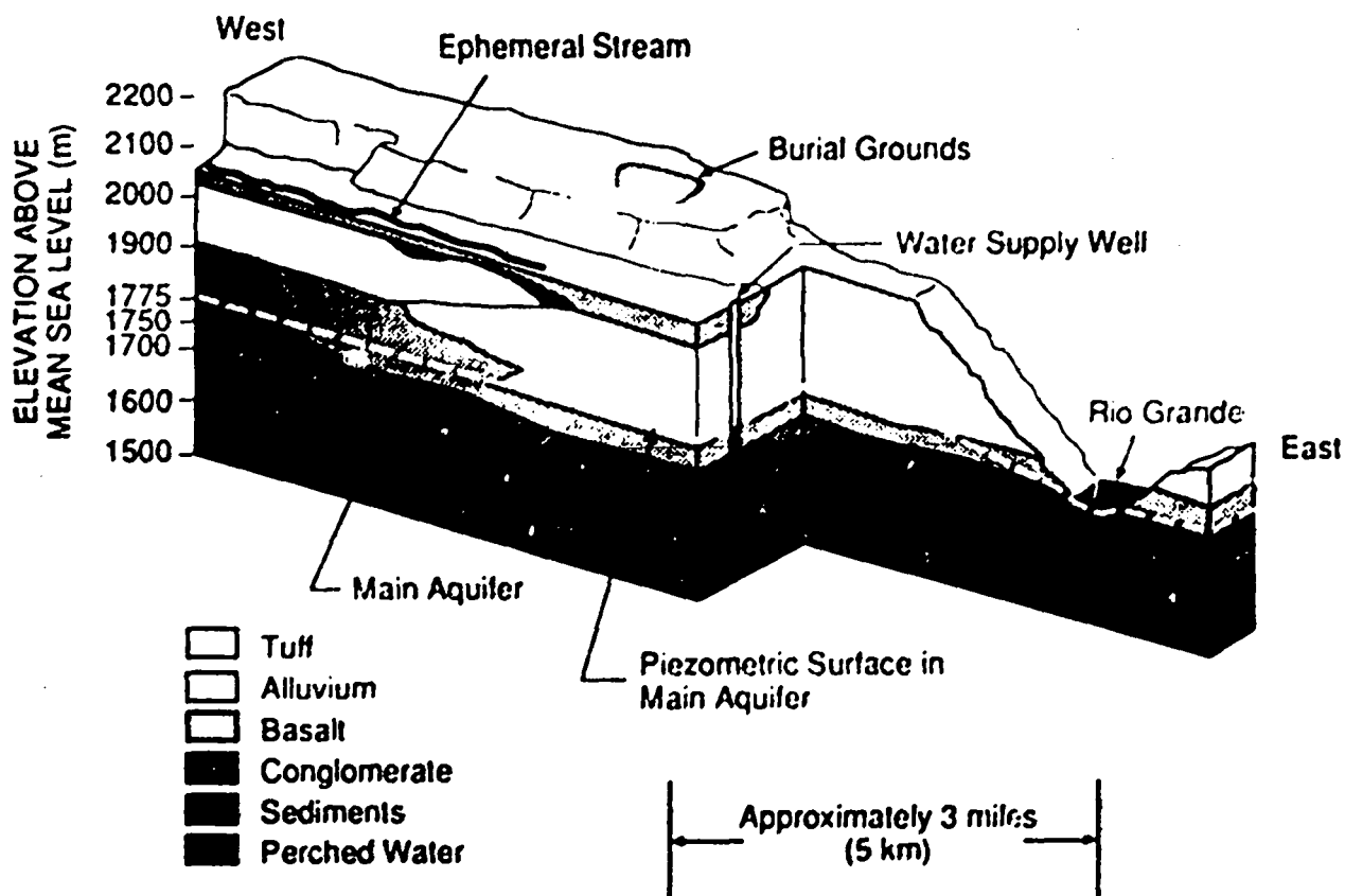
Fig. 6. Conceptual illustration of geologic-hydrologic relationship in Los Alamos area.
