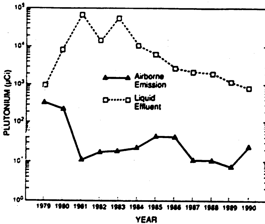
Fig. 11. Summary of plutonium releases (airborne emissions and liquid effluents).
