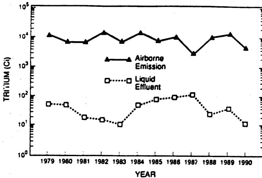
Fig. 10. Summary of tritium releases (airborne emissions and liquid effluents).
