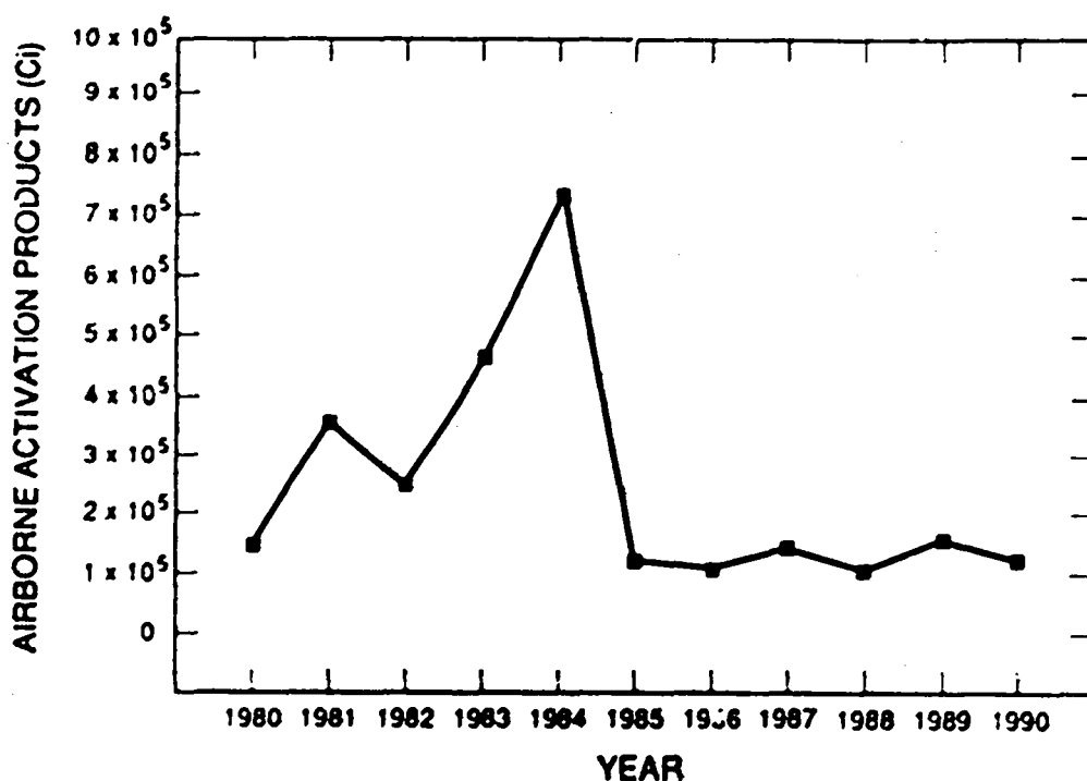
Fig. 12. Airborne activation product emissions (principally, 10 C, 11 C, 12 N, 16 N, 14 O, 15 O, 41 Ar) from LAMPF, the Los Alamos Meson Physics Facility (TA-53).
