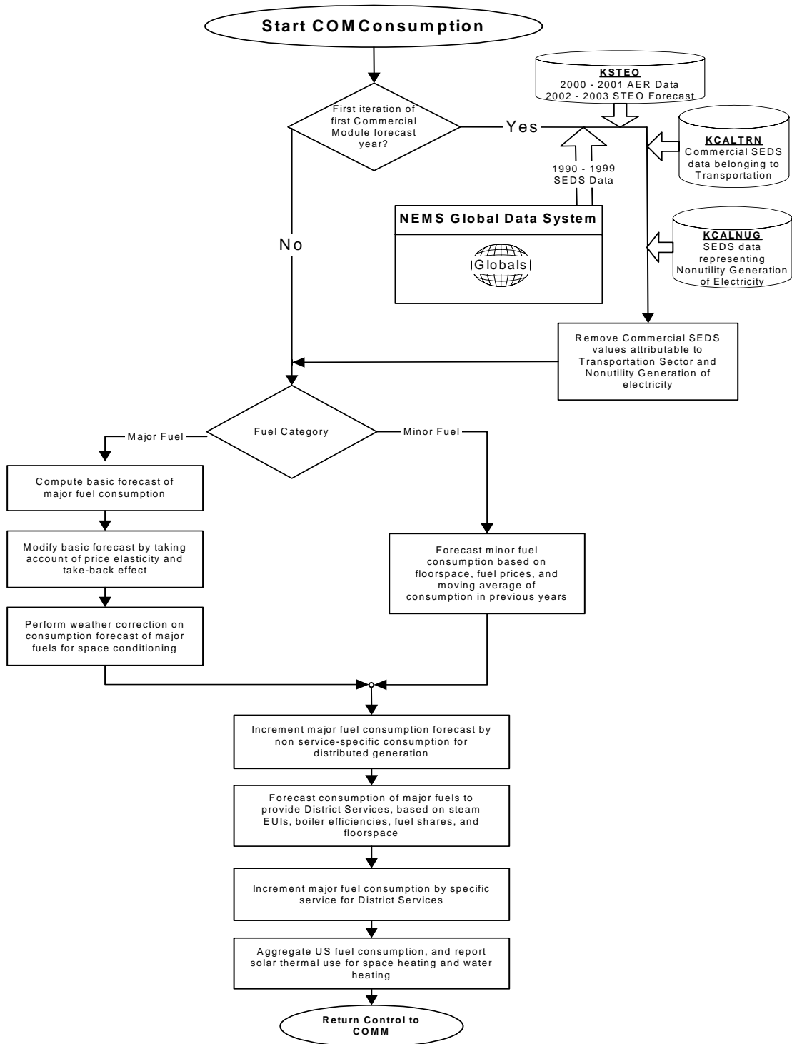
Figure 8. COMConsumption Calculation Process Flow
