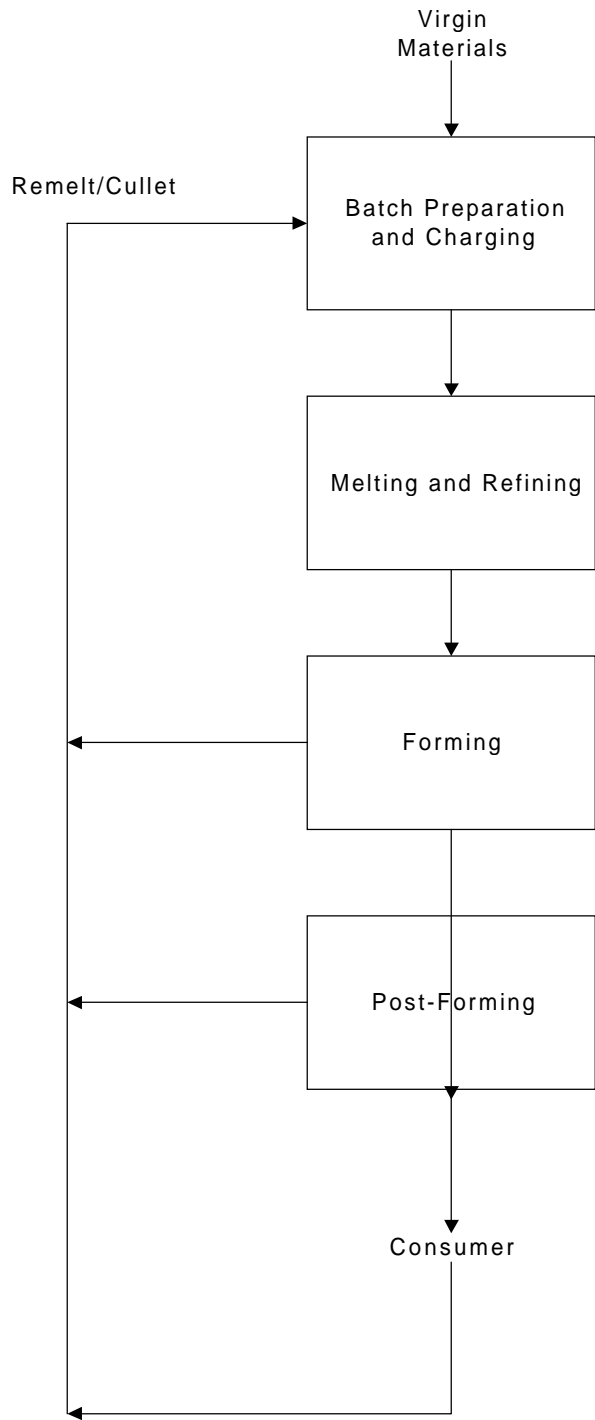
Figure 5. Glass and Glass Products Industry Process Flow
