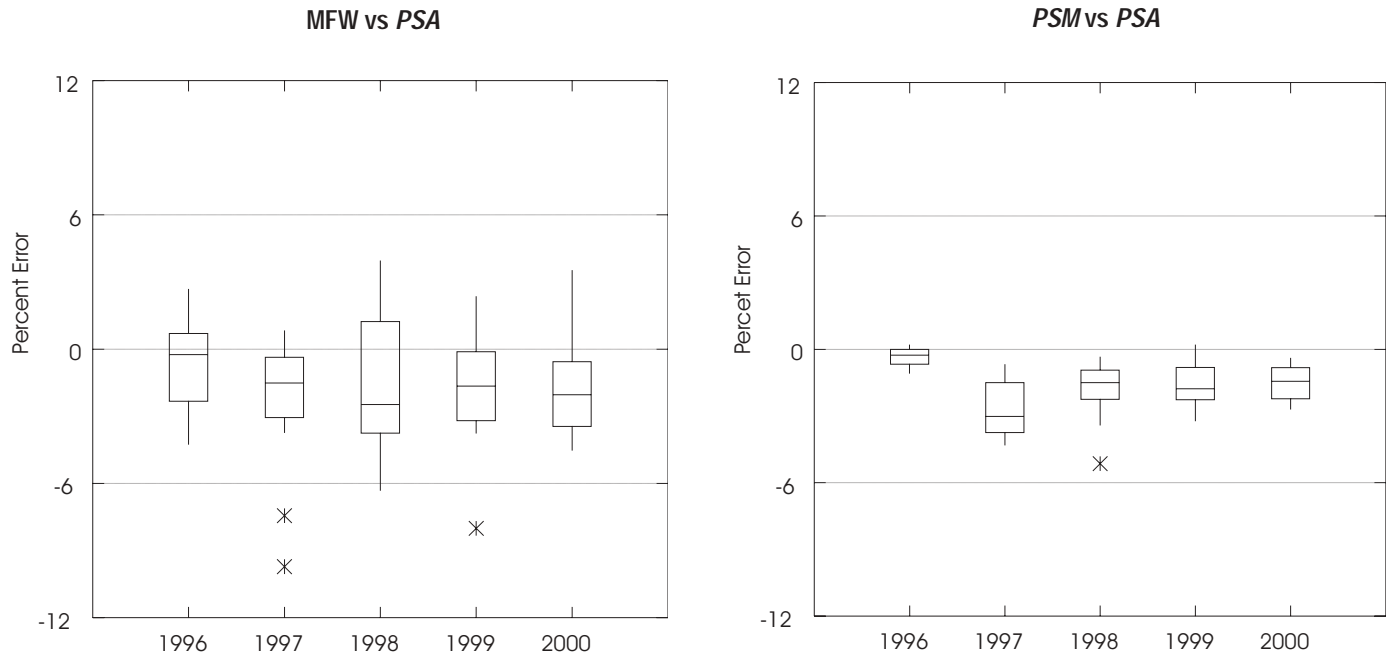
Figure FE9. Range of Percent Errors for MFW and PSM Crude Oil Imports Excluding SPR Data, 1996 - 2000
