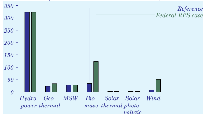
Figure 11. Renewable electricity generation in two cases, 2020 (billion kilowatthours)
