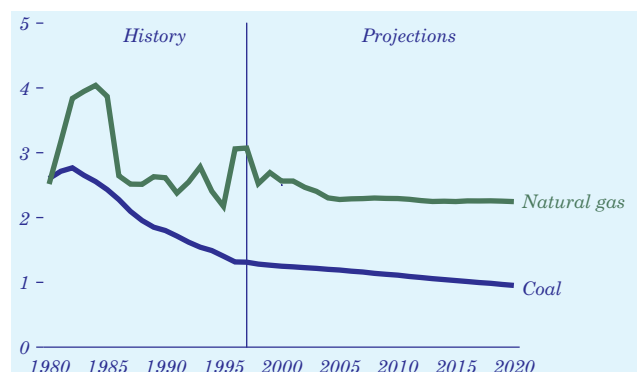
Figure 73. Average fuel costs for coal- and gas-fired generating plants, 1980-2020 (1997 mills per kilowatthour)
