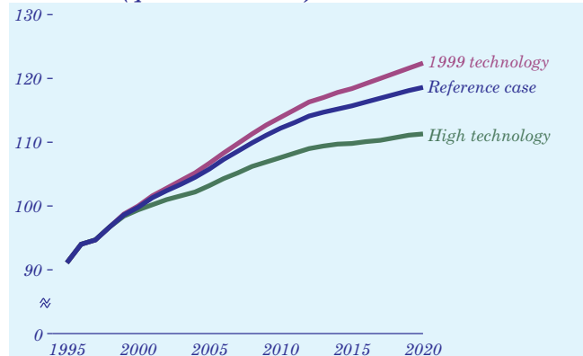
Figure 31. U.S. energy consumption in three cases, 1997-2020 (quadrillion Btu)
