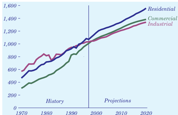
Figure 67. Annual electricity sales by sector, 1970-2020 (billion kilowatthours)
