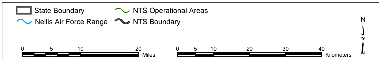
Figure 7.1 Hydrographic Subbasins on or near the Nevada Test Site
