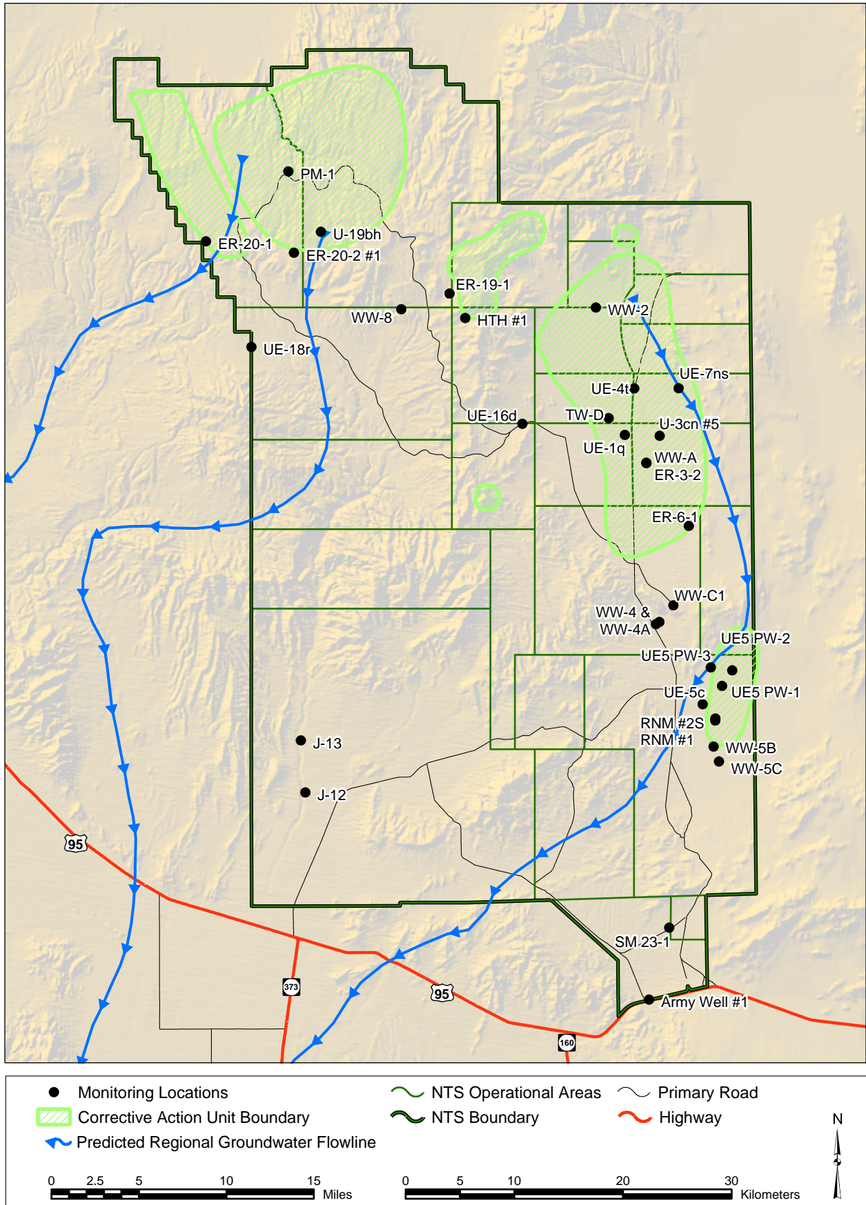
Figure 8.2 Nevada Test Site Onsite Groundwater Monitoring Locations - 2000
