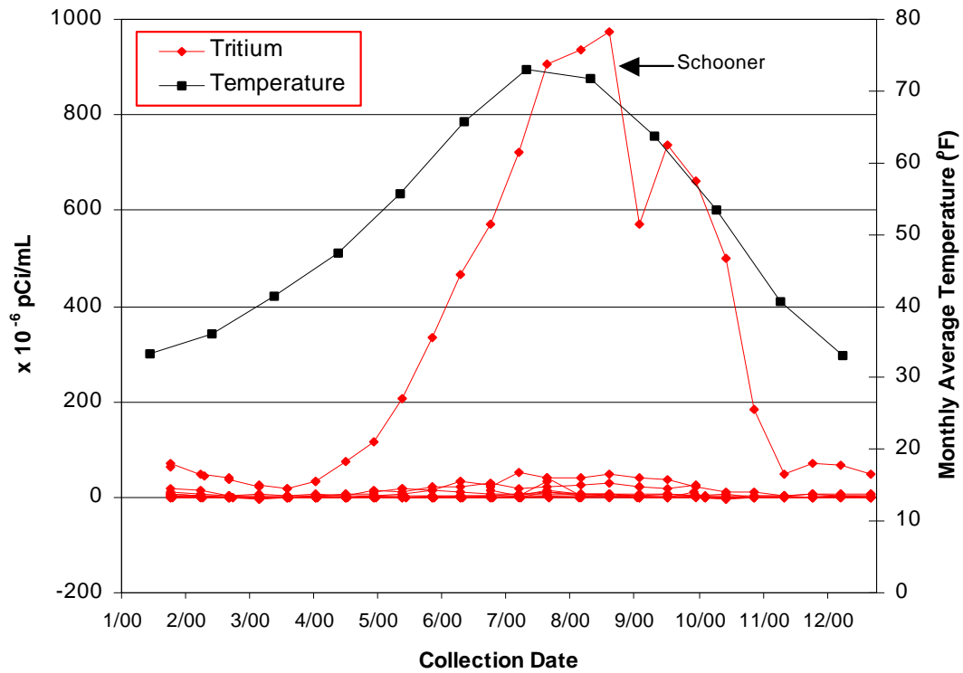
Figure 5.10 Time Series Plot of HTO vs Temperature
