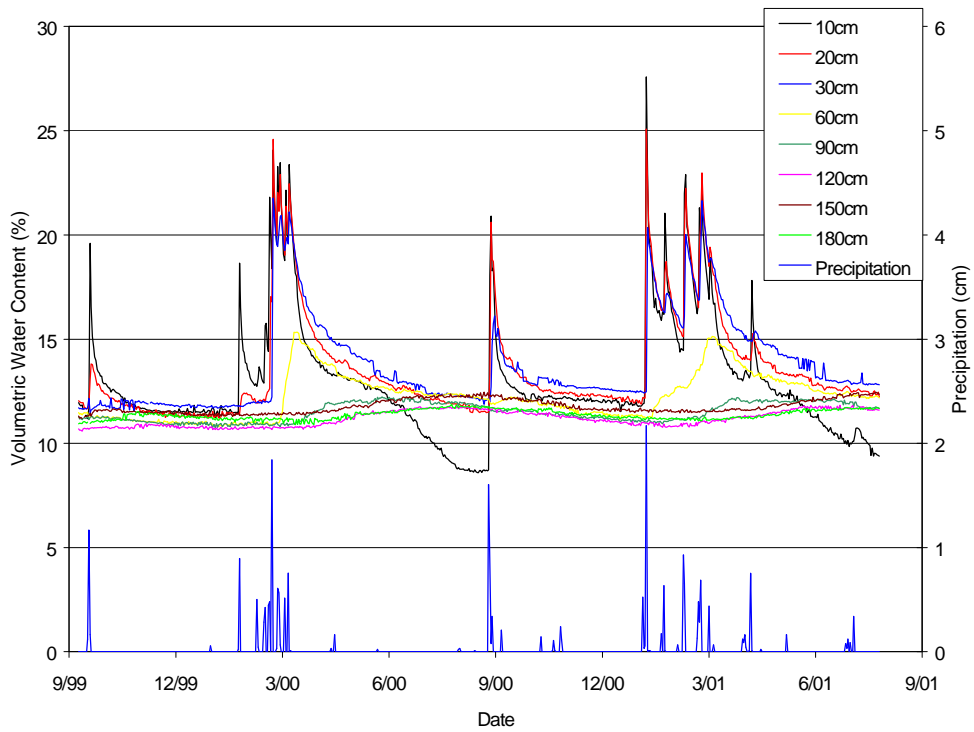
Figure 8.10 Soil Water Content in Pit 3 Waste Cover (North Site) Using an Automated Monitoring System
