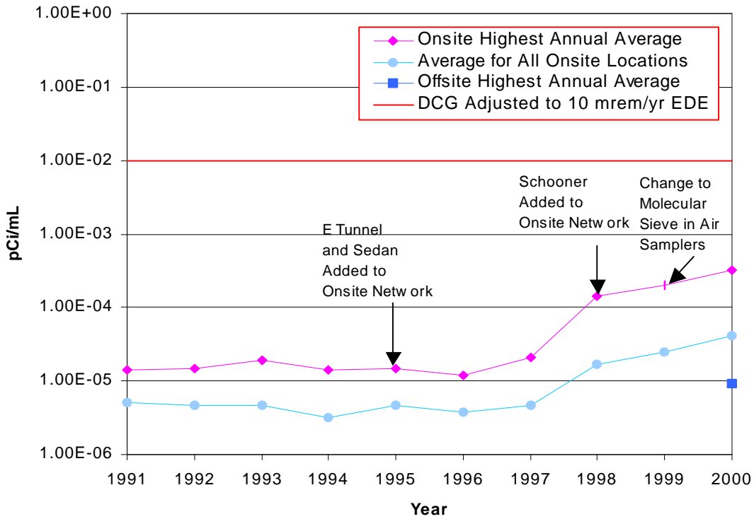
Figure 5.12 Trend in Annual Averages for HTO Concentrations Onsite
