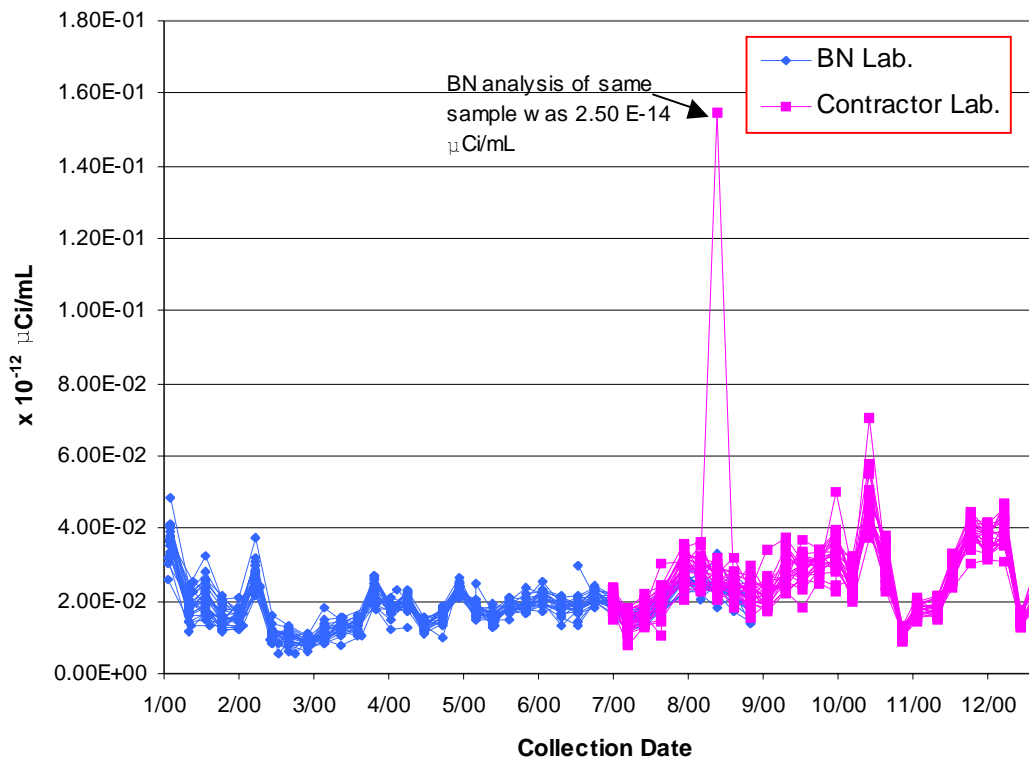
Figure 5.3 Times Series Plot of Beta - 2000
