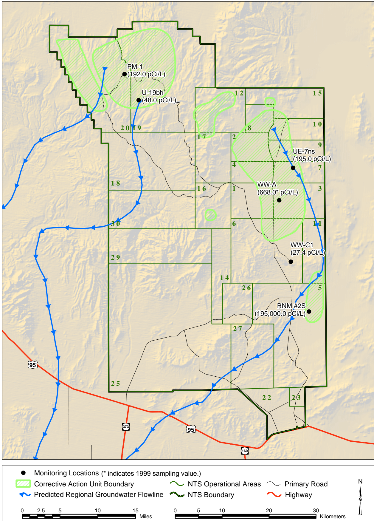
Figure 8.5 Nevada Test Site Groundwater Monitoring Locations With a History of Detectable Tritium - 2000
