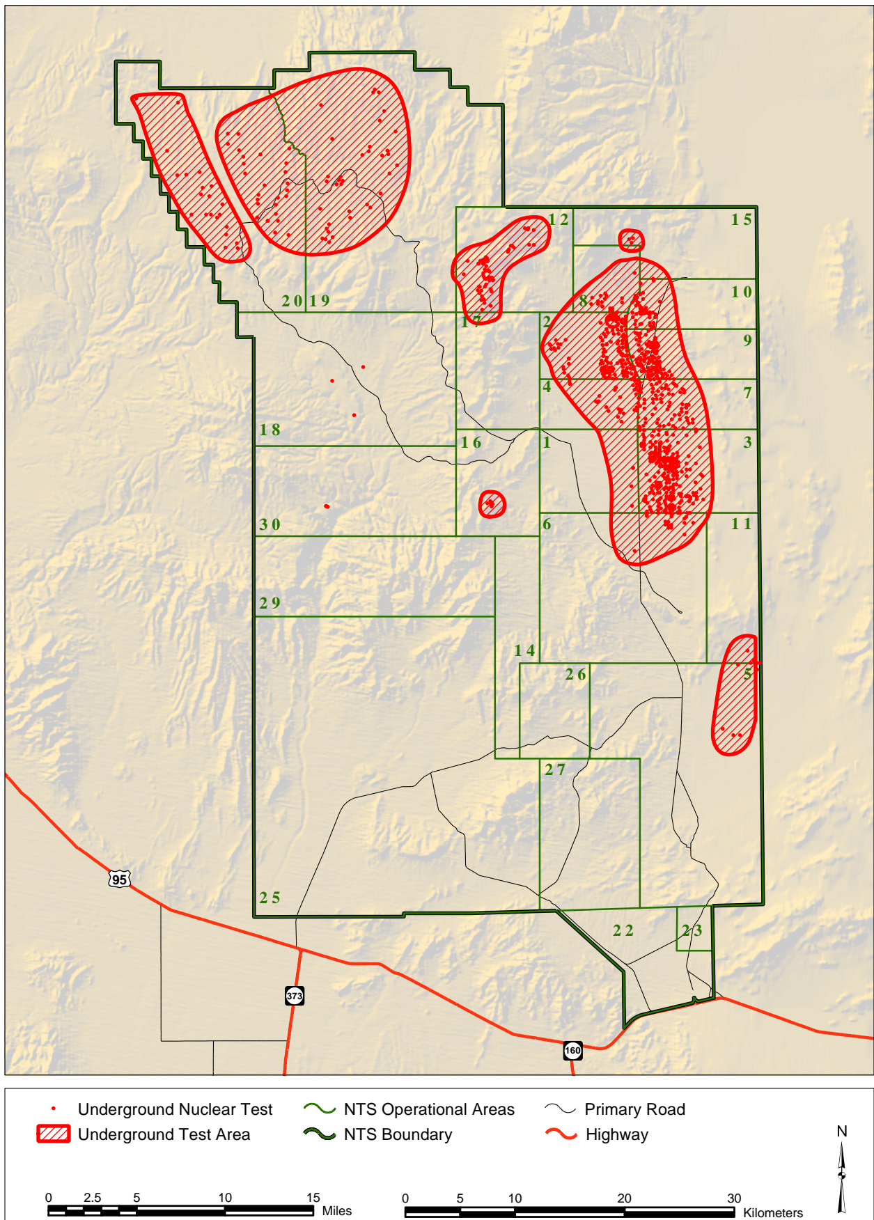
Figure 8.1 Areas of Potential Groundwater Contamination on the Nevada Test Site
