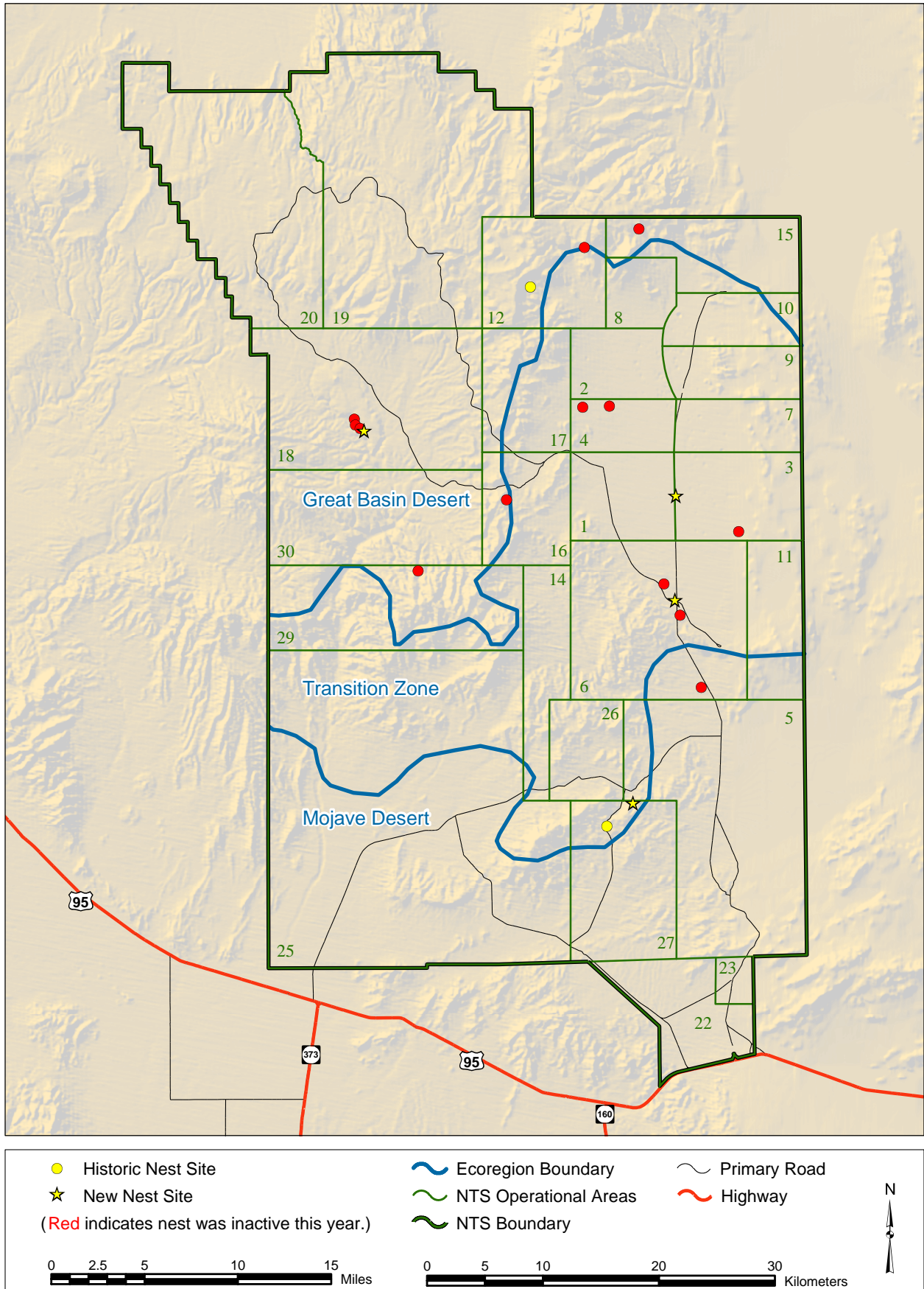
Figure 6.3 Location of Known Raptor Nests on the Nevada Test Site - 2000
