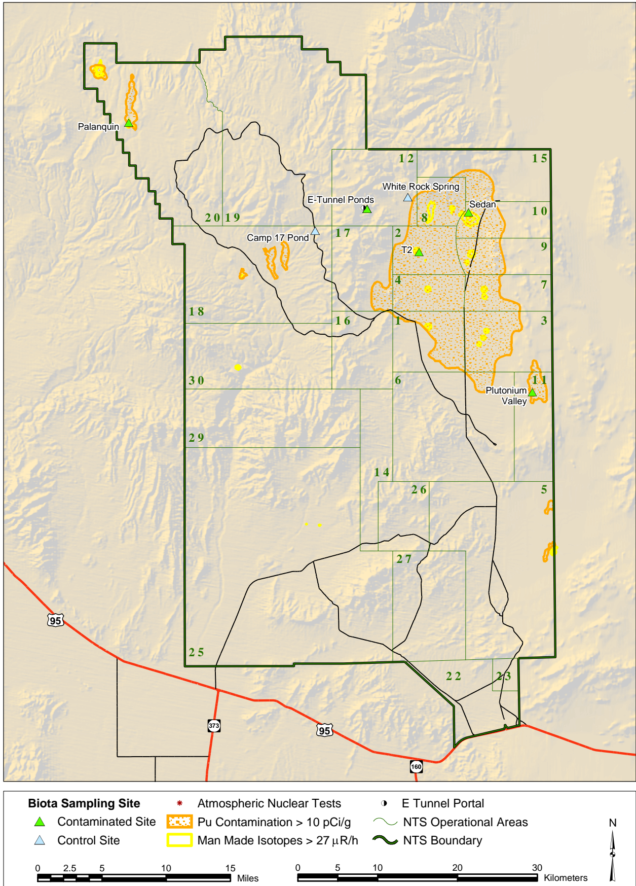
Figure 5.16 Nevada Test Site Onsite Surface Biota Radiological Monitoring Sites - 2000
