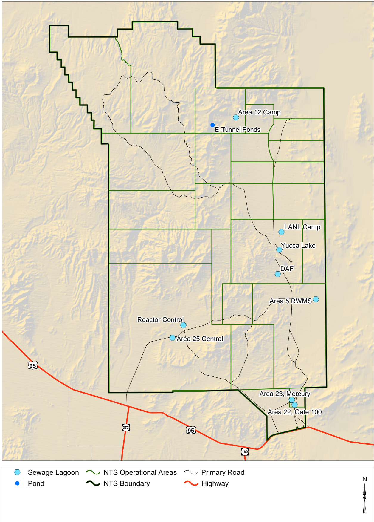
Figure 5.15 Surface Water Sampling Locations on the Nevada Test Site - 2000
