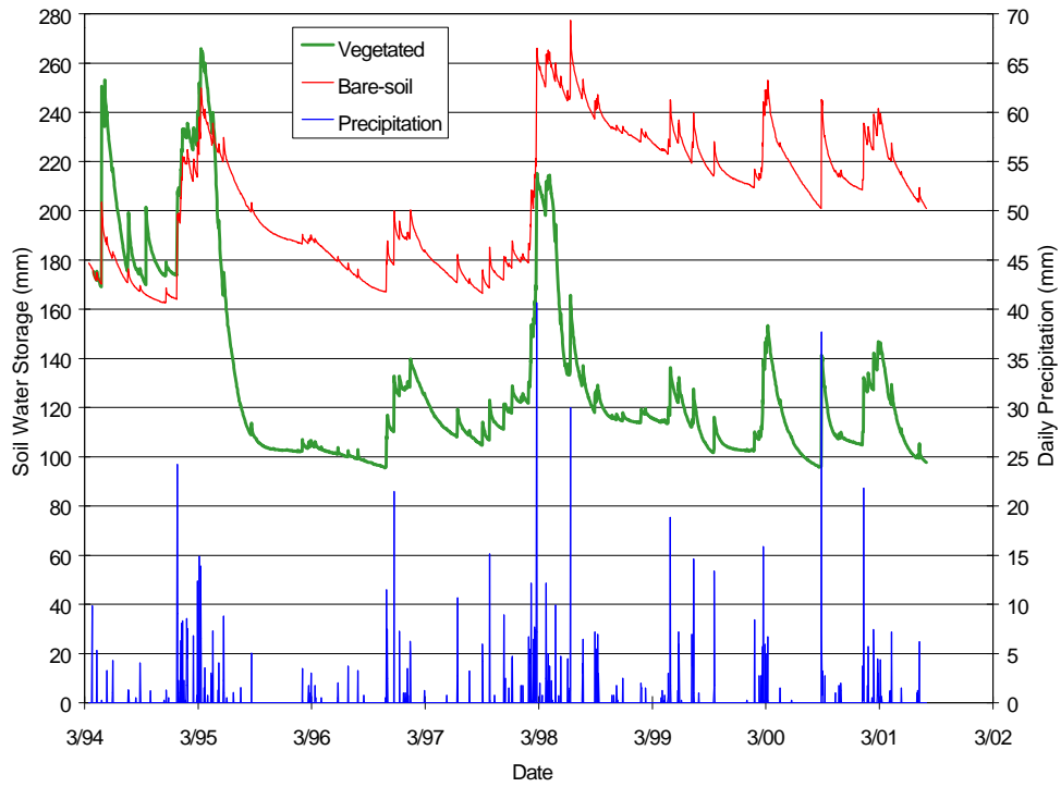
Figure 8.9 Weighing Lysimeter and Precipitation Data from March 1994 through July 2001
