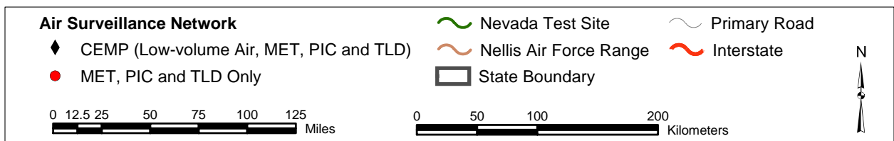
Figure 5.19 CEMP, MET, PIC and Air Sampling Sites on or near the Nevada Test Site - 2000
