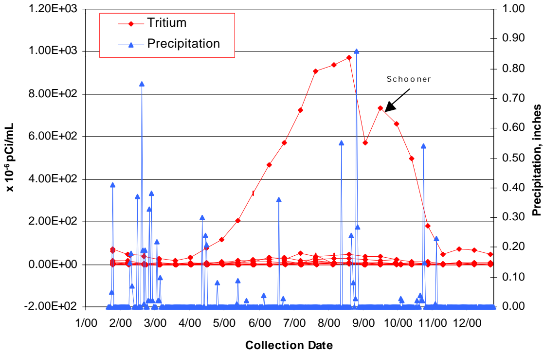
Figure 5.11 Time Series Plot of HTO vs Precipitation
