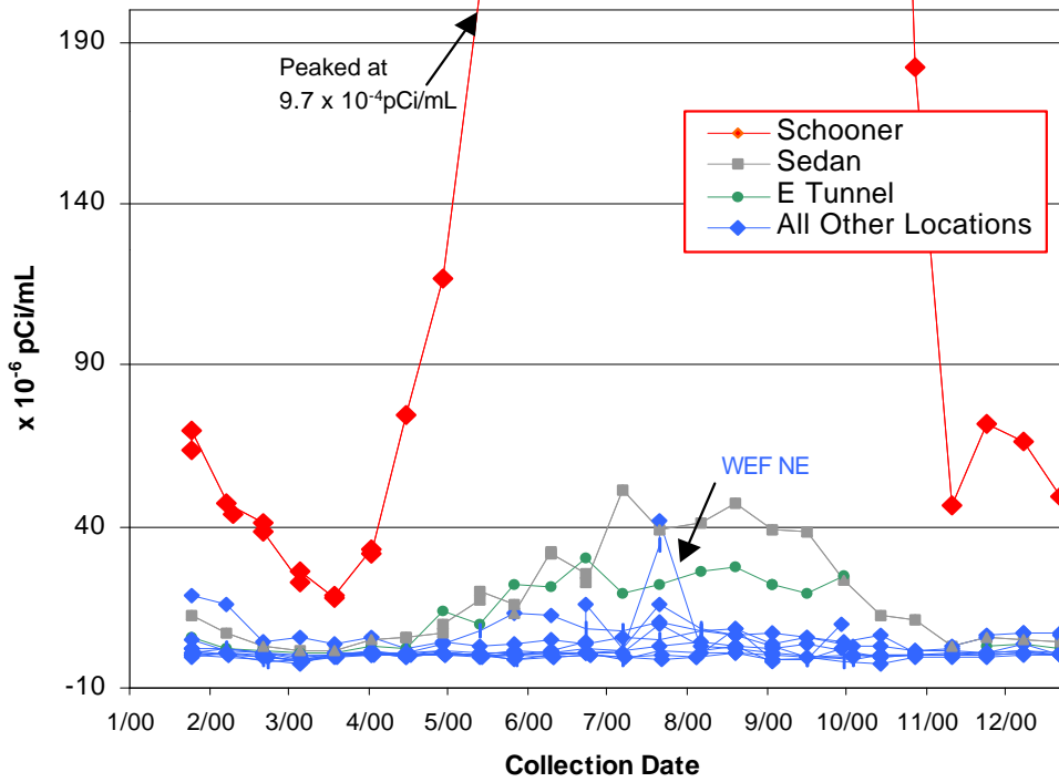
Figure 5.9 Time Series Plot of Tritium in Air - 2000
