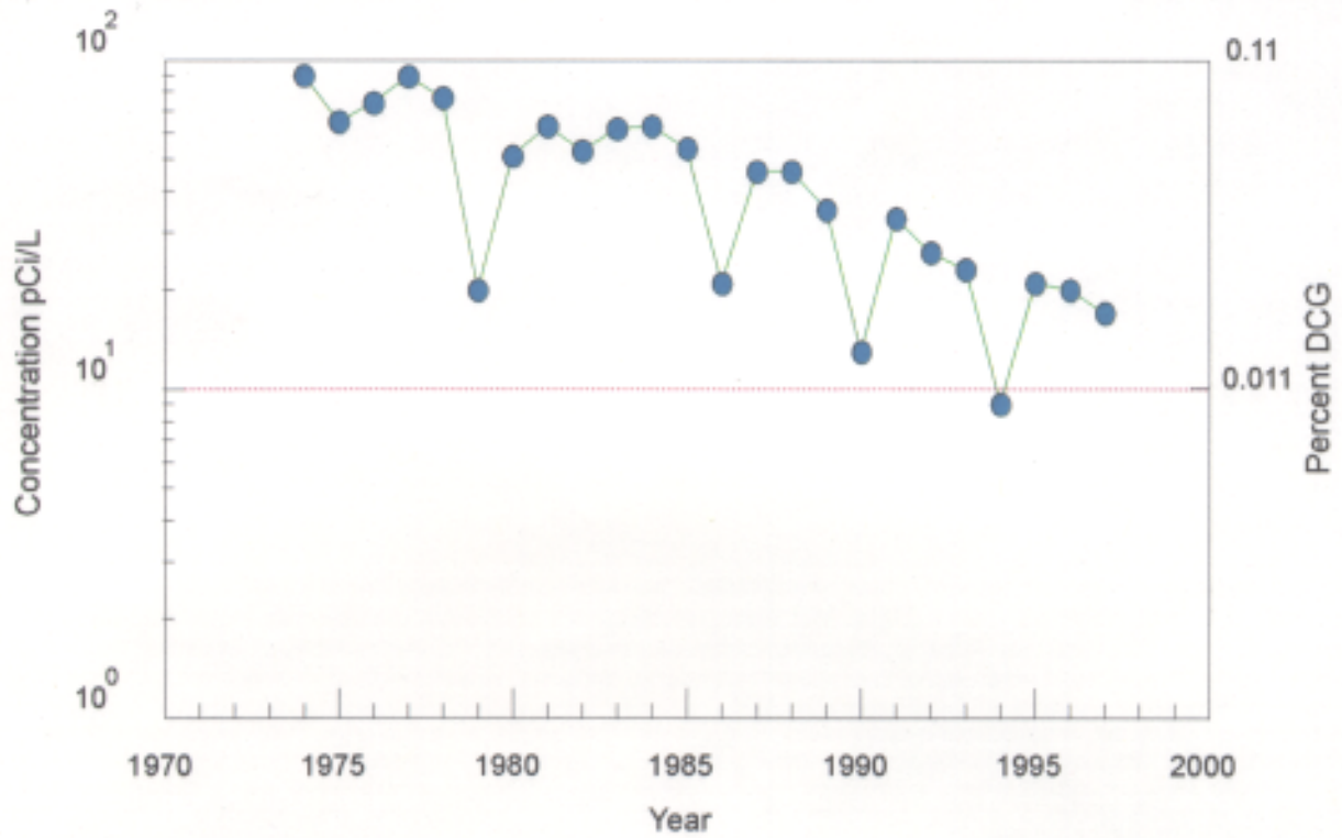
Figure 5.15 Tritium Results Trends in Baxterville, Public Drinking Water Supply - 1997
