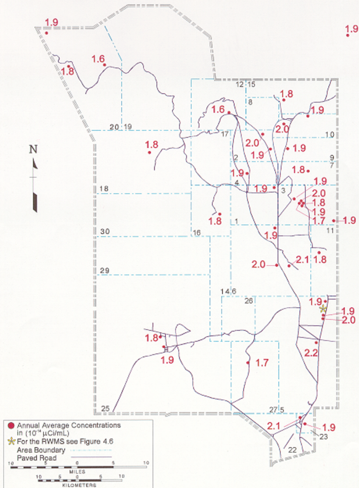
Figure 4.5 Annual Average Gross Beta from Air Sampling - 1997
