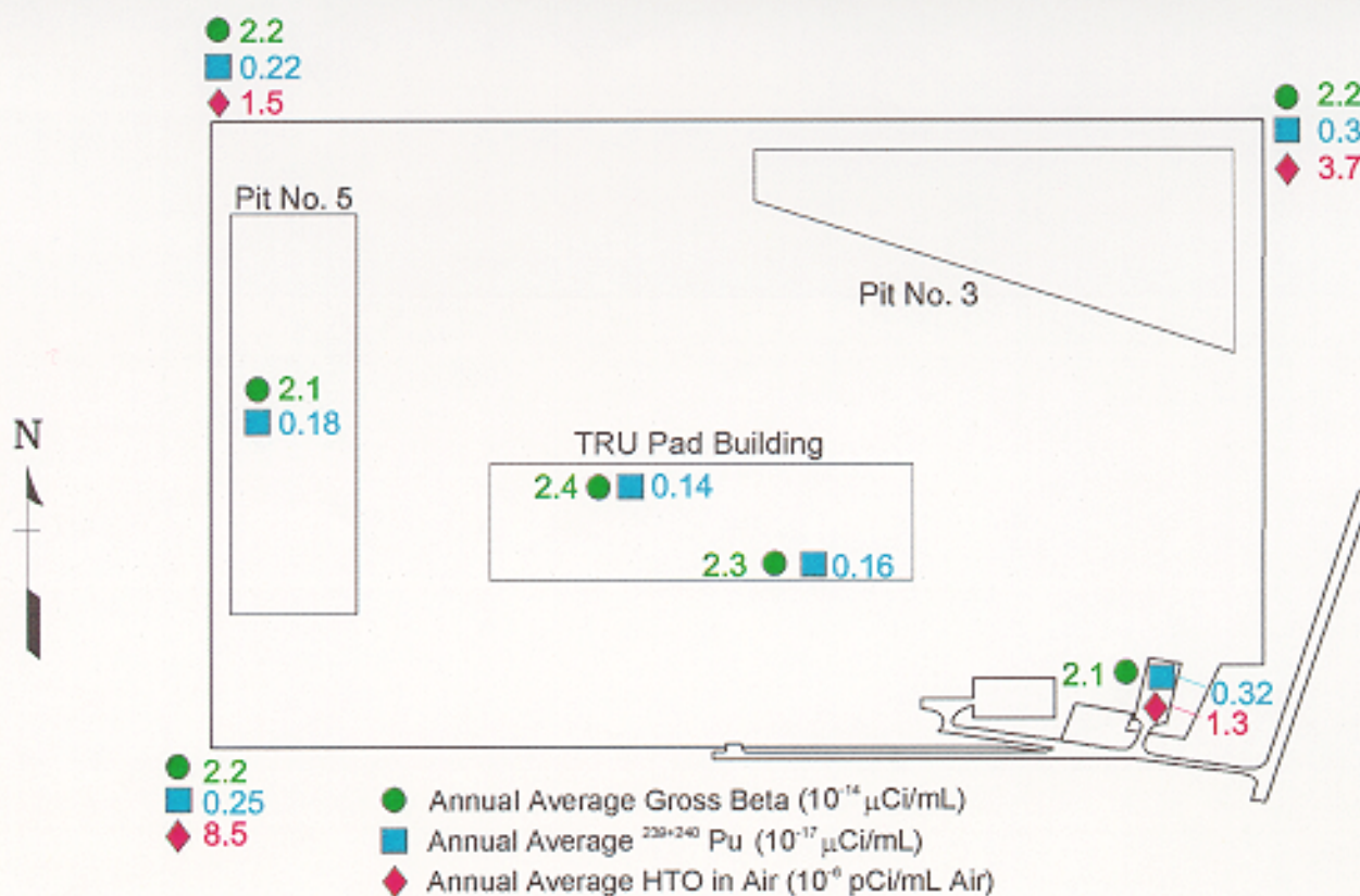
Figure 4.6 Air Monitoring Results for RWMS-5 - 1997
