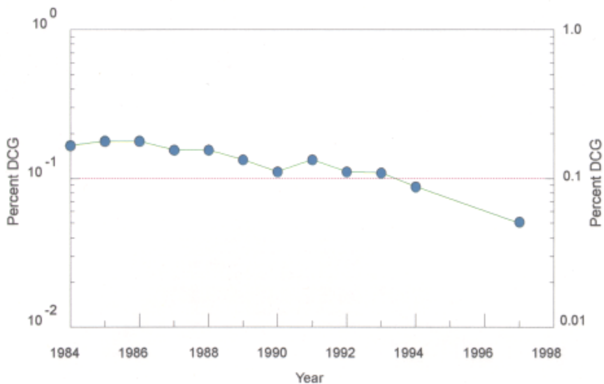
Figure 5.6 Trends in Tritium Concentration, Test Well B on the NTS
