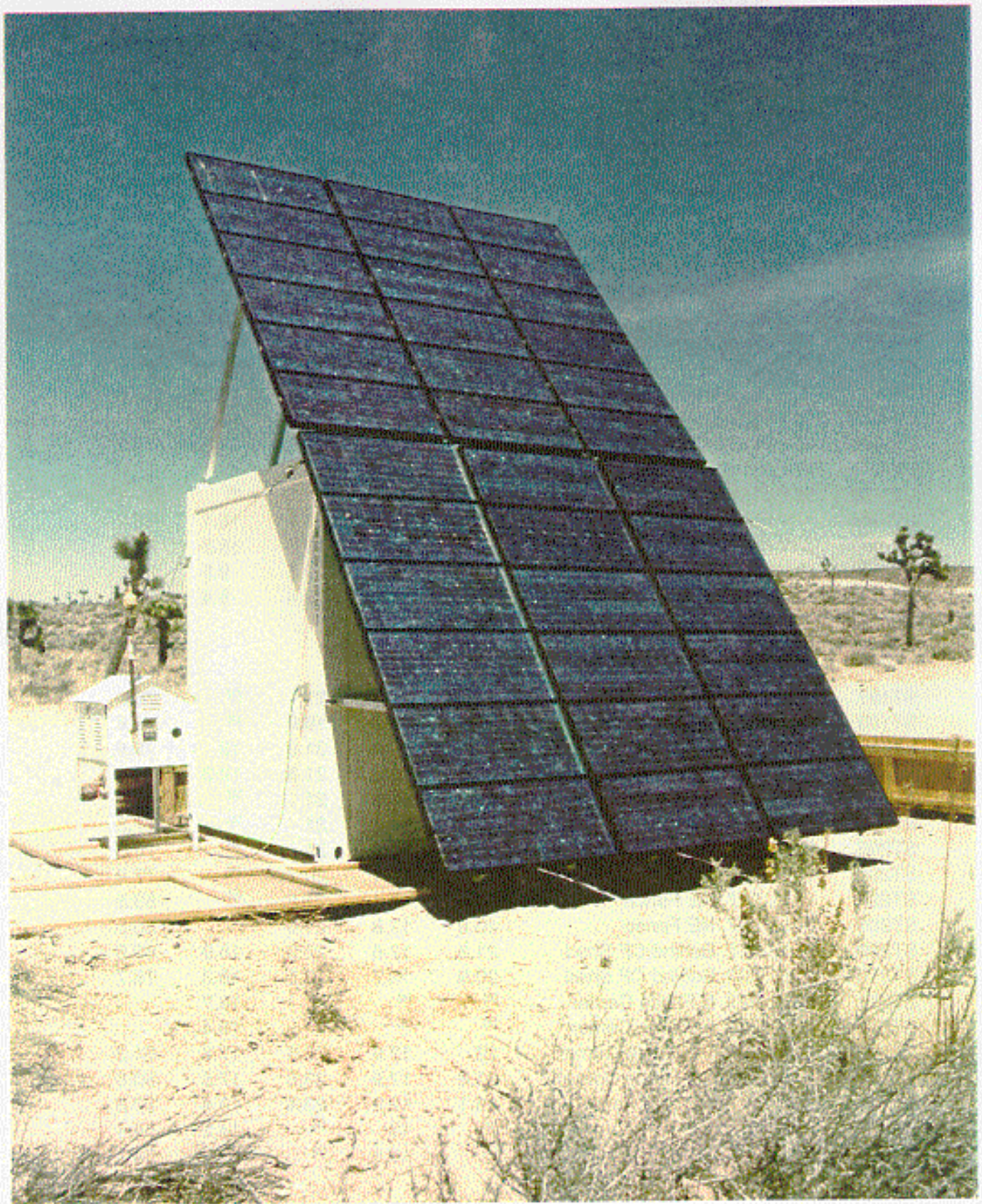
Solar Air Sampler Located at Well ER-3-1
