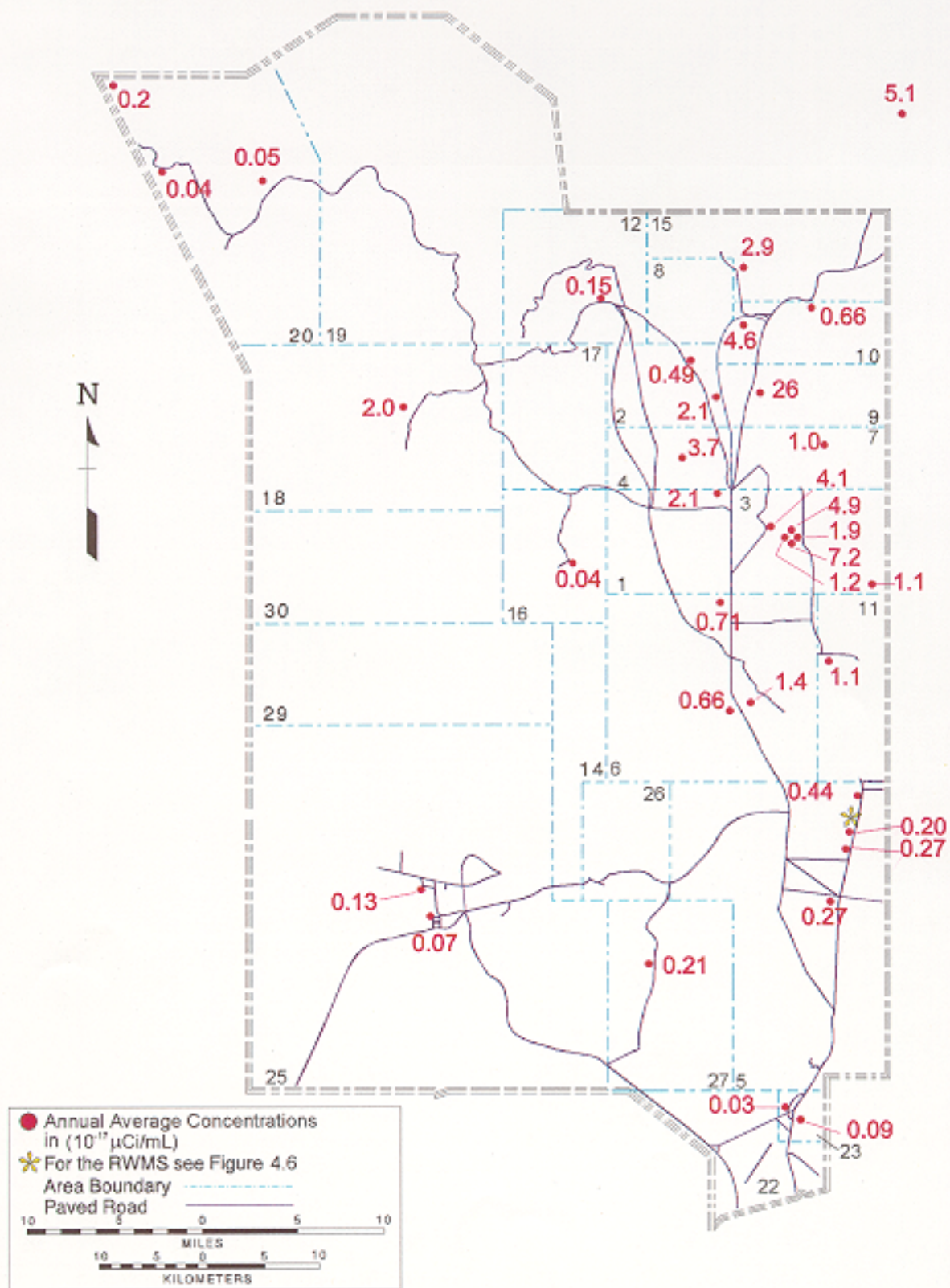
Figure 4.8 Annual Average ^{239+240}\text{Pu} in Air on the NTS - 1997
