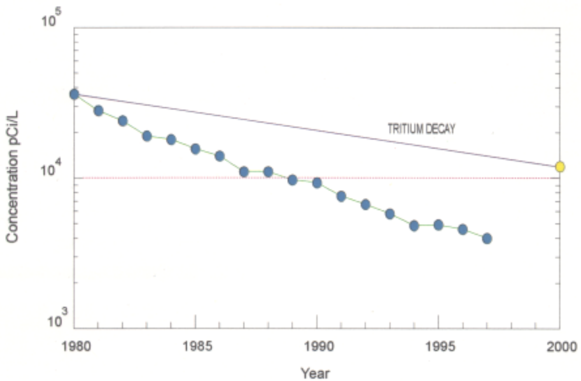
Figure 5.16 Tritium Results in Well HM-S, SALMON Site, Project DRIBBLE - 1997
