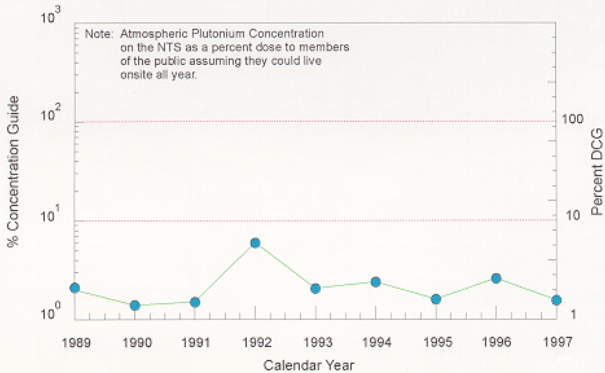
Figure 4.9 Trend in Annual Averages for Plutonium Concentration on the NTS
