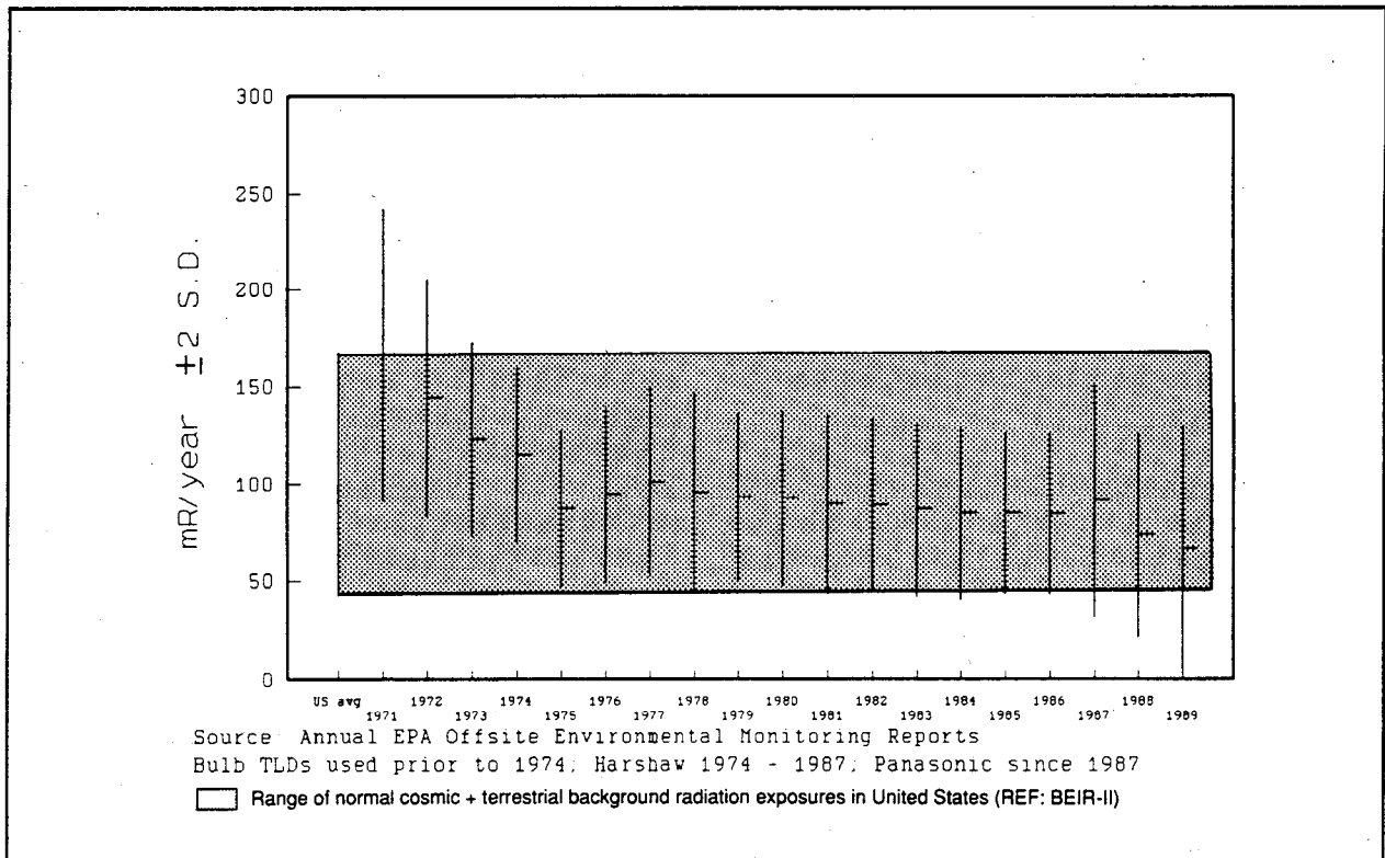
Figure 35. Historical Trends — TLD Exposures at Fixed Environmental Stations — 1971-1989.
