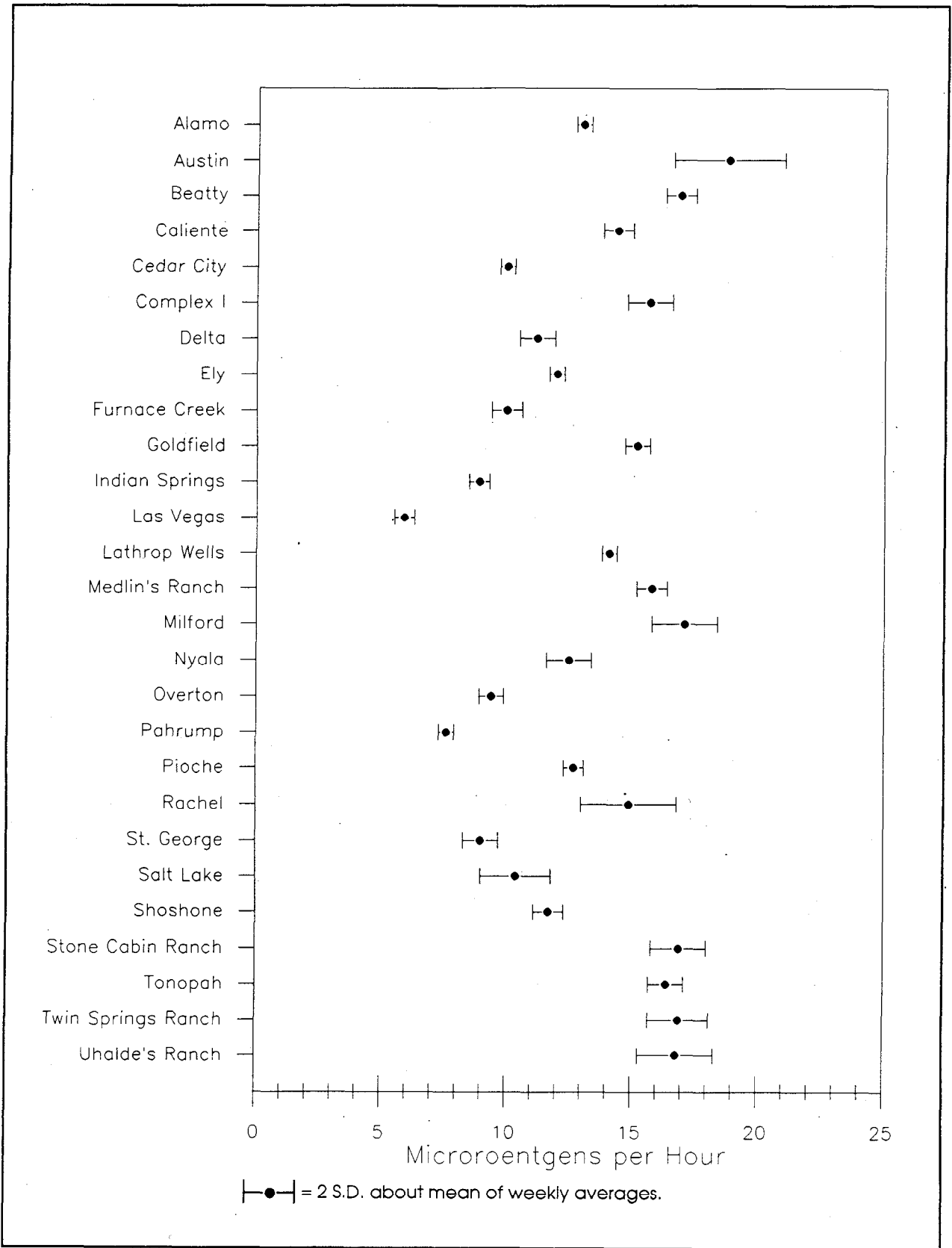
Figure 42. Annual PIC Averages by Station in Microrentgens per Hour — 1989.
