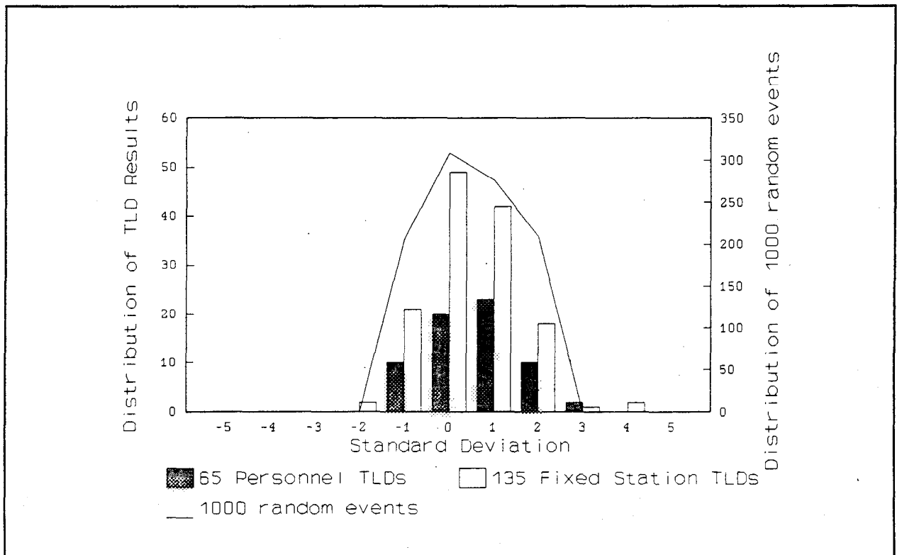
Figure 38. Frequency Distribution Analysis Fixed Station and Personnel TLDs — 1989.
