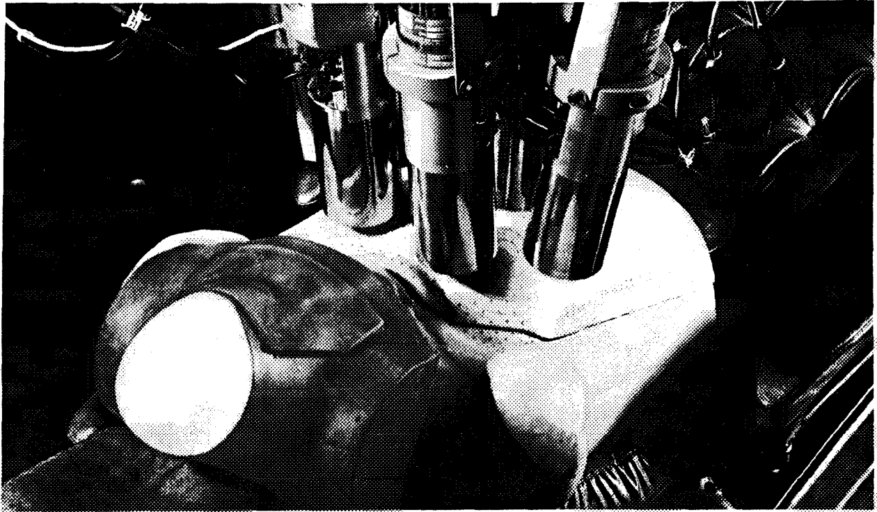
Figure 46. Calibration of the Semi-Planar Detectors for Transuranic Radionuclides Using the LLNL Realistic Lung Phantom. (The thyroid and coaxial detectors are calibrated for the radioiodines with the thyroid neck phantom.)
