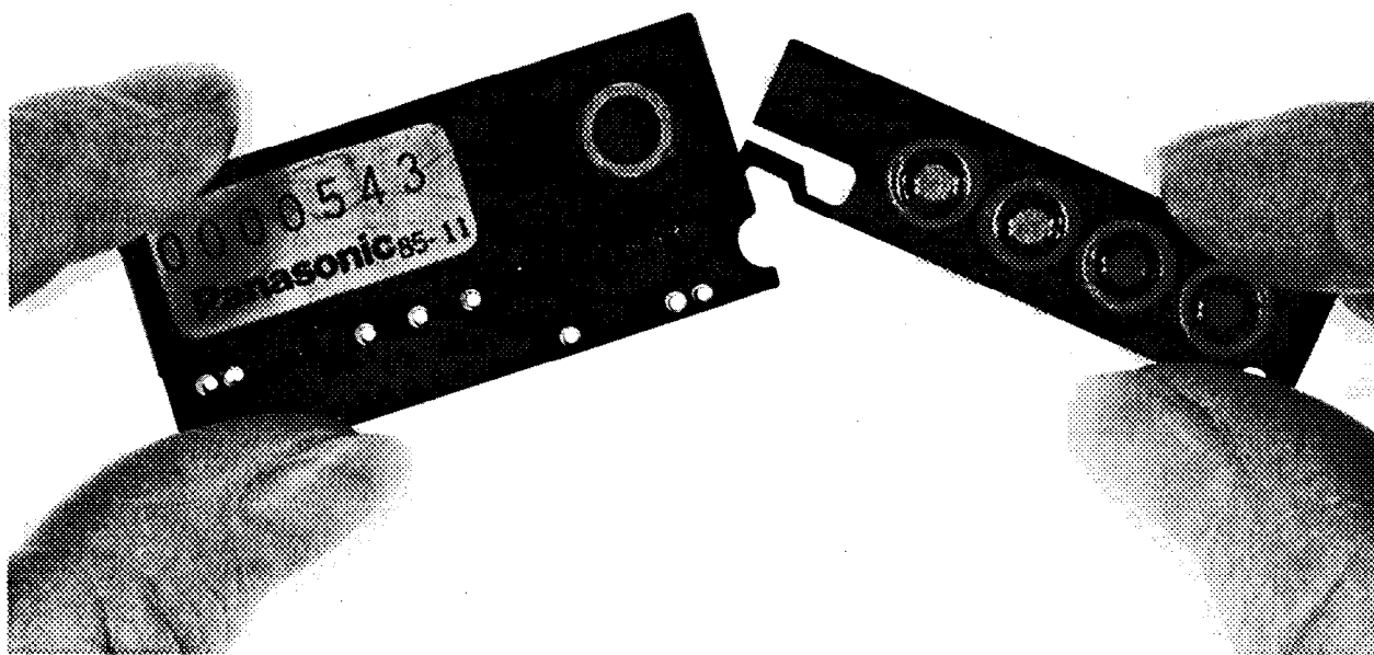
Figure 29. Construction of a Typical Panasonic Dosimeter.
