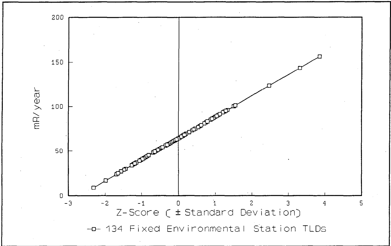
Figure 37. Distribution of Fixed Station TLD Results — 1989.
