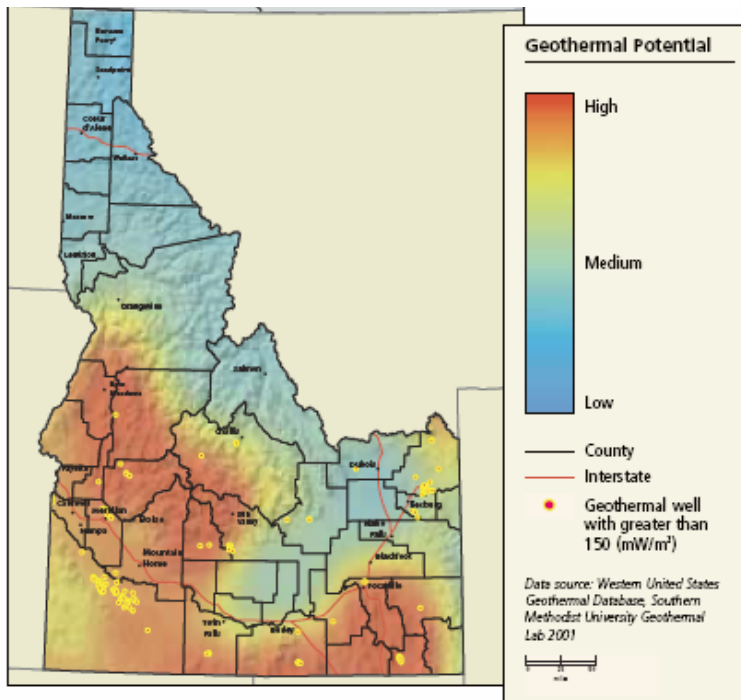
Figure 7: Map of Idaho's Geothermal Potential
