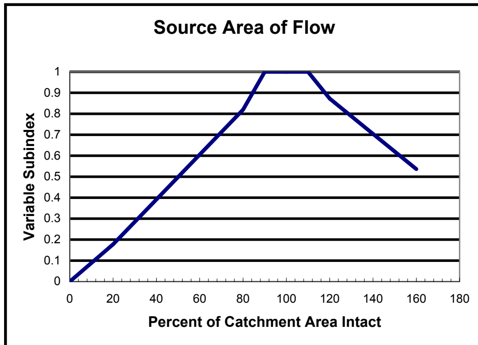
Figure 8. Relationship of the existing catchment to the variable subindex
