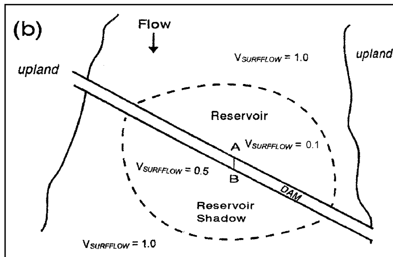
Figure 3. Alteration to hydrologic regime caused by an impediment to surface flow ( V_{SURFFLOW} ). (a) For dams that cross a flat perpendicular to the direction of flow, the elevation of the overflow point (A) is the same as that of the reservoir boundary (area within dotted line below C). The distance from A to C equals the distance from the outlet point (B) to the boundary of the reservoir shadow (area within dotted line above D). Assuming a constant gradient, if the gradient of the wet flat is 0.002 (0.2%) and the overflow point on the dam is 0.5 m high, then the distance from A to C and B to D is 250 m ( 0.5/0.002 ). Note: footprint of dam is treated as a fill (see V_{STORAGE} ). (b) Dam crossing a wet flat at angle that is not perpendicular to flow. The area upslope is determined by circumscribing a boundary of elevation equal to that of the outlet point, but its precise shape is unknown. The reservoir shadow is assumed to be the same size as the reservoir. The sub-index for V_{SURFFLOW} is 0.1 in the reservoir and 0.5 in the reservoir shadow in both examples.
