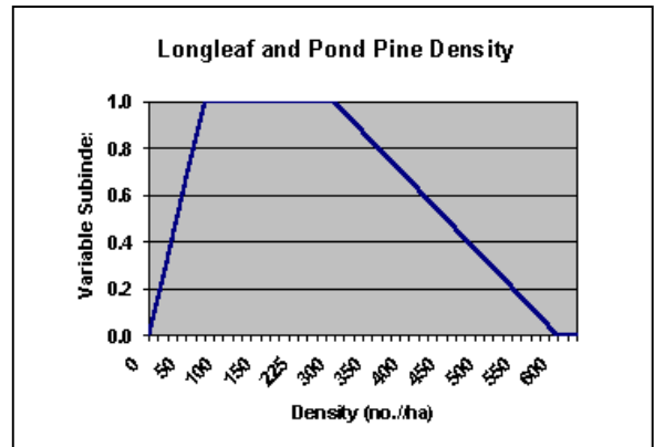
Figure 22. Relationship between canopy-size longleaf and pond pine density and functional capacity
