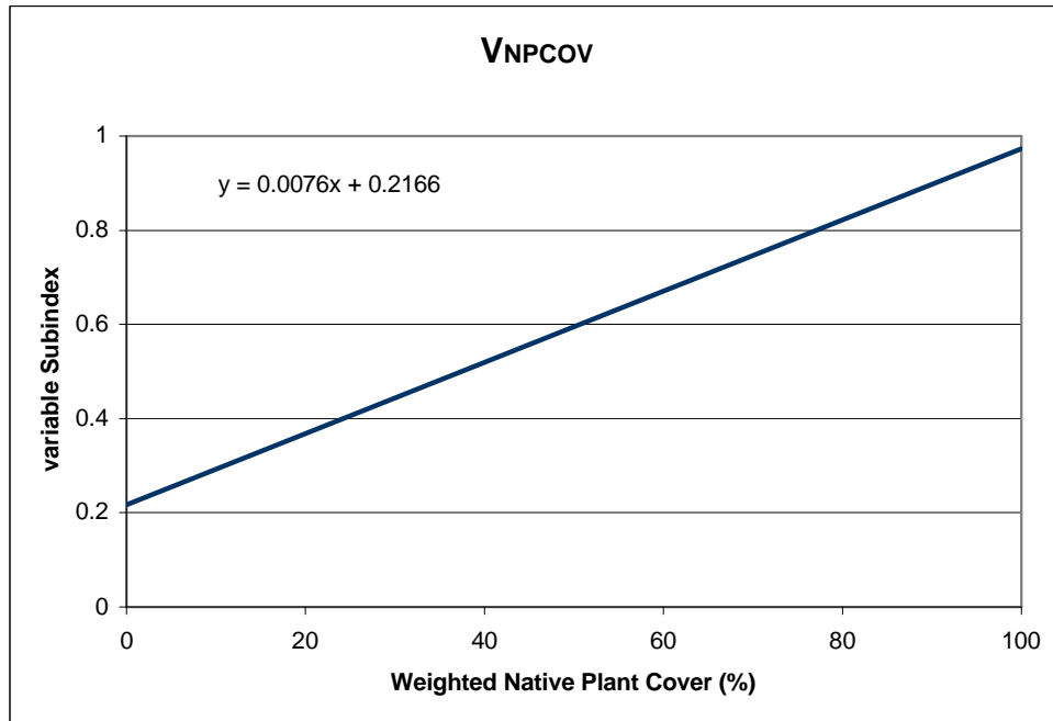
Figure 17. Correlation between percent Native Plant Cover and the Variable Subindex Score
