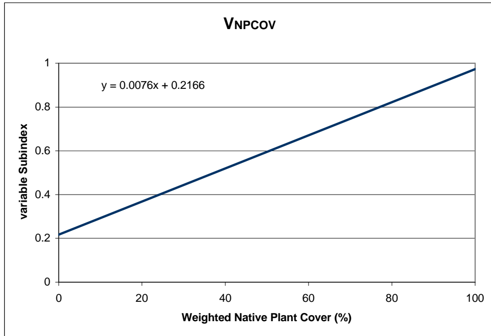
Figure 24. Correlation between Percent Native Plant Cover and the Variable Subindex Score
