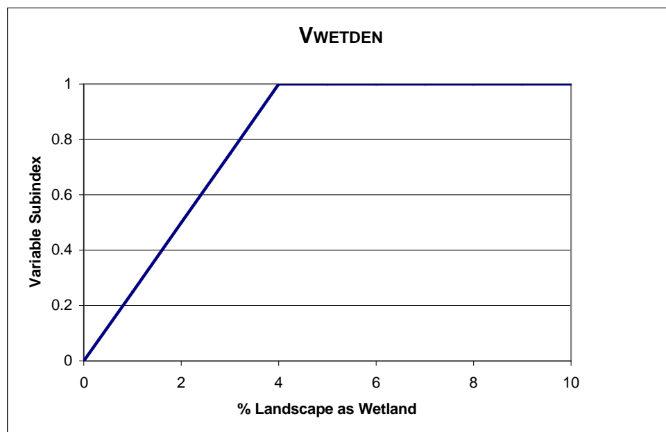
Figure 27. The relationship between the percentage of the landscape within an 800-m (0.5-mile) radius that is covered by wetland and the Variable Subindex Score
