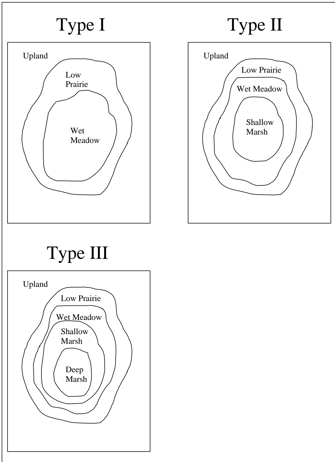
Figure 31. Wetland types and zonation of intermontane prairie potholes. Each zone expresses specific water regime, soil, and vegetation characteristics
