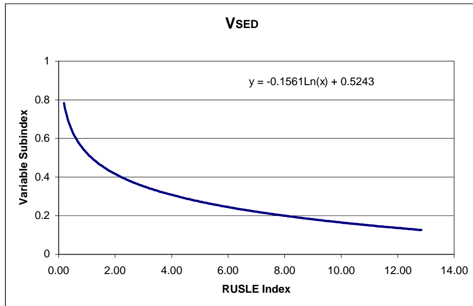
Figure 21. Relationship between RUSLE Index and the Variable Subindex Score
