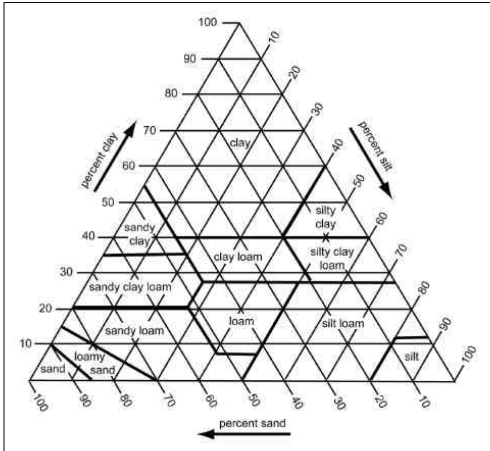
Figure 11. Chart showing the percentages of clay, silt, and sand in the basic soil textural classes and the corresponding soil textural names
