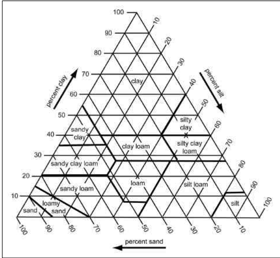
Figure 8. Chart showing the percentages of clay, silt, and sand in the basic soil textural classes and the corresponding soil textural name
