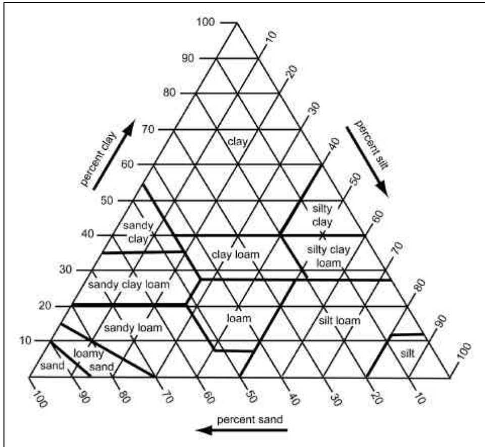
Figure 35. Chart showing the percentages of clay, silt, and sand in the basic soil textural classes
