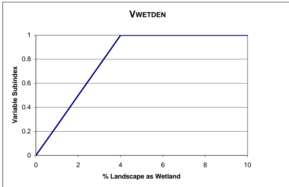
Figure B9. The relationship between the percentage of the landscape within an 800-m (0.5-mile) radius that is covered by wetland and the Variable Subindex Score
