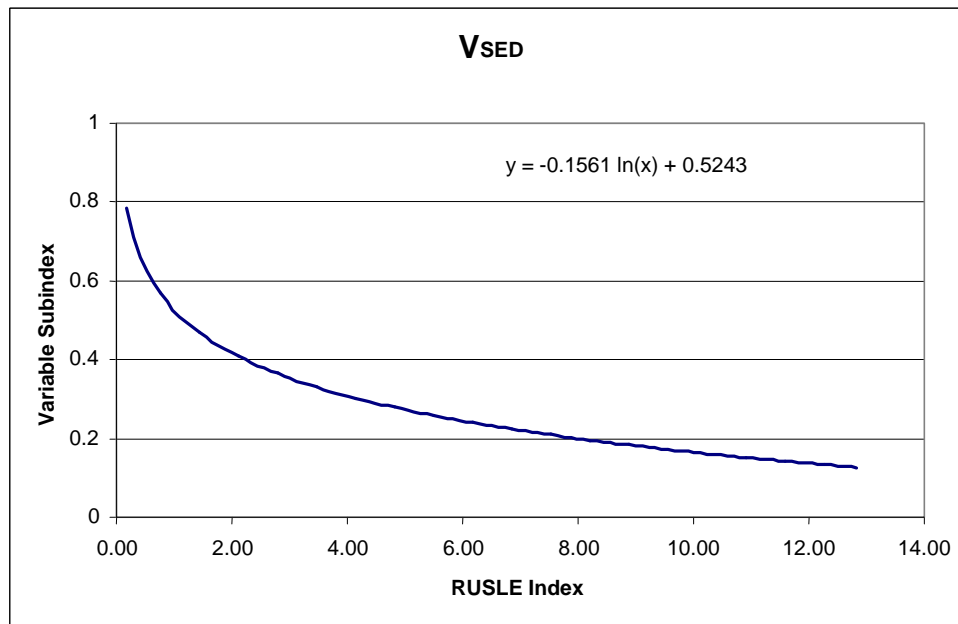
Figure B2. Relationship between RUSLE Index and the Variable Subindex Score
