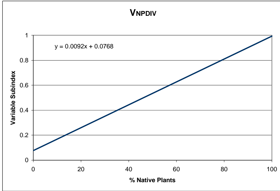
Figure B5. Correlation between Percent Native Plants and the Variable Subindex Scores
