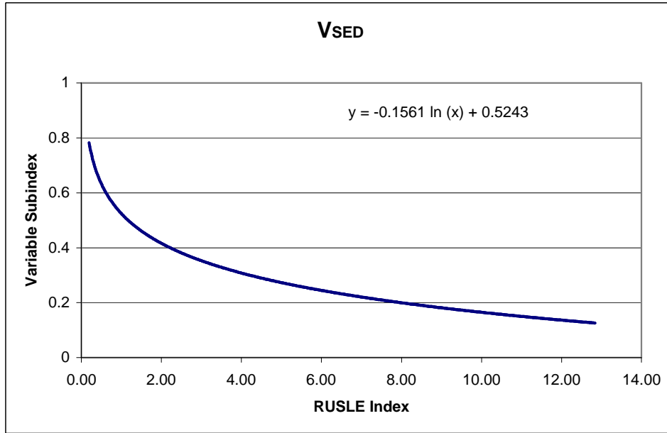
Figure 10. Relationship between RUSLE Index and Variable Subindex Score
