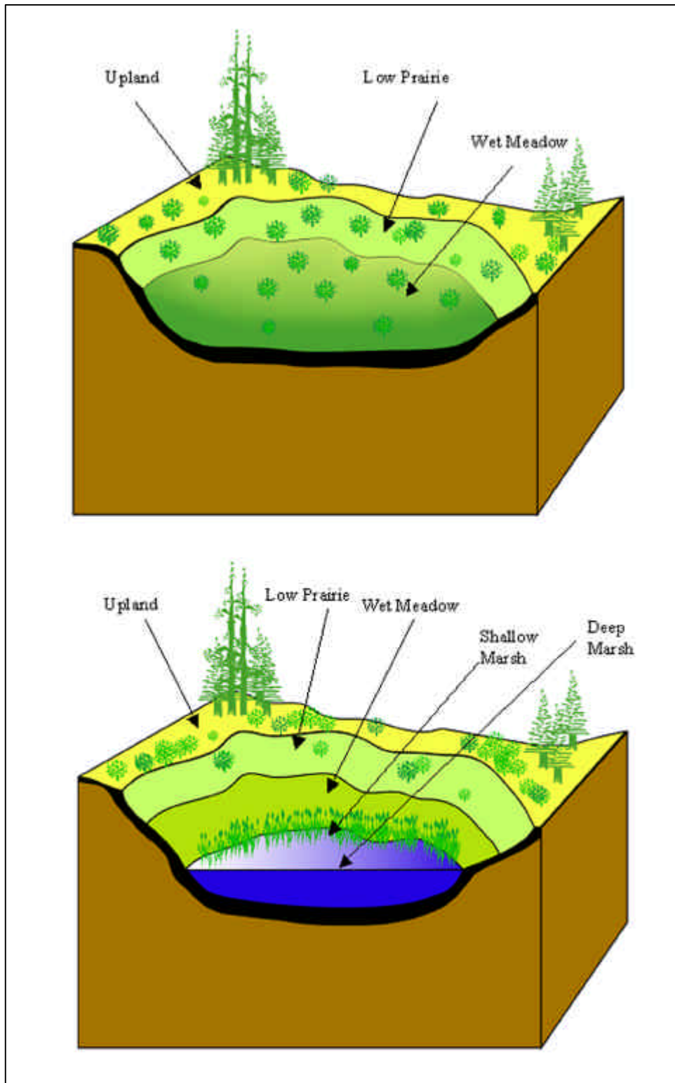
Figure 4. Two wetland types typical of the Intermontane Prairie Potholes. The upper panel shows a pothole wetland having only Low Prairie and Wet Meadow zones. The lower panel shows a pothole having Low Prairie, Wet Meadow, Shallow Marsh, and Deep Marsh zones
