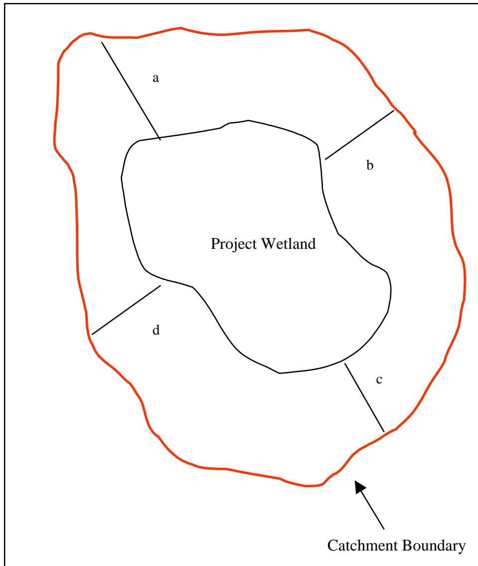
Figure 34. A wetland, its catchment boundary, and typical arrangement of four transects (a-d) for measuring catchment size and slope
