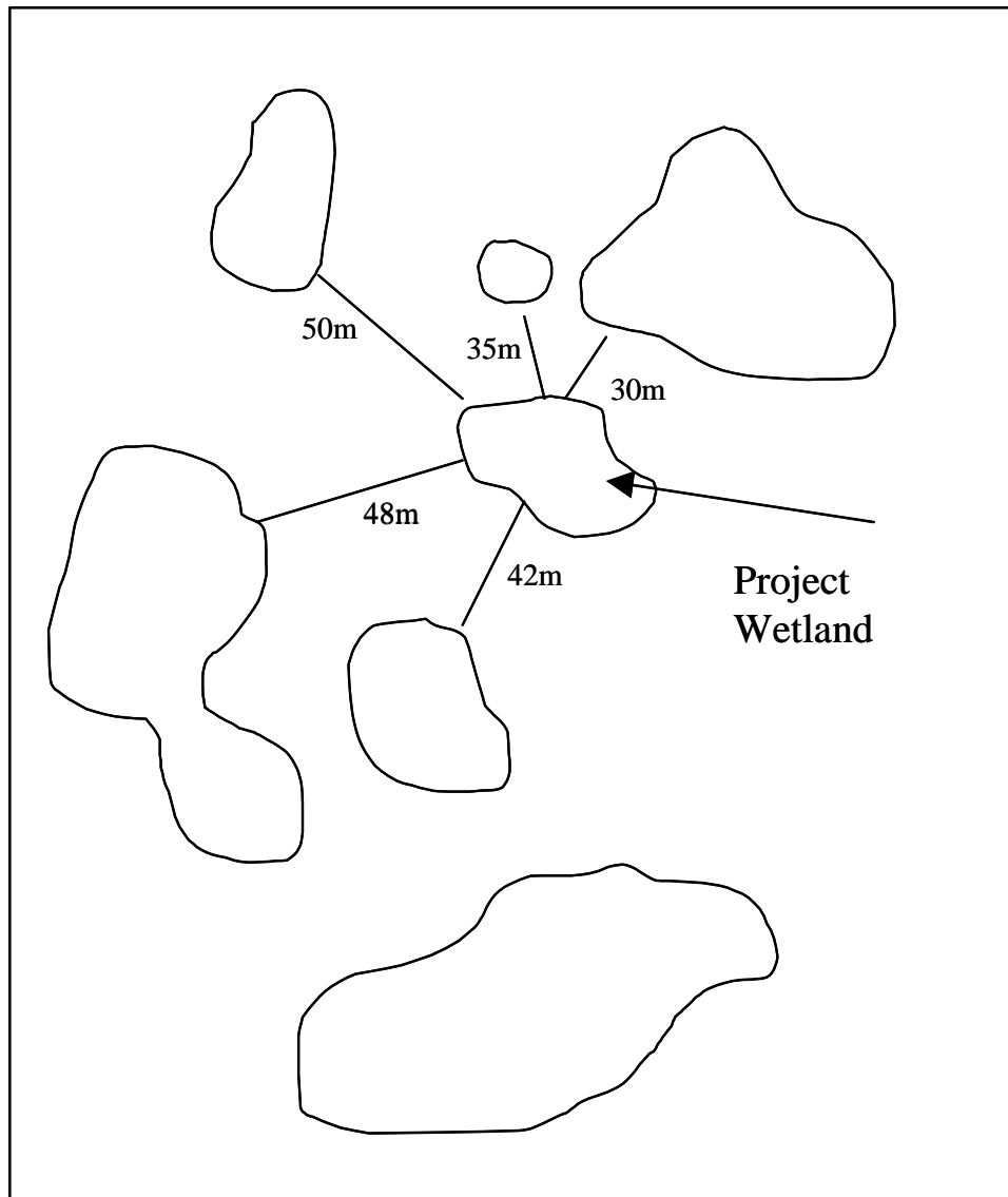
Figure 33. Measuring the five nearest neighbors to a project wetland. Measurements extend between upper Wet Meadow boundaries
