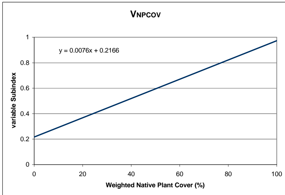
Figure B6. Correlation between percent Native Plant Cover and the Variable Subindex Score
