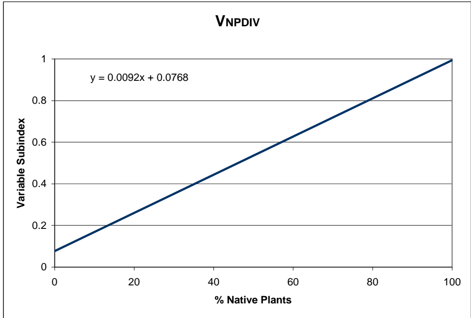
Figure 16. Correlation between Percent Native Plants and the Variable Subindex Score
