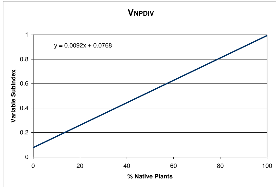
Figure 23. Correlation between Percent Native Plants and the Variable Subindex Score
