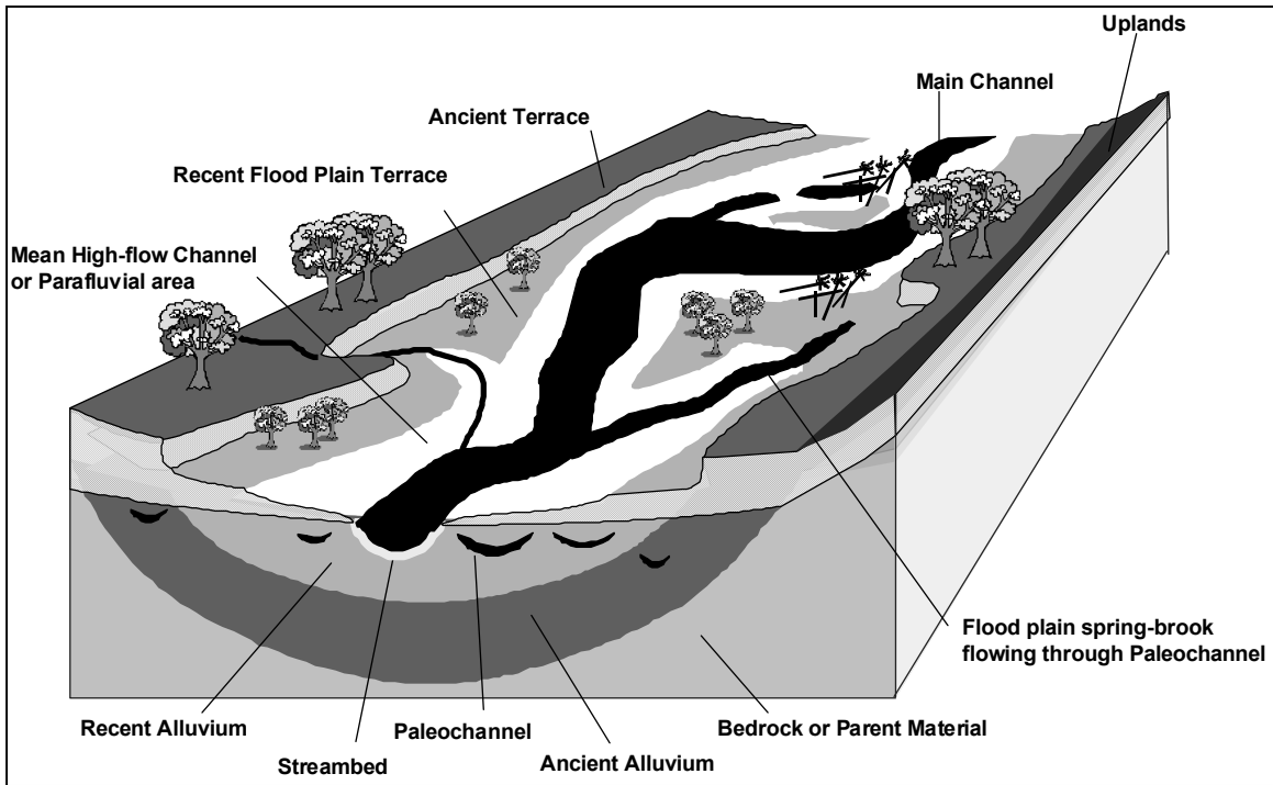
Figure 5. Schematic model of a floodplain in the reference domain of the northern Rocky Mountain ecoregion. (The model illustrates the extent of underground connectivity between the main channel and the subsurface and surface paleochannels.)
