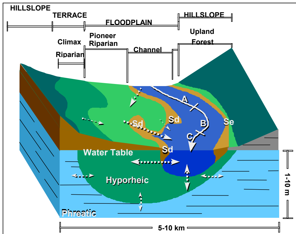
Figure 2. Three-dimensional illustration of groundwater-surface water interaction in gravel-bed rivers and the formation and development of the hyporheic zone (after Stanford and Ward 1988)
