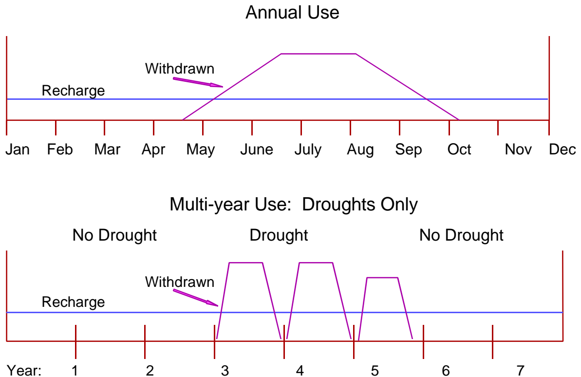
FIGURE 10. CONJUNCTIVE USE OF GROUNDWATER FOR DROUGHT
