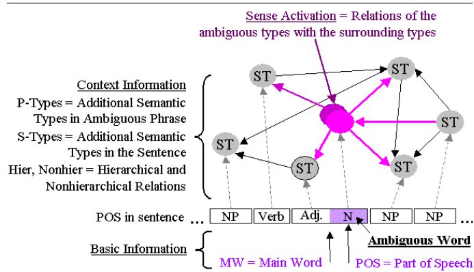
Figure 1 - Symbolic Knowledge Used (ST = Semantic Types)
