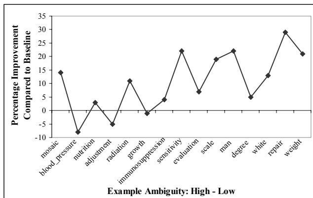
Figure 4 - Actual Accuracy Improvement (Ambiguity-Ordered)
