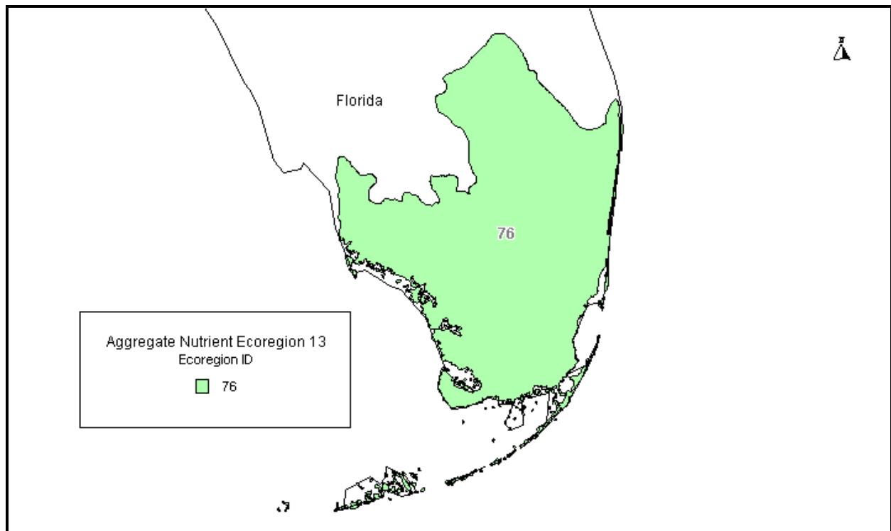
Figure 2. Ecoregion XIII with level III ecoregions shown
