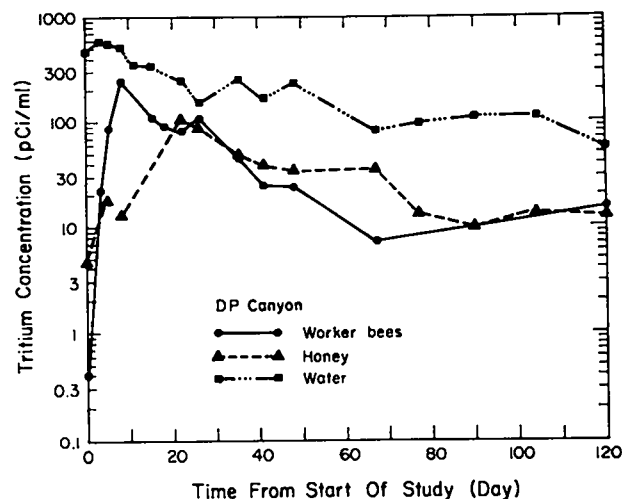
Fig. T-2. DP Canyon bee study.
