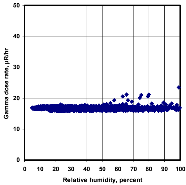
Relative humidity and gamma dose rate at NEWNET TA-54 Met Tower, Aug 2002
