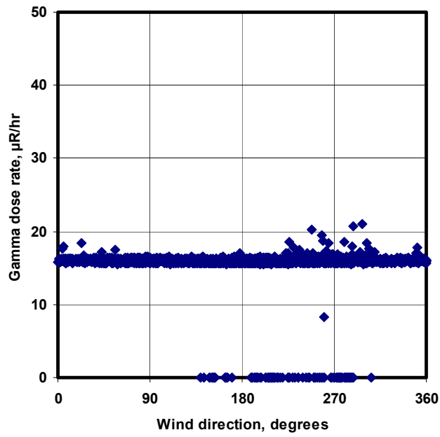
Wind direction and gamma dose rate at NEWNET DP West, Aug 2002
