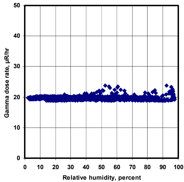
Relative humidity and gamma dose rate at NEWNET Area G South, Aug 2002
