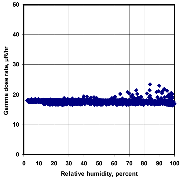
Relative humidity and gamma dose rate at NEWNET Buey East, Aug 2002
