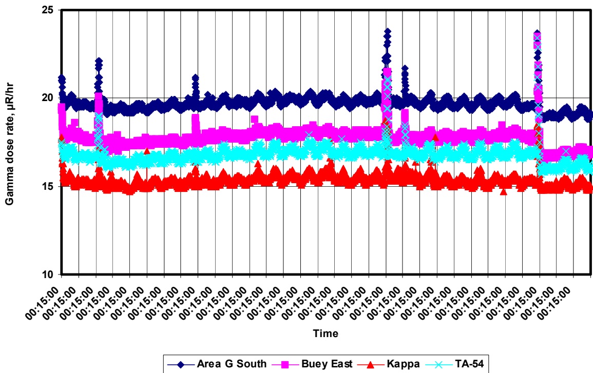
Figure 2. Gamma dose rates in August 2002 at NEWNET stations Area G South, Buey East, Kappa and TA 54
