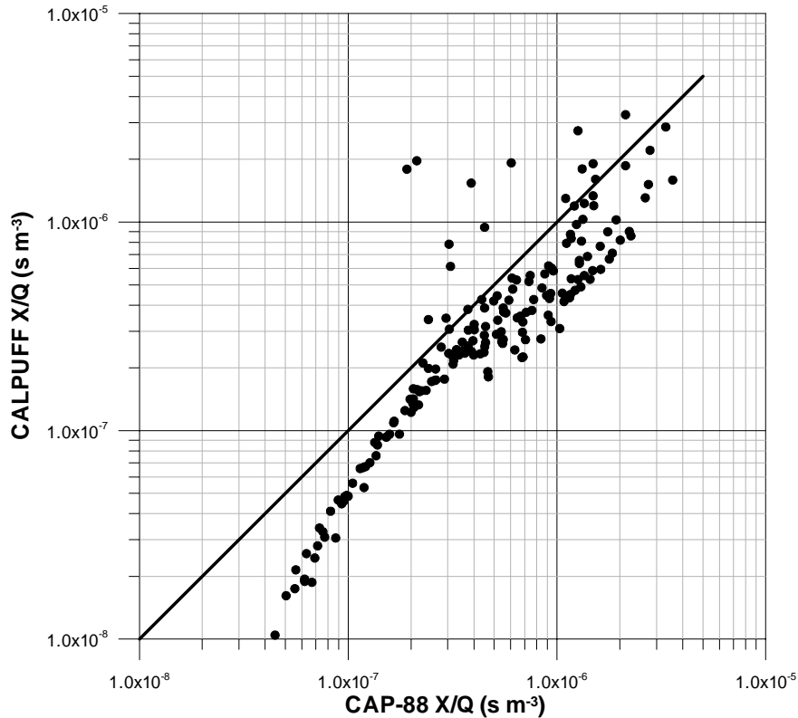
Figure 3. Annual average CAP-88 \chi/Q values versus CALPUFF annual average \chi/Q values for 1999 from a source located at Site D (Facility 3002919). Site D stack parameters are as follows: Stack height = 15.88 m, stack exit velocity = 25.9 m s -1 , stack diameter = 1.07 m, and stack exit temperature = 282 K.
