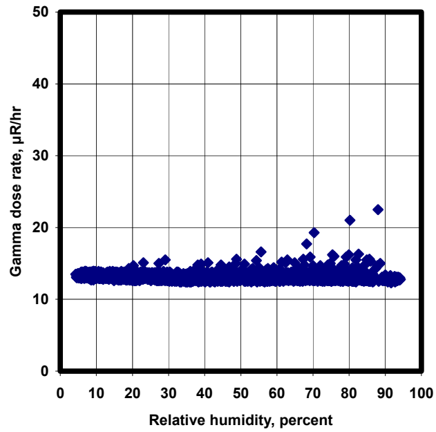
Relative humidity and gamma dose rate at NEWNET LAHS, Aug 2002
