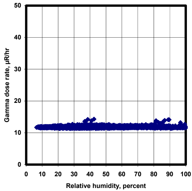
Relative humidity and gamma dose rate at NEWNET Ohkay Owingeh, Aug 2002
