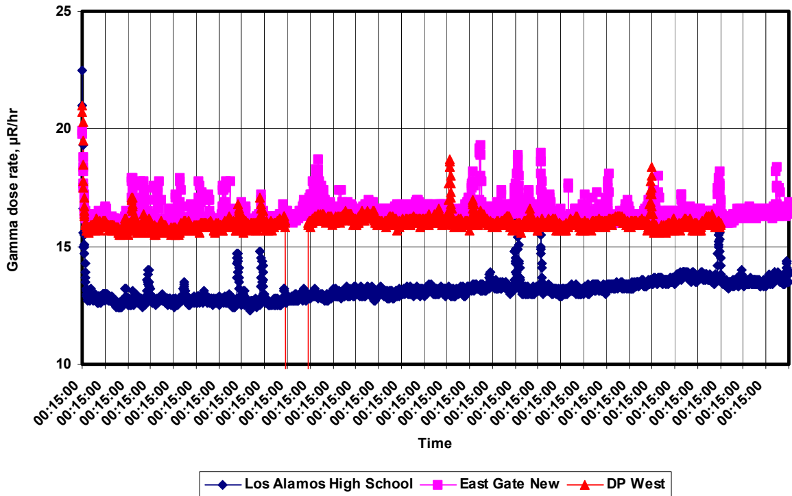
Figure 3. Gamma dose rates in August 2002 at NEWNET stations Los Alamos High School, East Gate New and DP West
