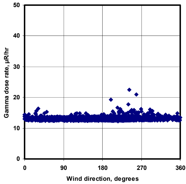
Wind direction and gamma dose rate at NEWNET LAHS, Aug 2002
