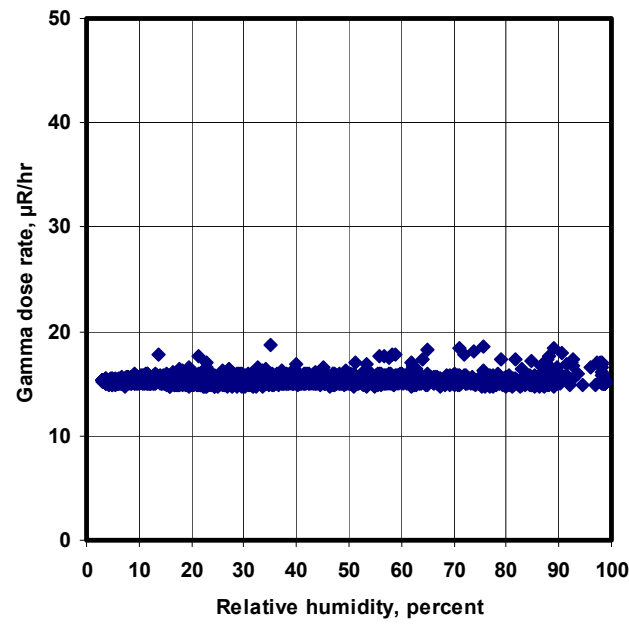
Relative humidity and gamma dose rate at NEWNET Kappa Site, Aug 2002
