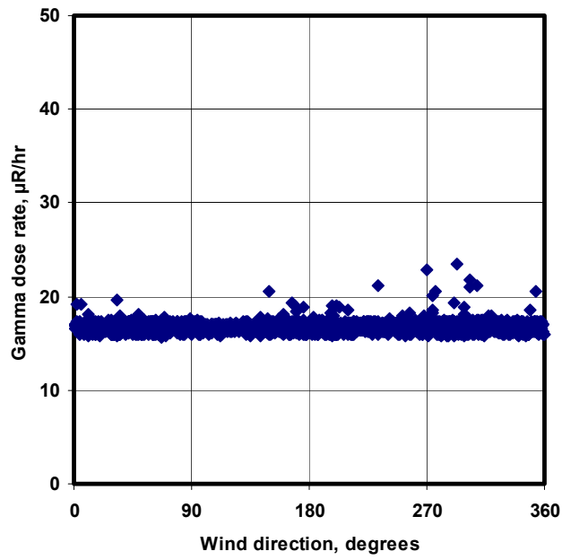
Wind direction and gamma dose rate at NEWNET TA-54 Met Tower, Aug 2002
