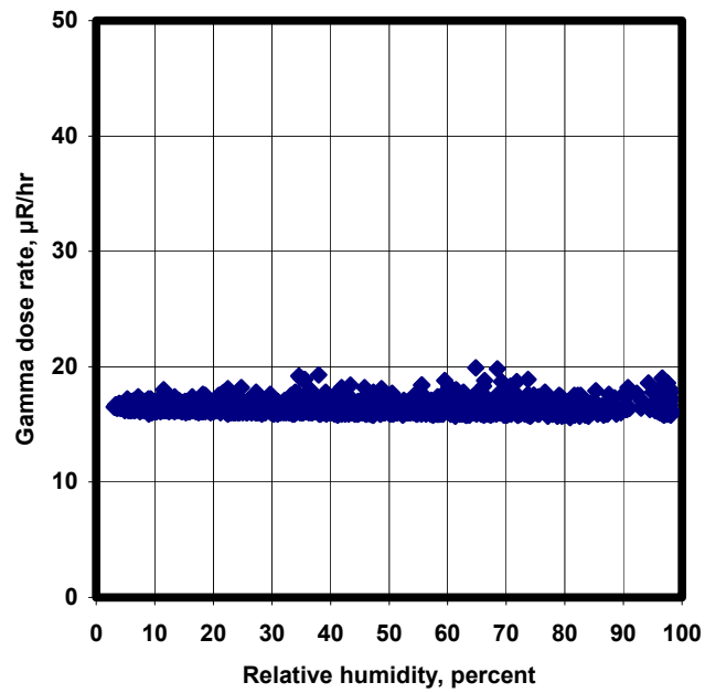
Relative humidity and gamma dose rate at NEWNET East Gate New, Aug 2002
