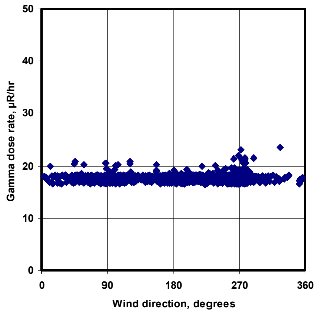
Wind direction and gamma dose rate at NEWNET Buey East, Aug 2002
