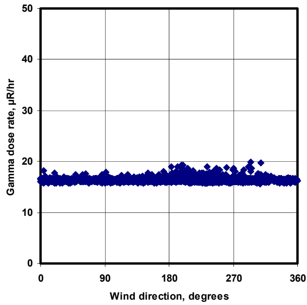
Wind direction and gamma dose rate at NEWNET East Gate New, Aug 2002
