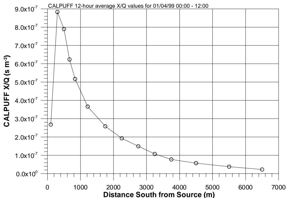
Figure 6. Twelve-hour average CALPUFF \chi/Q values as a function of distance south from the Site D stack.
