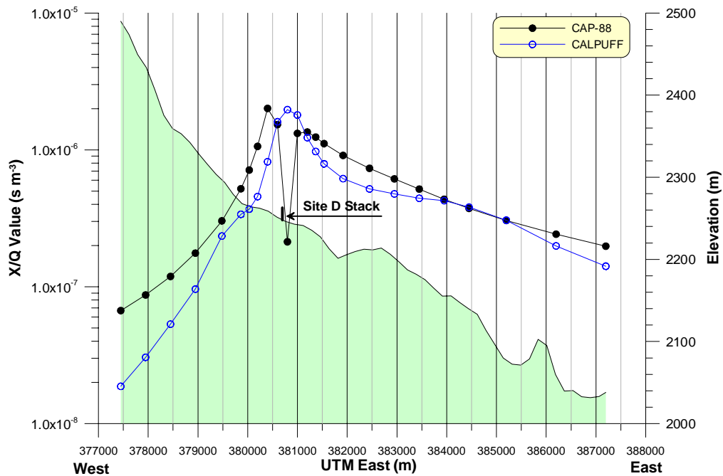
Figure 5. West-to-east cross section of terrain and annual average \chi/Q values for CALPUFF and CAP-88. Terrain is represented by the shaded area.
