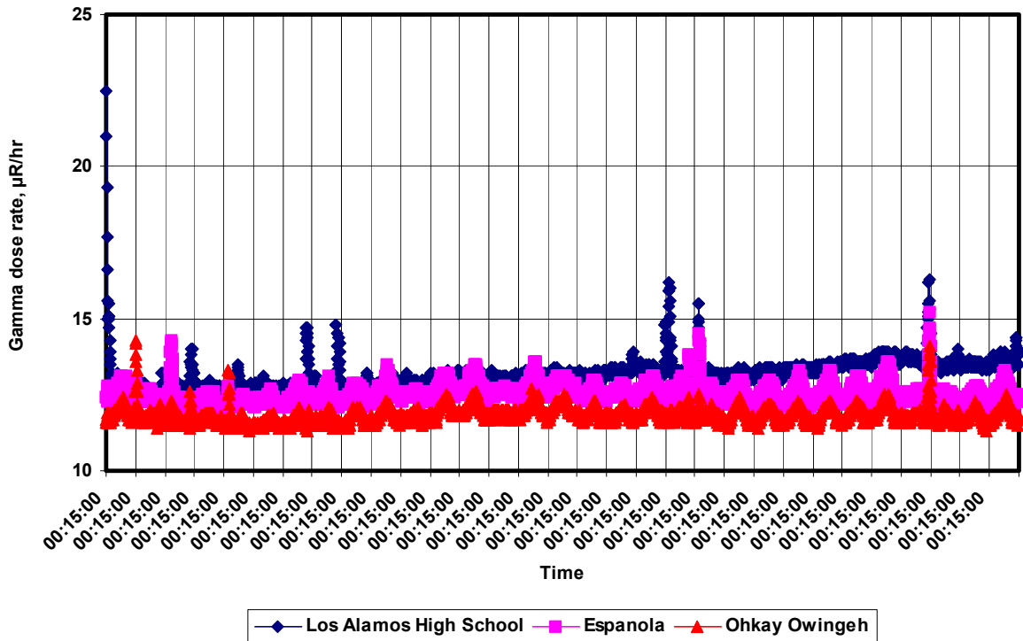
Figure 1. Gamma dose rates in August 2002 at NEWNET stations Los Alamos High School, Espanola, and Ohkay Owingeh
