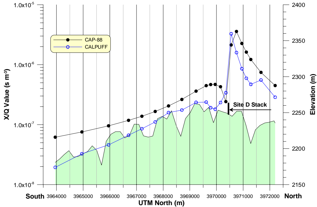
Figure 4. South-to-north cross section of terrain and annual average \chi/Q values for CALPUFF and CAP-88. Terrain is represented by the shaded area.
