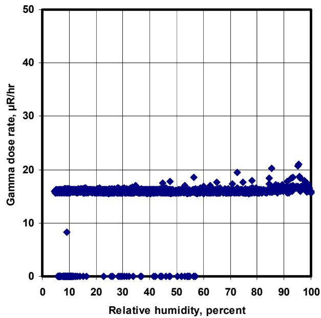
Relative humidity and gamma dose rate at NEWNET DP West, Aug 2002
