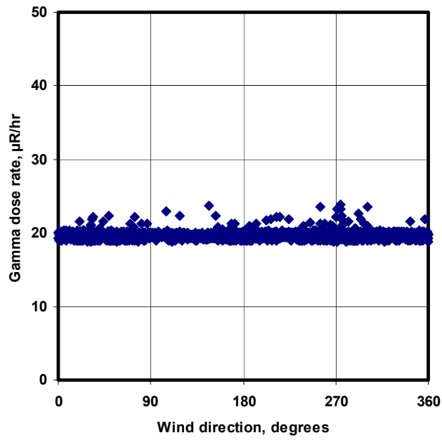
Wind direction and gamma dose rate at NEWNET Area G South, Aug 2002
