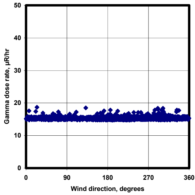
Wind direction and gamma dose rate at NEWNET Kappa Site, Aug 2002
