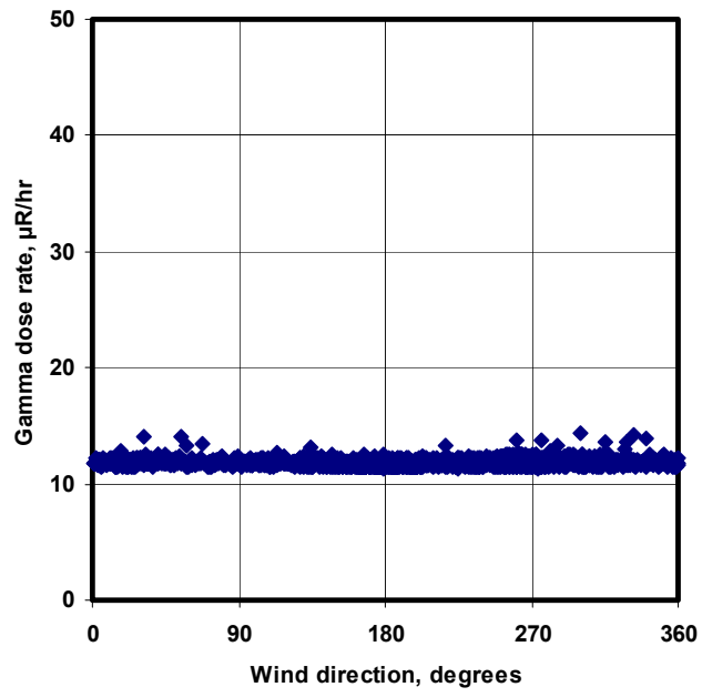
Wind direction and gamma dose rate at NEWNET Ohkay Owingeh, Aug 2002
