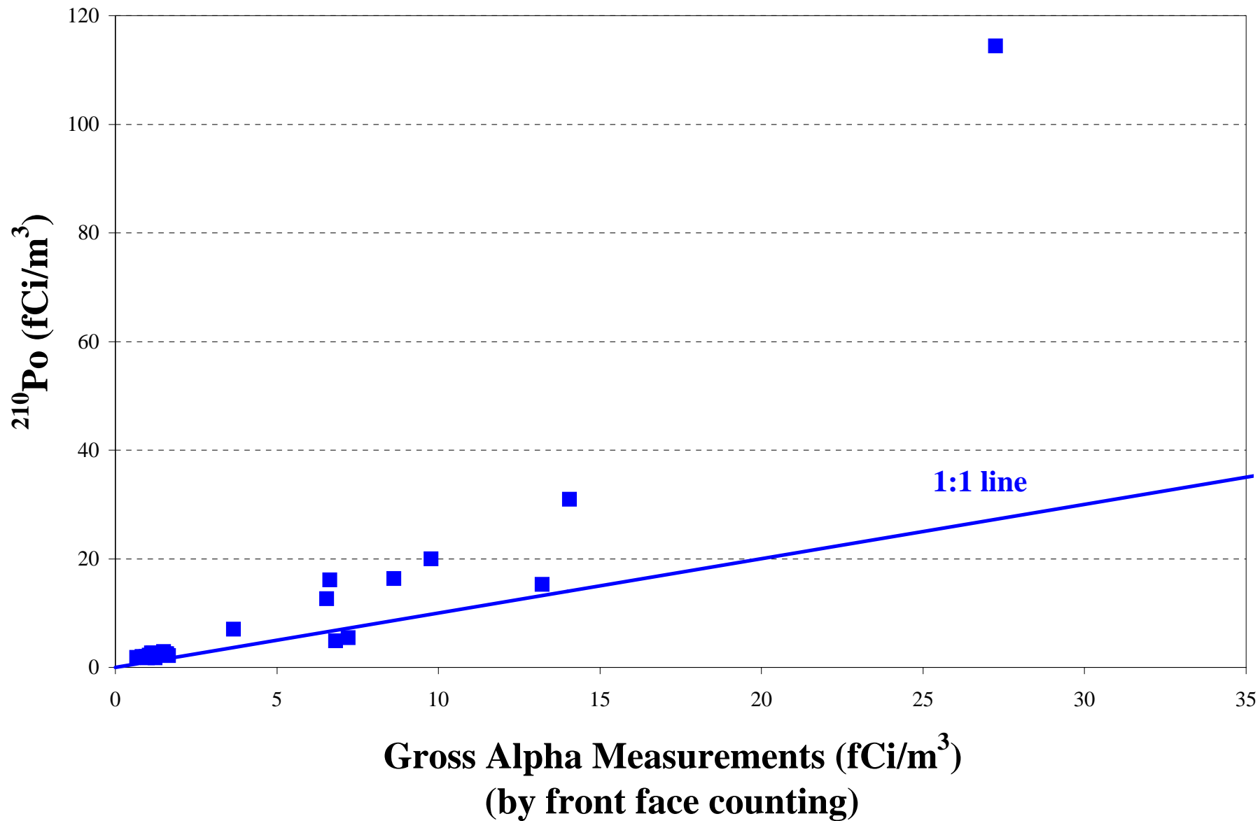
Figure 5. Gross Alpha Measurements versus Polonium-210 Measurements during the Cerro Grande Fire
