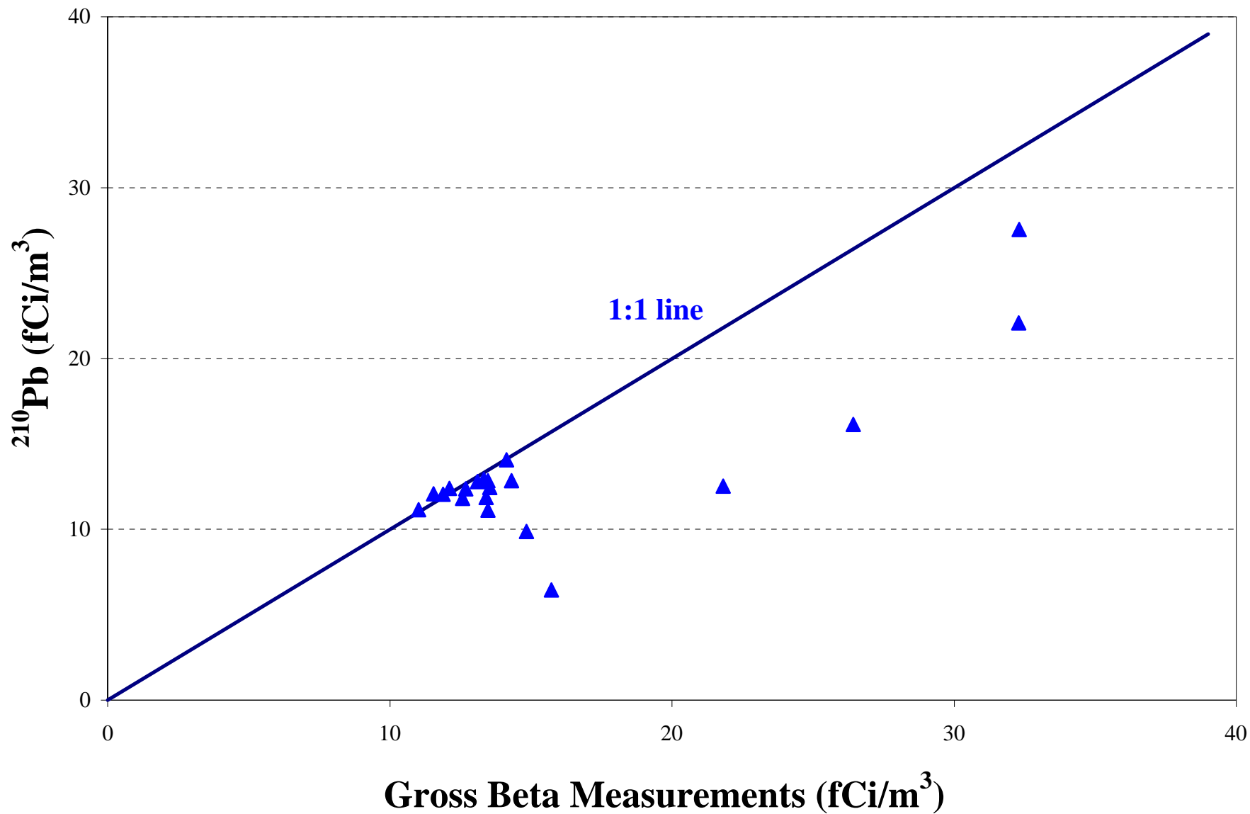
Figure 4. Gross Beta Measurements versus Lead-210 Measurements during the Cerro Grande Fire
