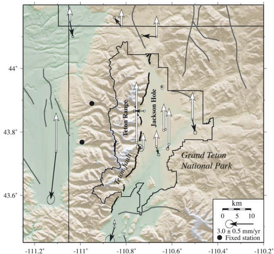
Figure 5. Horizontal (black) and vertical (white) velocities measured in the Teton fault network from 1987 to 2003. Two sites on the Teton mountain block were fixed to estimate velocities in a local reference frame. Error ellipses represent 1- \sigma uncertainties.
