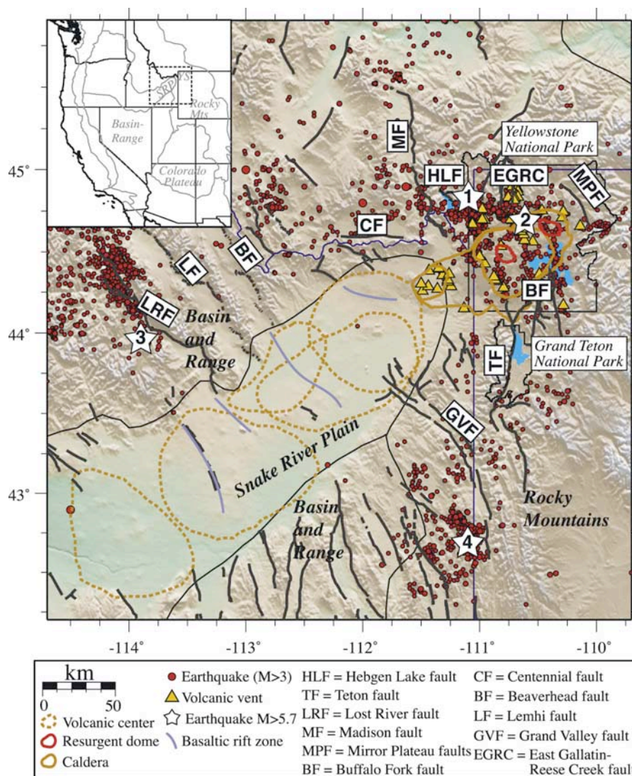
Figure 1. Index map of the Yellowstone–Snake River Plain magmatic-tectonic area showing earthquakes, Late Quaternary faults, and volcanic structures. Inset shows tectonic provinces of western United States and location of study area. Stars mark epicenters of significant historic earthquakes: (1) 1959 M7.5 Hebgen Lake, Montana, earthquake, (2) 1975 M6.1 Norris Junction, Wyoming, earthquake, (3) 1983 M7.3 Borah Peak, Idaho, earthquake, and (4) 1994 M5.9 Draney Peak, Idaho, earthquake. SRP rift zones associated with Holocene lava flows were obtained from Kuntz et al. [1986].
