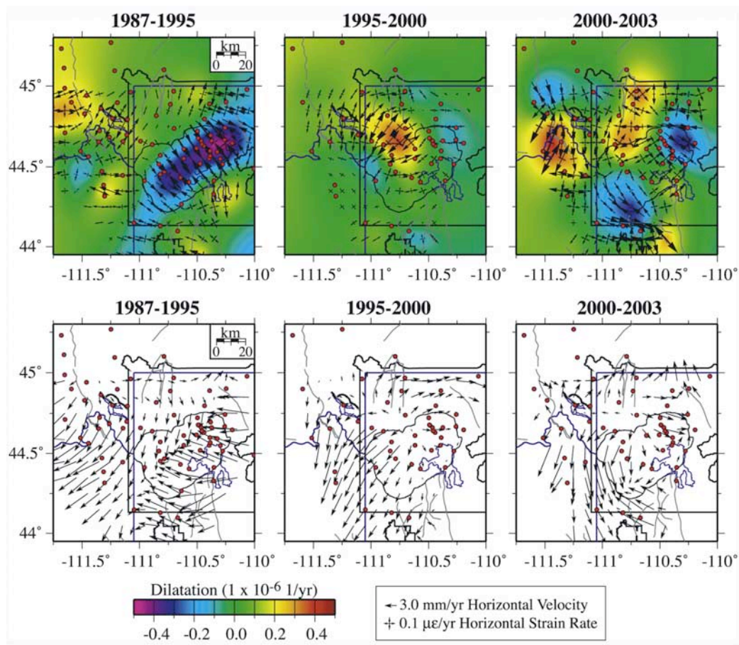
Figure 8. (top) Principal strain rates and (bottom) horizontal velocity fields for each of the three time windows of Figure 4. Strain rates are plotted as crosses and show direction of deformation. Dilatation rates representing fractional volume changes are shown as color contours in Figure 8 (top).
