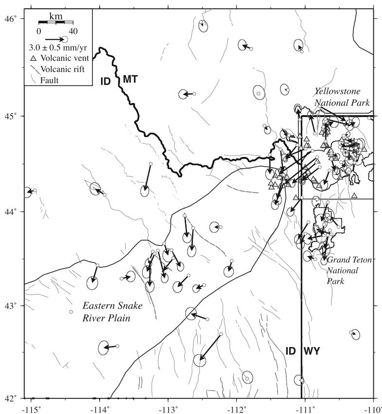
Figure 6. GPS-measured eastern Snake River Plain horizontal velocities for the time period 1995–2000. Error ellipses represent 1\text{-}\sigma uncertainties.
