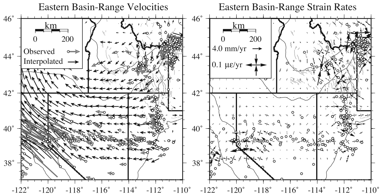
Figure 9. (left) Horizontal velocity field and (right) principal strain rates for the eastern Basin and Range province and the YSRP determined by GPS measurements.
