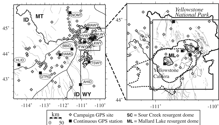
Figure 2. Map of campaign and continuous GPS stations in the YSRP used in this study. Continuous stations labeled separately. (left) Regional GPS network and (right) the Yellowstone National Park GPS network.
