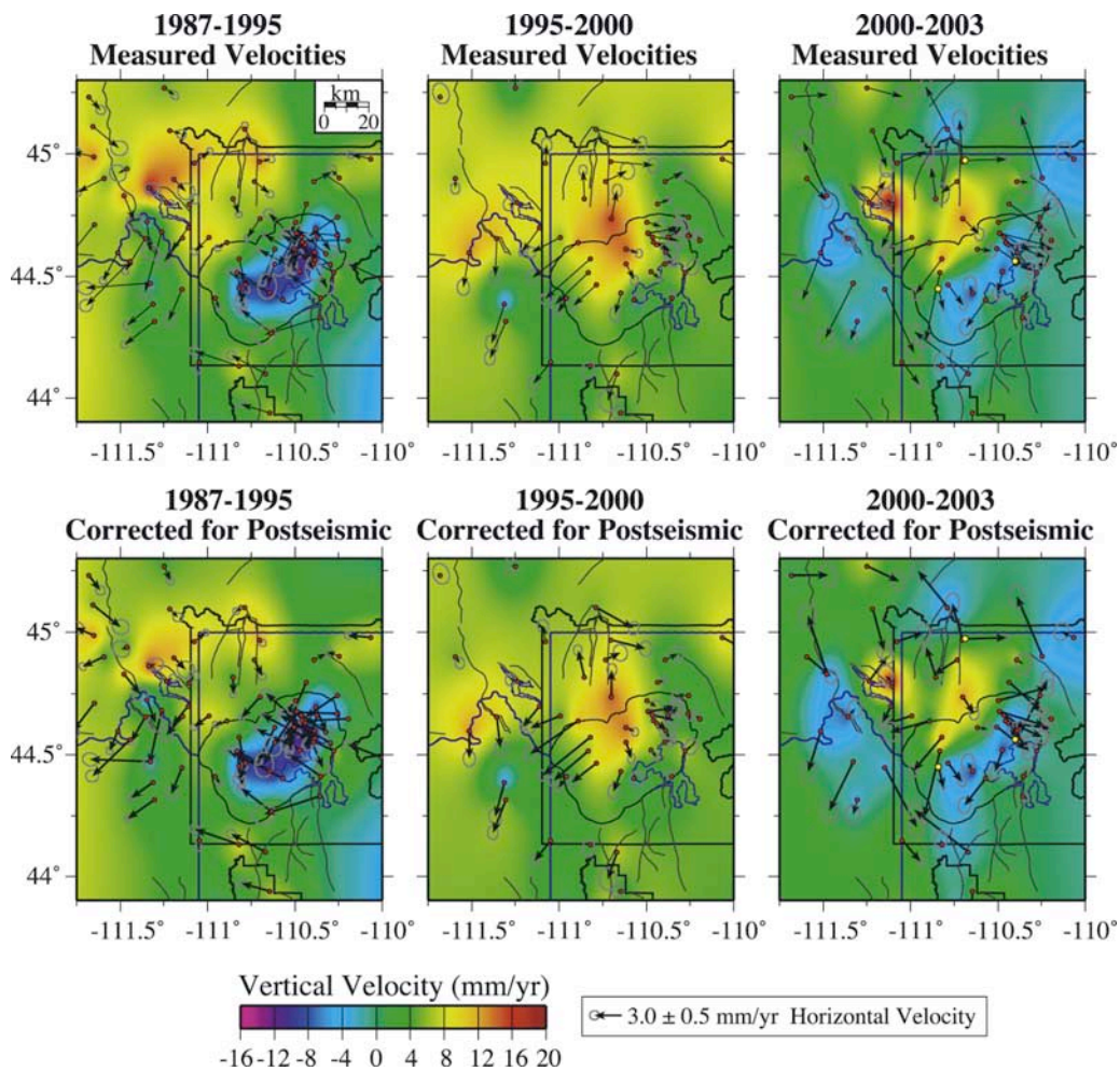
Figure 4. GPS-measured horizontal and vertical velocities of the Yellowstone Plateau at different time windows of 1987–1995, 1995–2000, and 2000–2003. Vectors represent horizontal velocities, and color contours represent vertical velocities. Error ellipses represent 1- \sigma uncertainties. (top) Observed velocities and (bottom) velocities corrected for viscoelastic relaxation.
