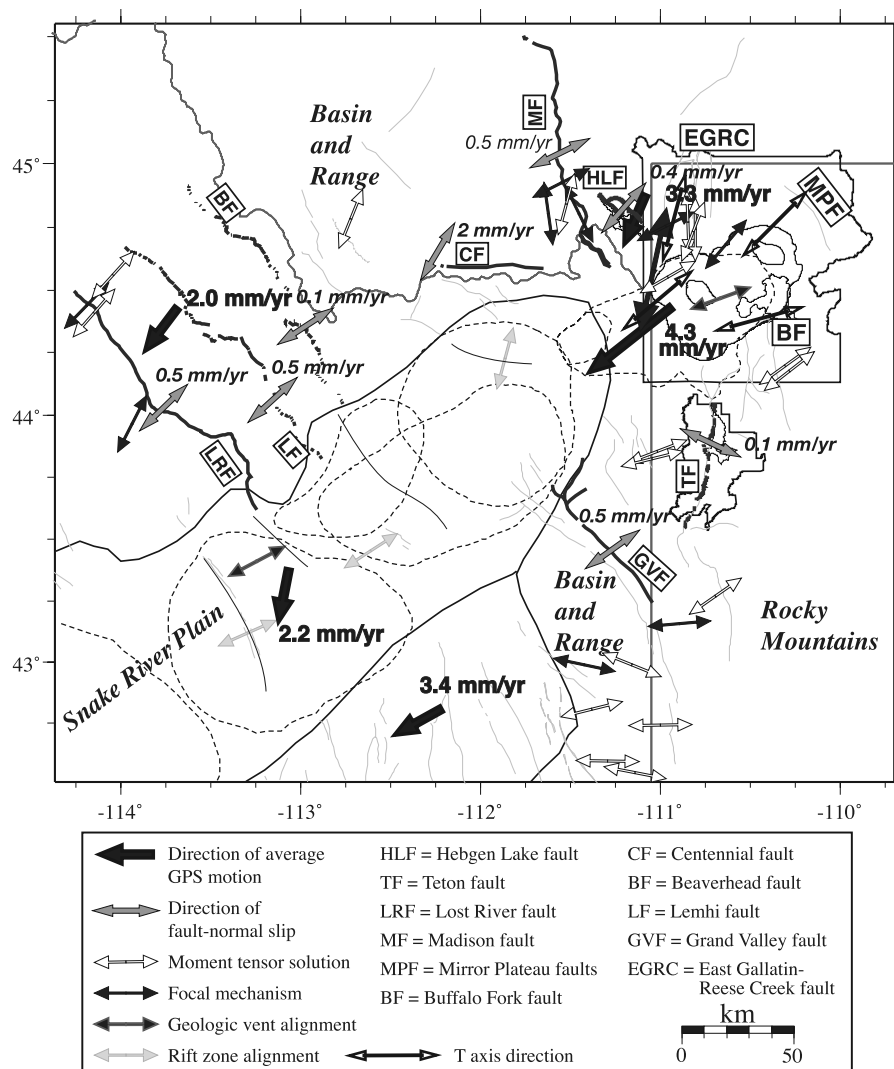
Figure 12. Summary map of GPS-measured deformation vectors derived from this study for the YSRP. Average GPS rates are labeled in large font. Fault slip rates from Byrd et al. [1994], Haller et al. [2002], and Wong et al. [2000] were converted to horizontal extension rates assuming a fault dip of 60^\circ and are labeled in small fonts. For comparison, minimum principal stress indicators from other studies are also shown. T axis directions are from Waite [1999], focal mechanisms and vent alignments are from Zoback [1992], moment tensor solutions are from http://quakes.oce.orst.edu/moment-tensor , and mapped rift zones are from Smith et al. [1996].
