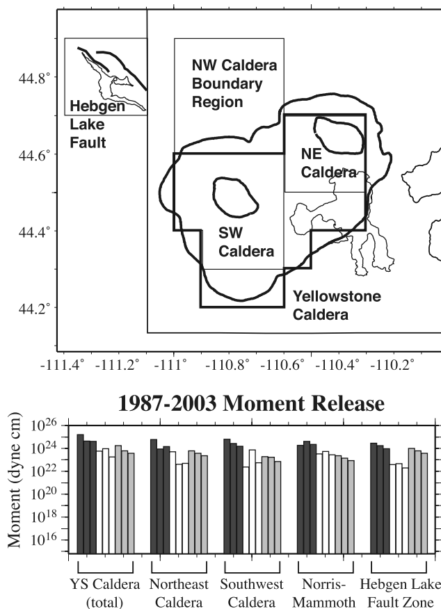
Figure 10. (bottom) Histogram of geodetic (dark gray), seismic (white), and geologic (light gray) moments for different regions in the Yellowstone Plateau. The three bars for each moment type represent the three time windows of 1987–1995, 1995–2000, and 2000–2003. (top) Map showing different regions of the plateau, with the caldera area outlined in bold.
