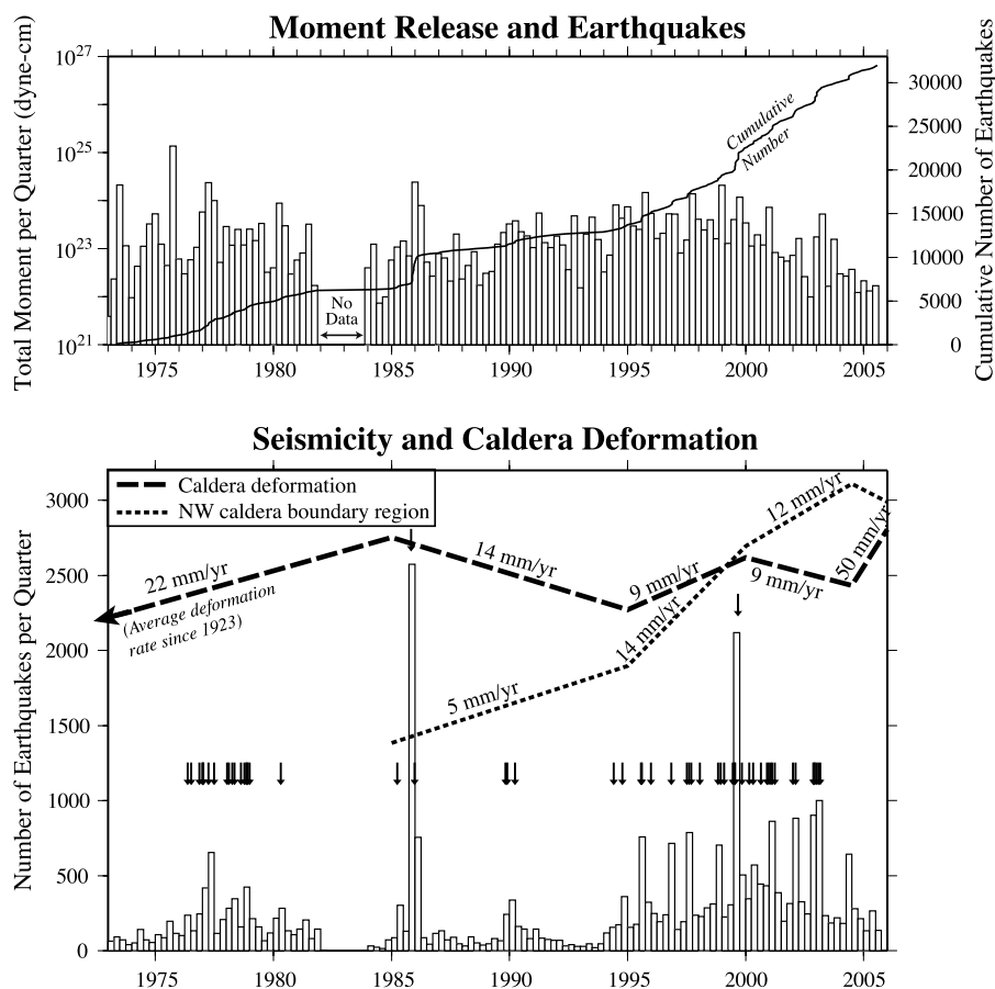
Figure 11. Plot of Yellowstone Plateau seismicity, deformation, and moment release. (top) Histogram showing the moment release per quarter and the cumulative number of earthquakes. (bottom) Histogram showing number of earthquakes per quarter and trends in caldera deformation from leveling and GPS campaigns. Earthquake swarms are marked by arrows.
