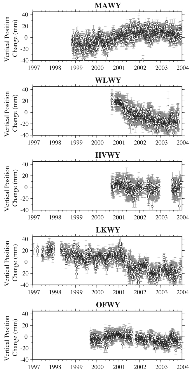
Figure 7. Time series of vertical components of continuous GPS stations in the Yellowstone Plateau. Increasing displacements over time indicate uplift; decreasing displacements indicate subsidence. Error bars are obtained from weighted RMS of daily solutions.
