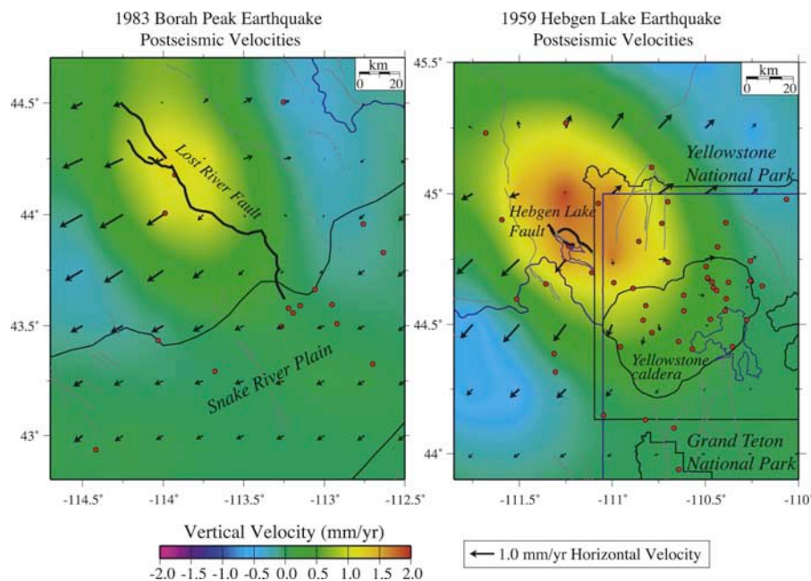
Figure 3. Velocity fields determined from modeling of viscoelastic relaxation following the 1959 M7.5 Hebgen Lake and 1983 M7.3 Borah Peak earthquakes. Vectors represent horizontal velocities, and color contours represent vertical velocities.
