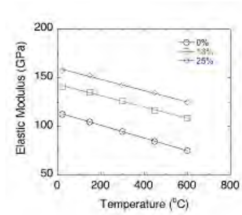
Fig. 3-16. Effect of temperature and concentration of TiC particulates on the elastic properties of titanium-matrix composites.
