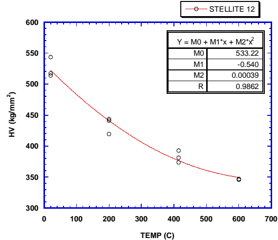
Fig. 2-4. High-temperature hardness tester vacuum chamber and lifting apparatus (left); effects of temperature on the Vickers microindentation hardness of Stellite 12 (right).
