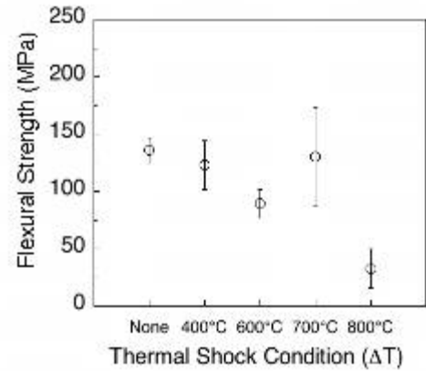
Fig. 3-14. Thermal shock resistance of polymer-derived SiCN ceramic.
