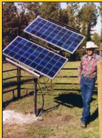
Solar pumping replaced a gas-powered generator on the Tomlinson Ranch near Gold Creek, MT.
