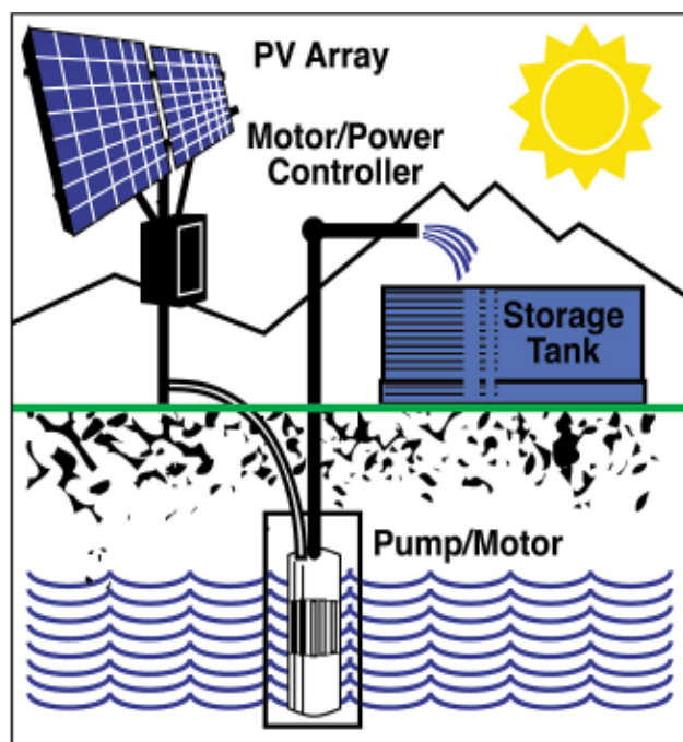
A typical solar-powered stock watering system includes a solar array, pump, storage tank and controller.
