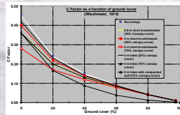
Figure 2. Pre-fire cover Management Factor estimates for Enhanced USLE Approach
