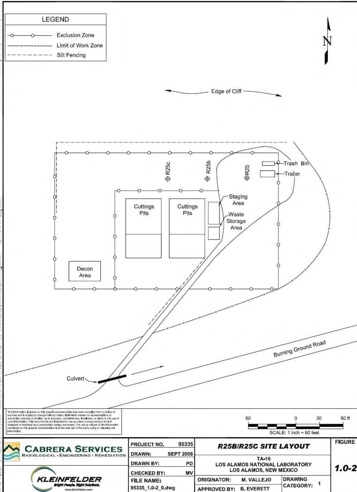
Figure 1.0-2 Site layout
