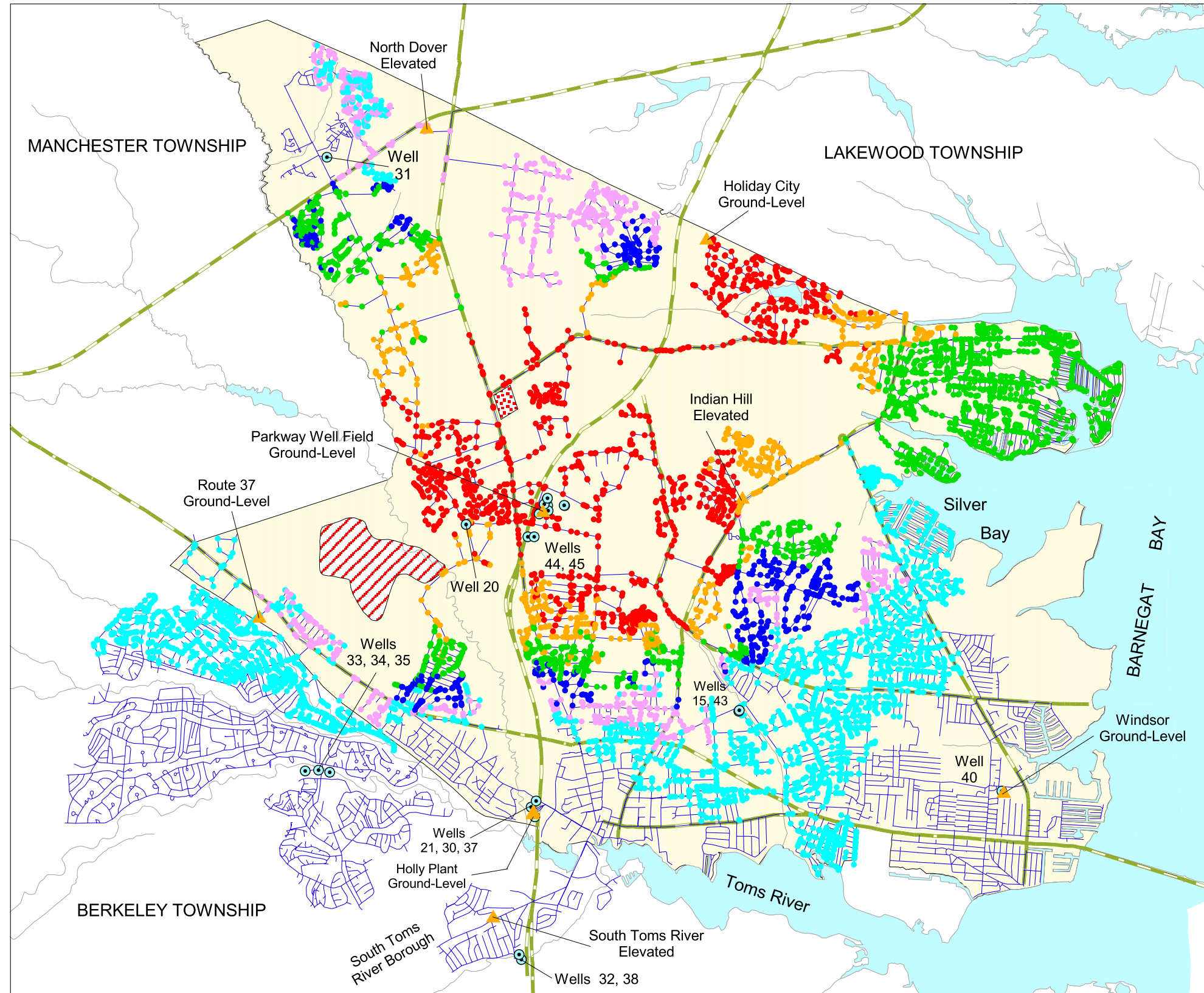
PLATE 20. AREAL DISTRIBUTION OF SIMULATED PROPORTIONATE CONTRIBUTION OF WATER FROM THE PARKWAY WELL FIELD GROUND-LEVEL STORAGE TANK TO LOCATIONS IN THE DOVER TOWNSHIP AREA, NEW JERSEY AUGUST 1998 CONDITIONS By Morris L. Maslia, Jason B. Sautner, and Mustafa M. Aral
