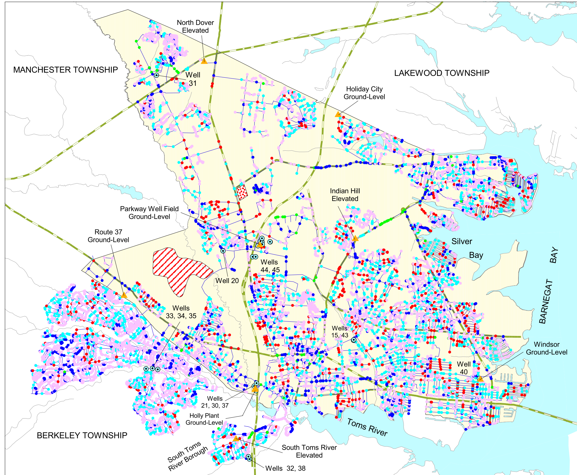
PLATE 7. DISTRIBUTION OF NODAL VALUES OF AVERAGE CONSUMPTION USED TO MODEL THE 1998 WATER-DISTRIBUTION SYSTEM SERVING THE DOVER TOWNSHIP AREA, NEW JERSEY
