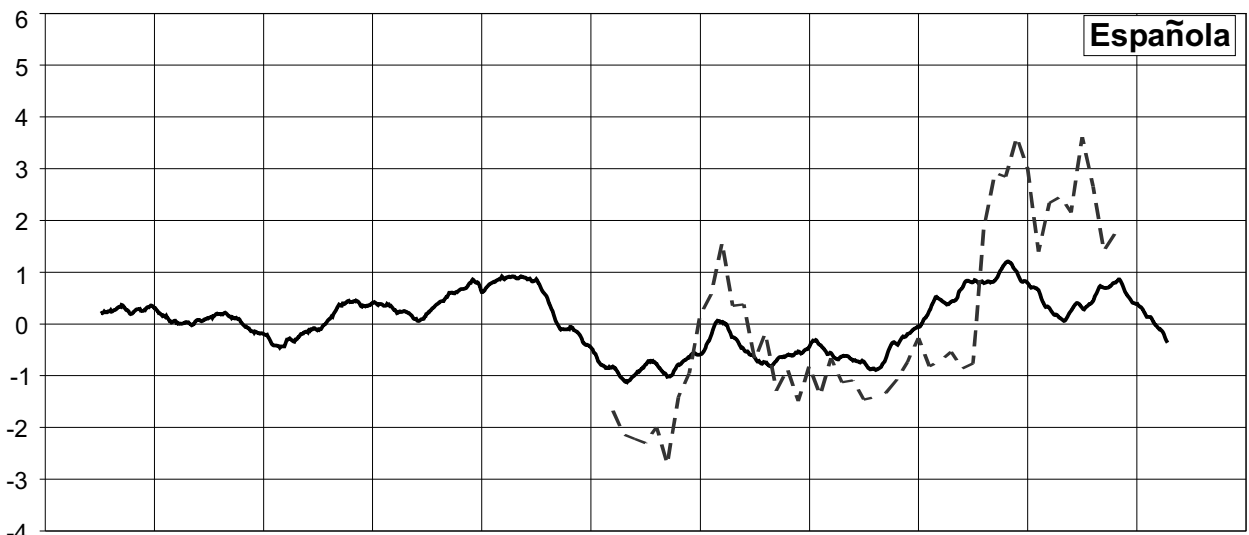
JEMEZ Y SANGRE REGIONAL WATER PLAN Normalized Annual Precipitation for Selected Precipitation Stations and the Pacific Decadal Oscillation (PDO) Index
