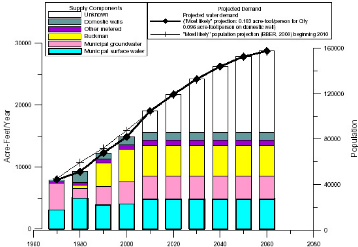
JEMEZ Y SANGRE REGIONAL WATER PLAN Domestic and Municipal Water Demand in the Santa Fe River Sub-Basin
