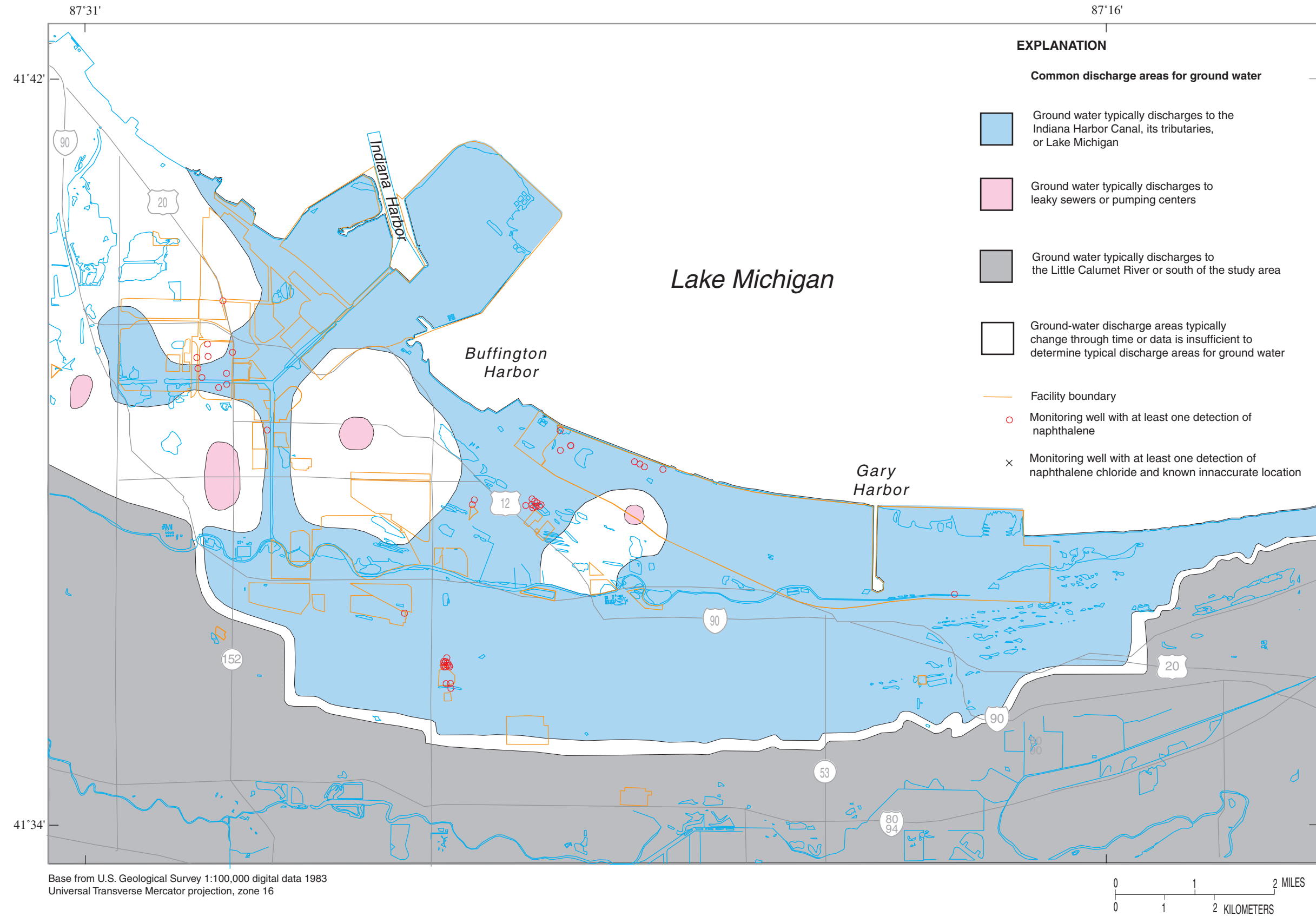
Figure 34. Common discharge areas for ground water in the Calumet aquifer and monitoring wells with at least one detection of naphthalene in the study area, northwestern Indiana.
