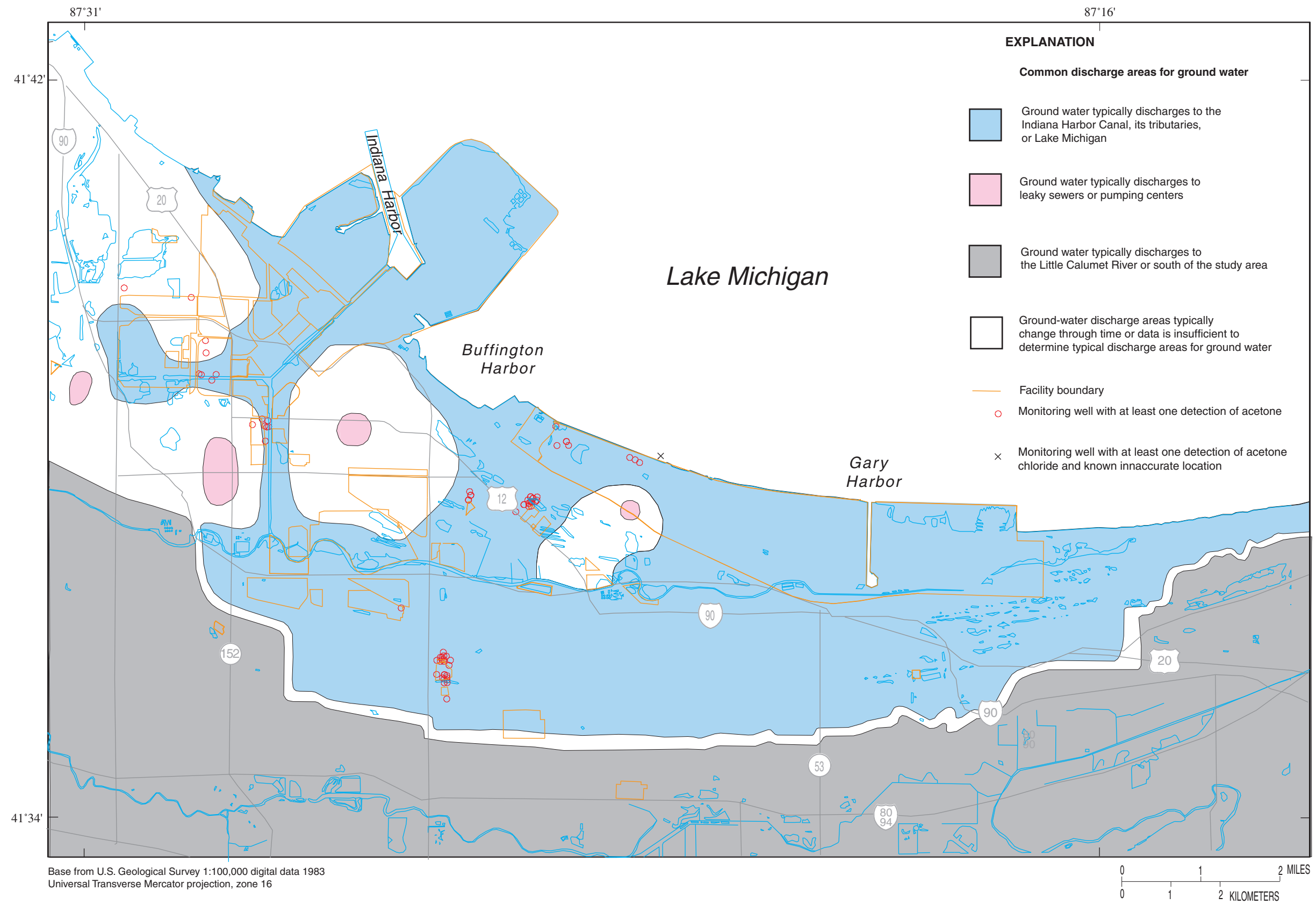
Figure 33. Common discharge areas for ground water in the Calumet aquifer and monitoring wells with at least one detection of acetone in the study area, northwestern Indiana.
