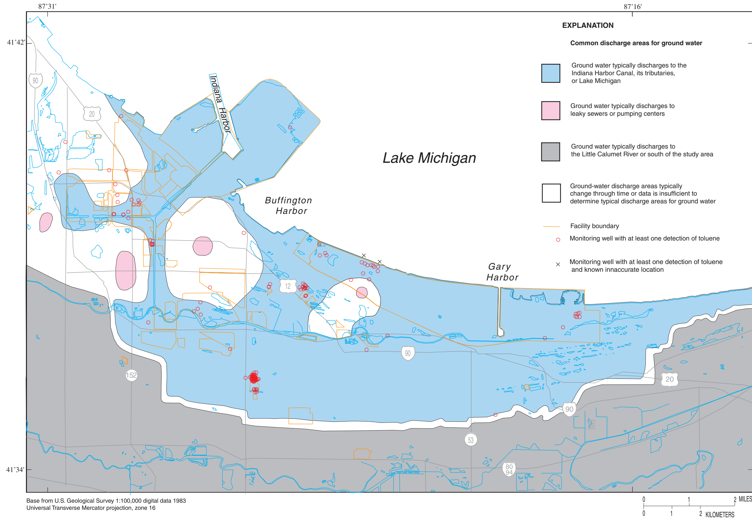
Figure 29. Common discharge areas for ground water in the Calumet aquifer and monitoring wells with at least one detection of toluene in the study area, northwestern Indiana.
