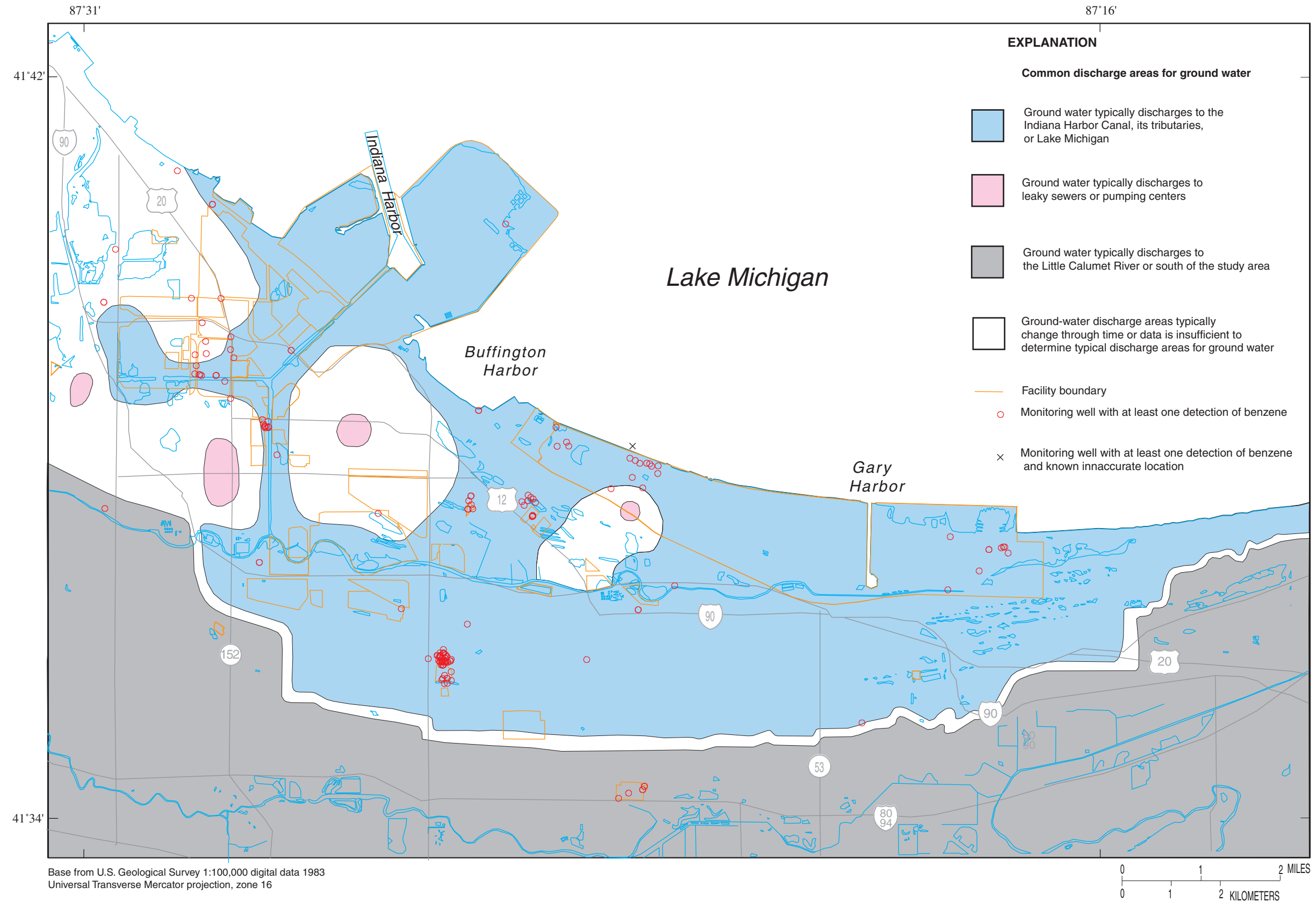
Figure 28. Common discharge areas for ground water in the Calumet aquifer and monitoring wells with at least one detection of benzene in the study area, northwestern Indiana.
