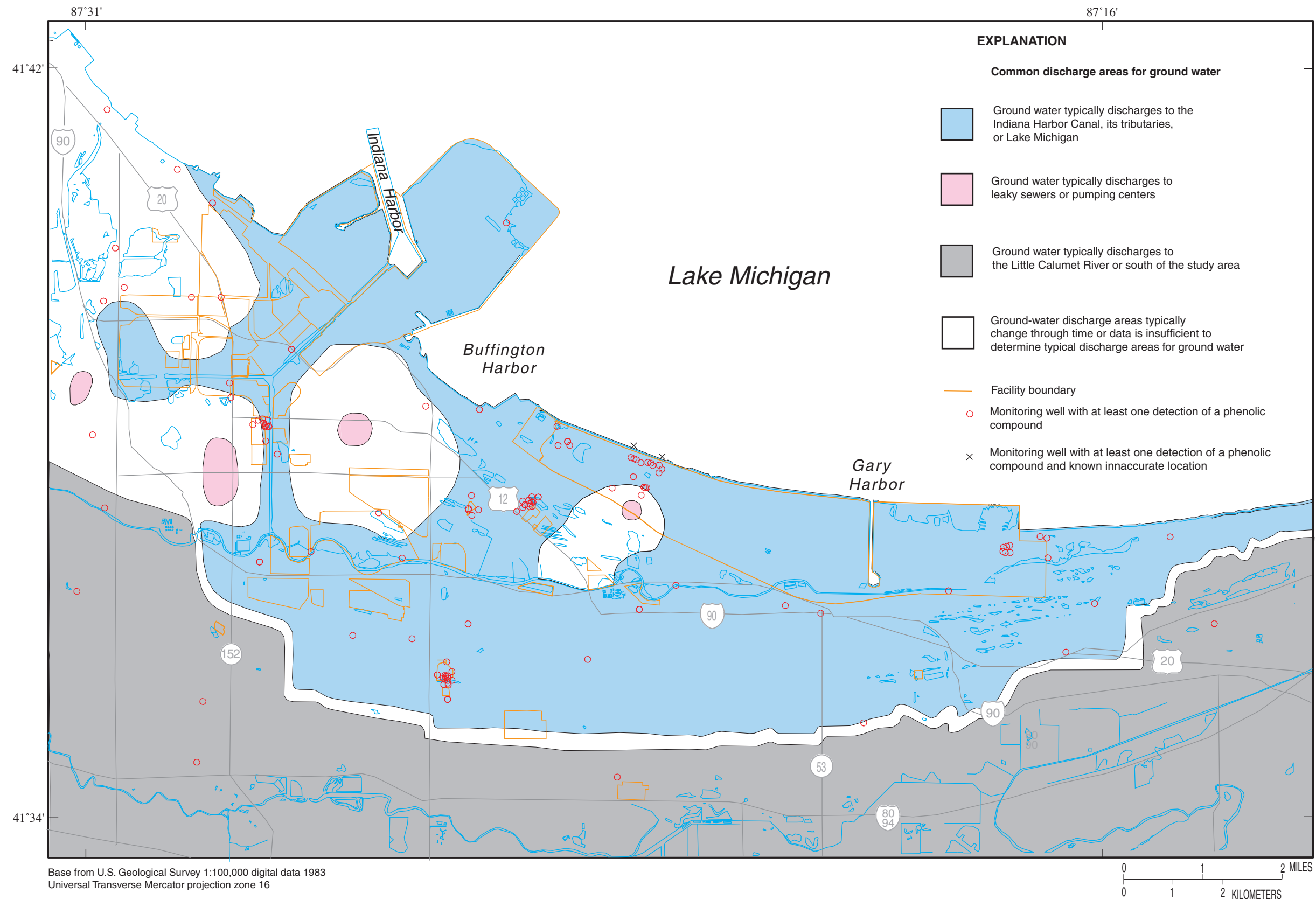
Figure 27. Common discharge areas for ground water in the Calumet aquifer and monitoring wells with at least one detection of a phenolic compound in the study area, northwestern Indiana.
