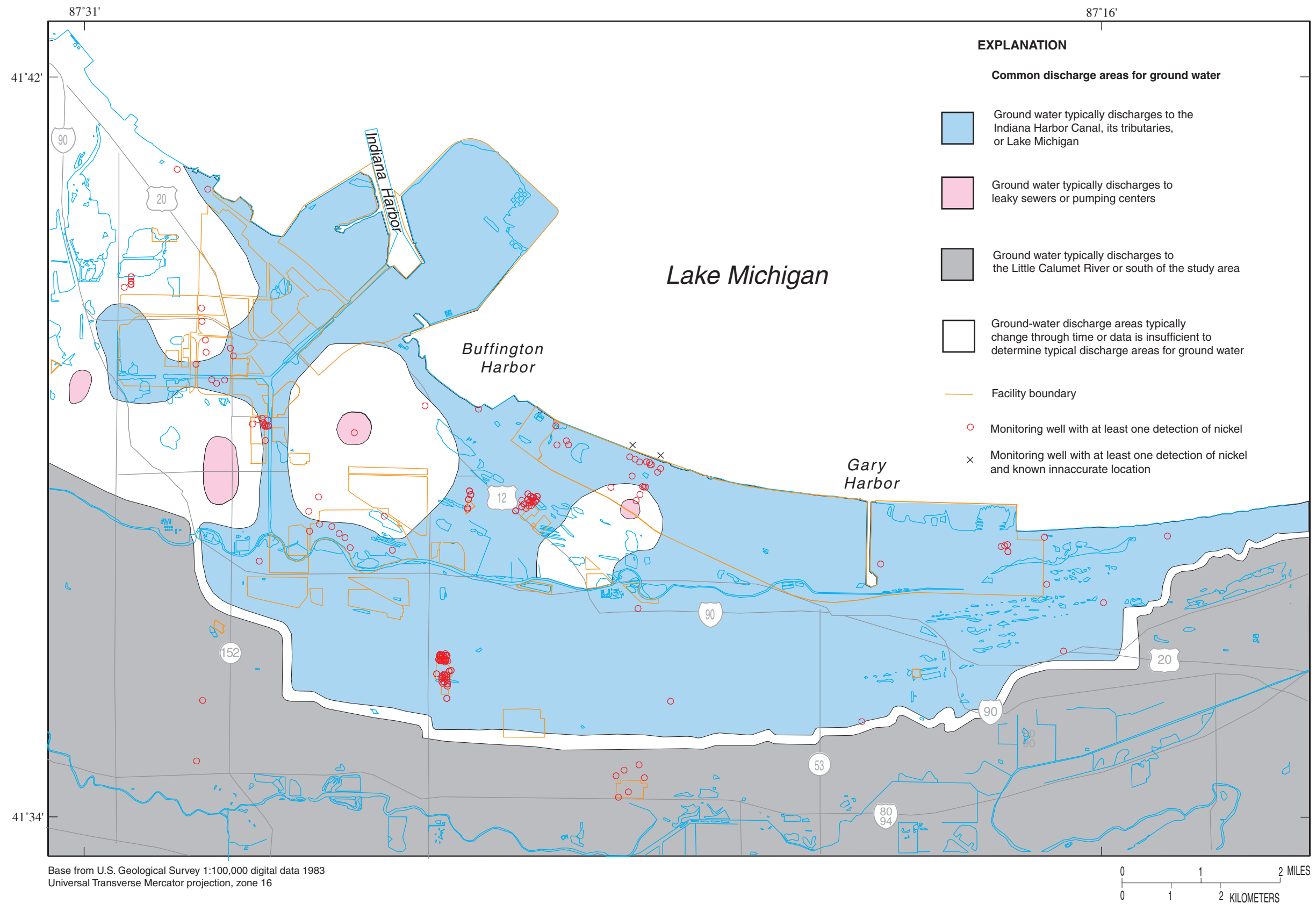
Figure 20. Common discharge areas for ground water in the Calumet aquifer and monitoring wells with at least one detection of nickel in the study area, northwestern Indiana.
