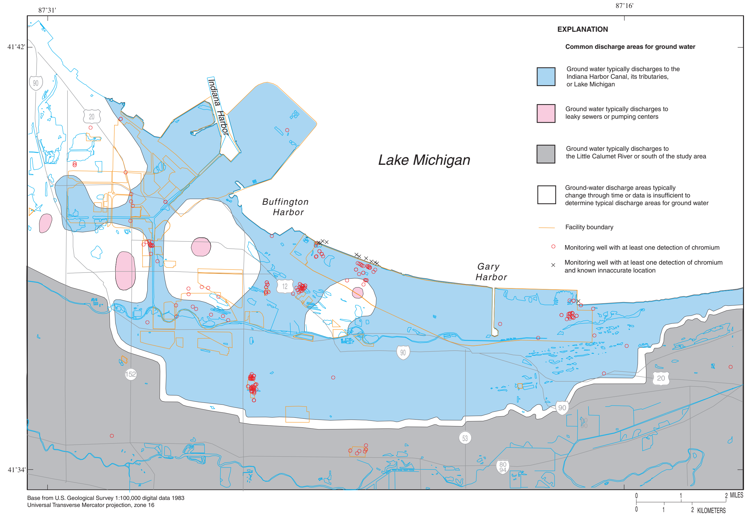
Figure 19. Common discharge areas for ground water in the Calumet aquifer and monitoring wells with at least one detection of chromium in the study area, northwestern Indiana.
