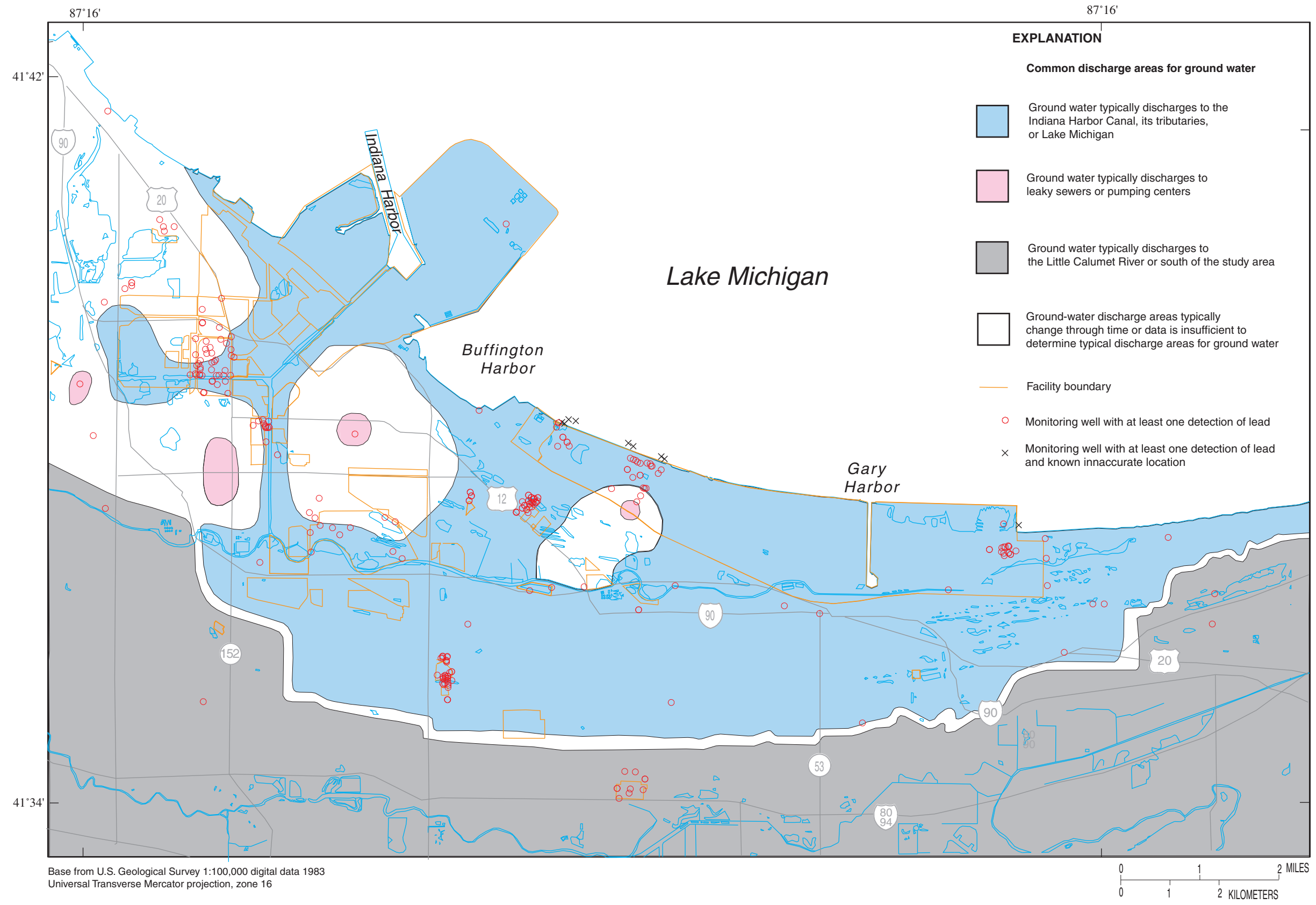
Figure 18. Common discharge areas for ground water in the Calumet aquifer and monitoring wells with at least one detection of lead in the study area, northwestern Indiana.
