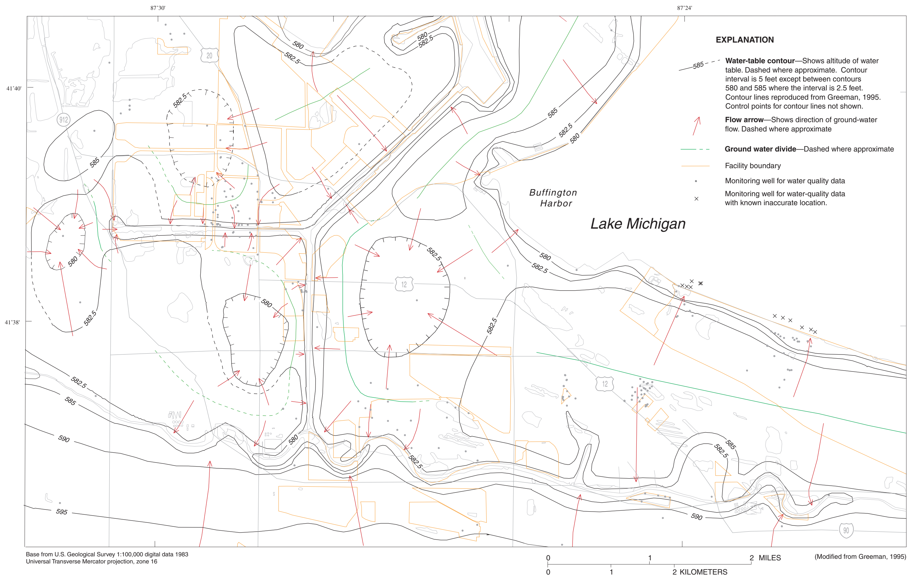
Figure 15. Configuration and altitude of the water table and directions of ground-water flow in the vicinity of the Indiana Harbor Canal, northwestern Indiana, February 26-March 1, 1990 (location for this area shown in Plate 1).
