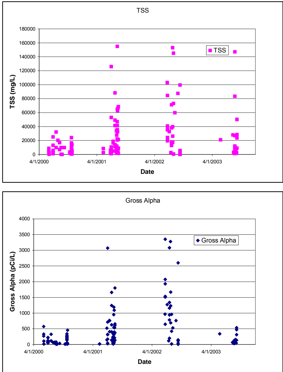
Figure 2.2.3-7. Time trends in TSS and total gross alpha activity in storm runoff on the Pajarito Plateau, 2000–2003.
