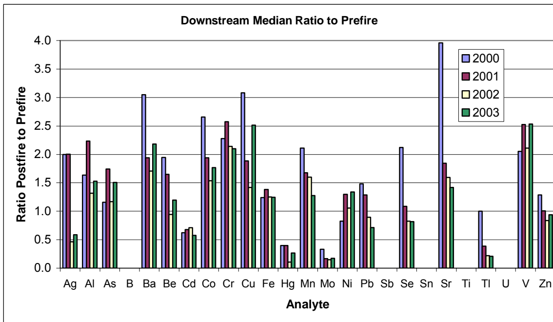
Figure 5.1-7. Ratio of median postfire concentration to median prefire concentration for minor constituents.
