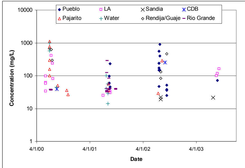
Figure 2.2.2-12. Time series of calcium concentrations in unfiltered runoff, 2000–2003.
