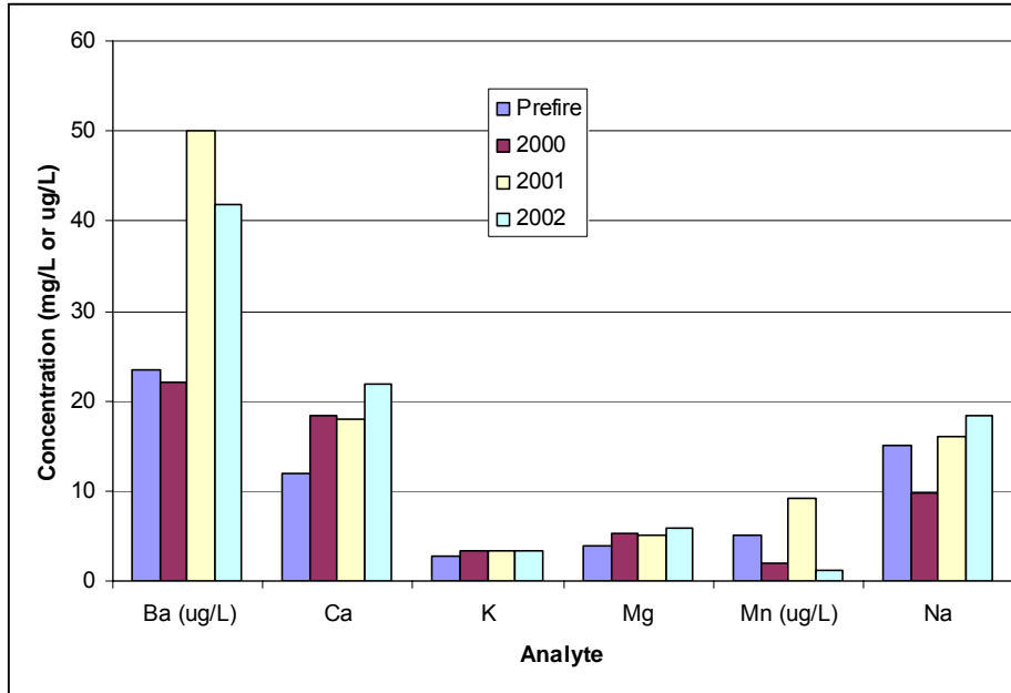
Figure 4-2. Median annual dissolved concentrations of constituents in alluvial groundwater.
