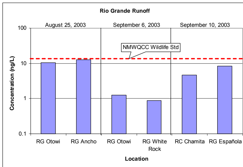
Figure 2.2.5-3. Total PCB concentration in runoff in the Rio Grande, 2003.
