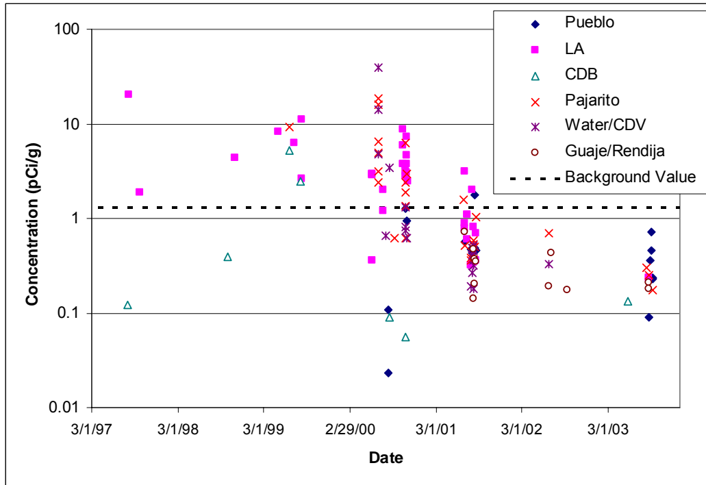
Figure 2.2.3-33. Time series of calculated concentrations of strontium-90 in suspended sediment in storm runoff.
