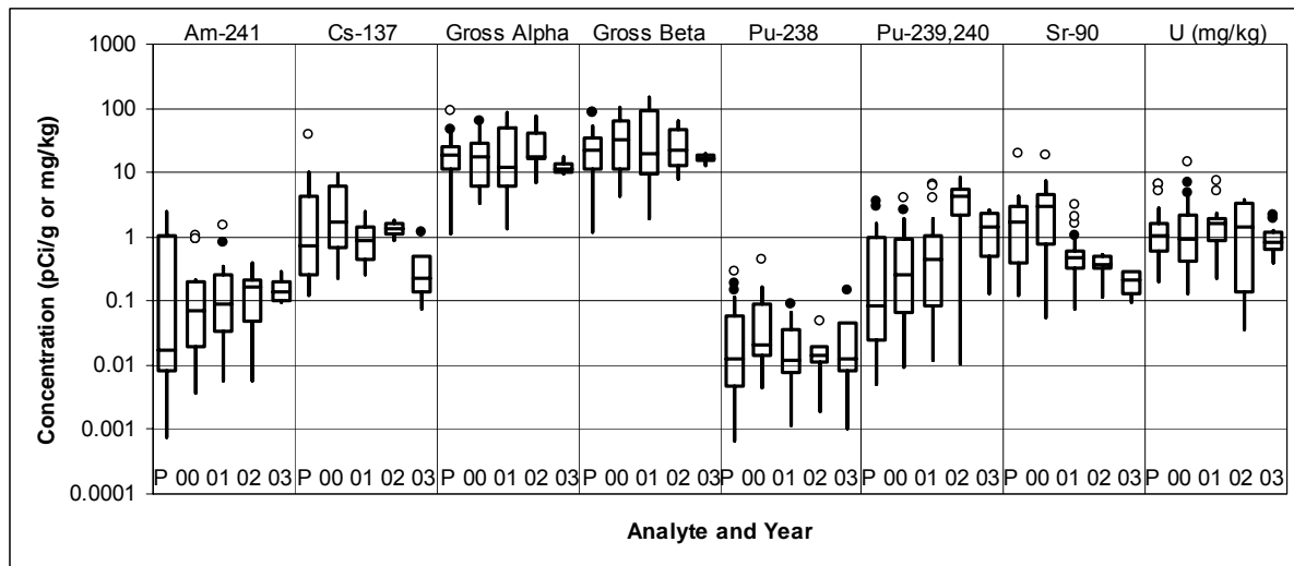
Figure 2.2.3-26. Calculated radionuclide concentrations in suspended sediment at downstream locations, prefire and 2000–2003.
