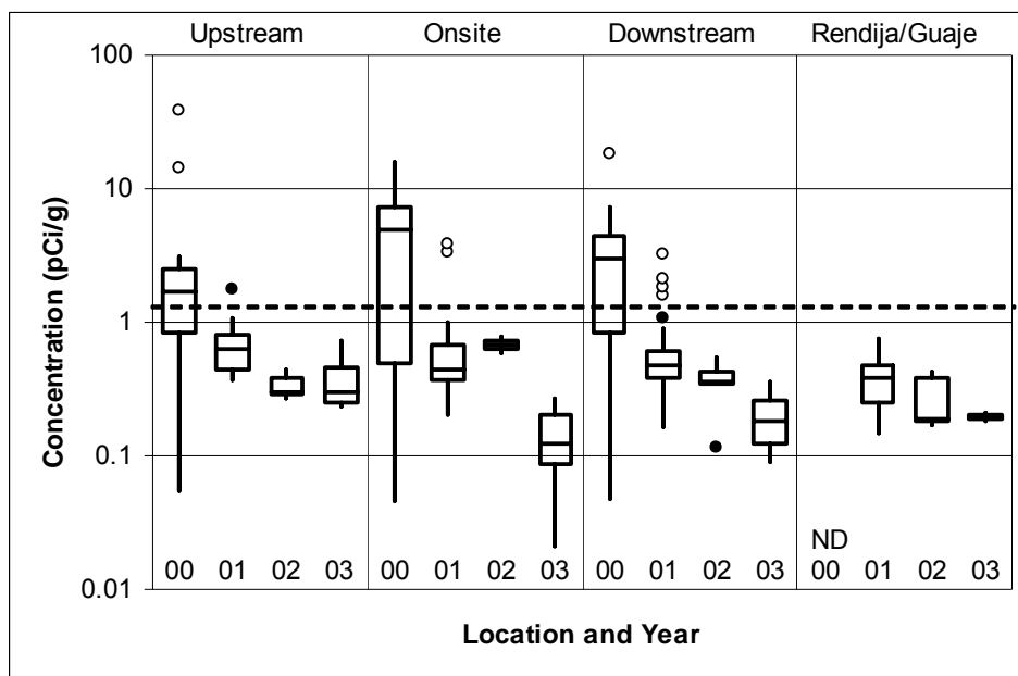
Figure 2.2.3-32. Calculated concentrations of strontium-90 in suspended sediment, 2000–2003.
