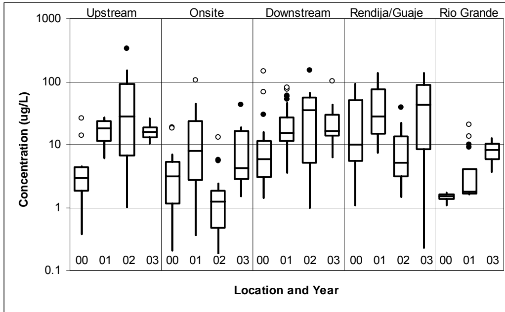
Figure 2.2.3-22. Distribution of uranium concentrations in unfiltered runoff from upstream, onsite, downstream, and Guaje Canyon and unfiltered baseflow from the Rio Grande, 2000–2003.
