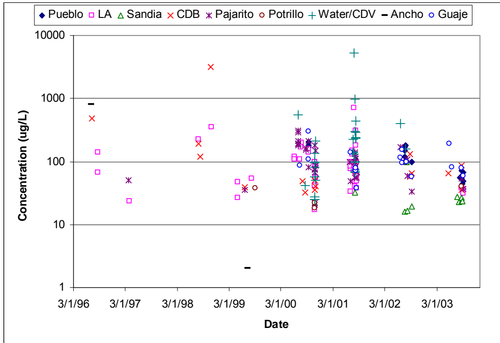
Figure 2.2.4-9. Time series of dissolved barium in runoff from major canyons, 1996–2003.
