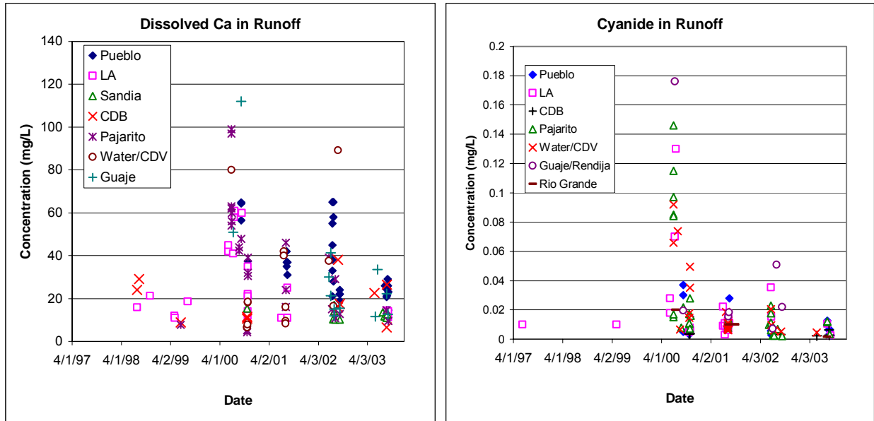
Figure 6.1-2. Time series of dissolved calcium and total cyanide concentrations in runoff, 1997–2003.
