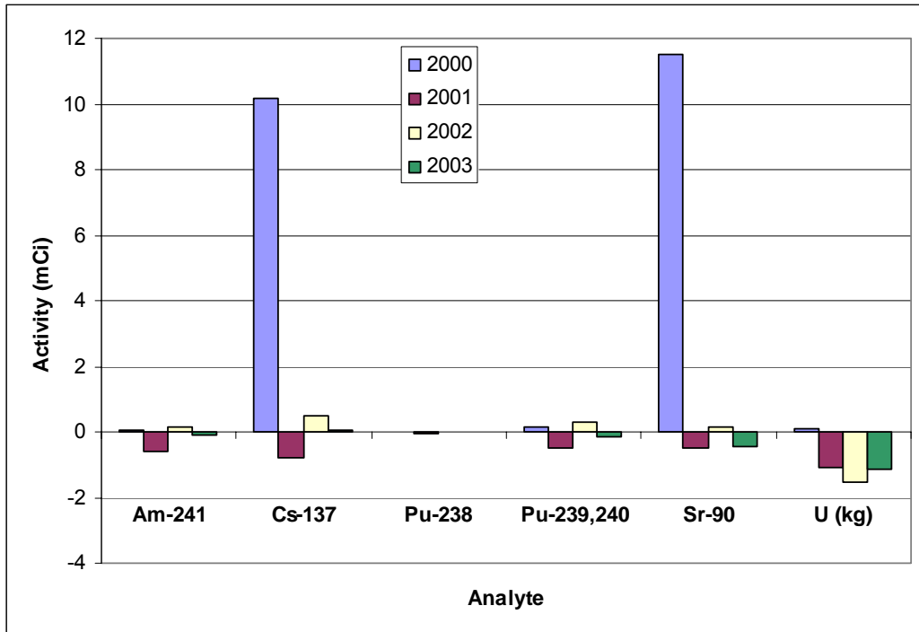
Figure 2.2.3-40. Calculated difference in activity of radionuclides in runoff at upstream and downstream LANL locations (upstream minus downstream; excludes Pueblo Canyon).
