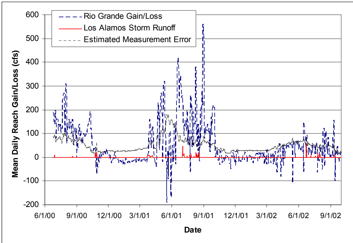
Figure 2.1-8. Stream flow gain/loss in the Rio Grande between USGS gaging stations at Otowi Bridge and near White Rock and runoff from Los Alamos canyons.
