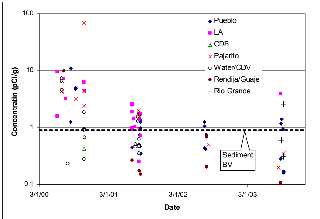
Figure 2.2.3-28. Time series of cesium-137 concentrations in suspended sediment.
