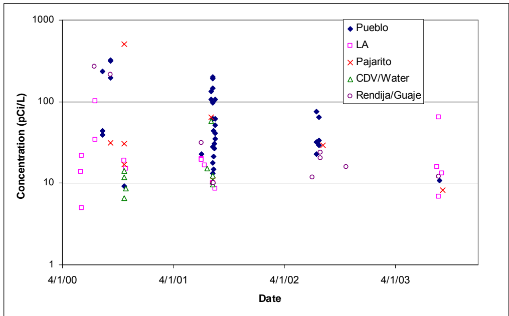
Figure 2.2.3-12. Time series of total cesium-137 detections in runoff from each canyon, 2000-2003.
