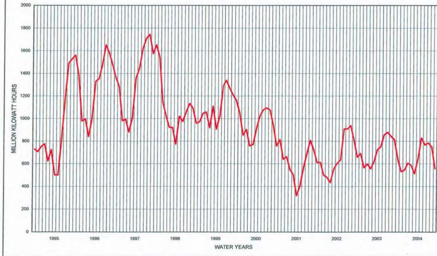
FIGURE CEG6 MONTHLY GENERATION - USBR & COE PLANTS
